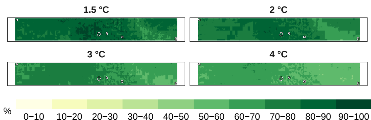
Figure ES1: Percent overall biodiversity remaining at 1 km resolution.
