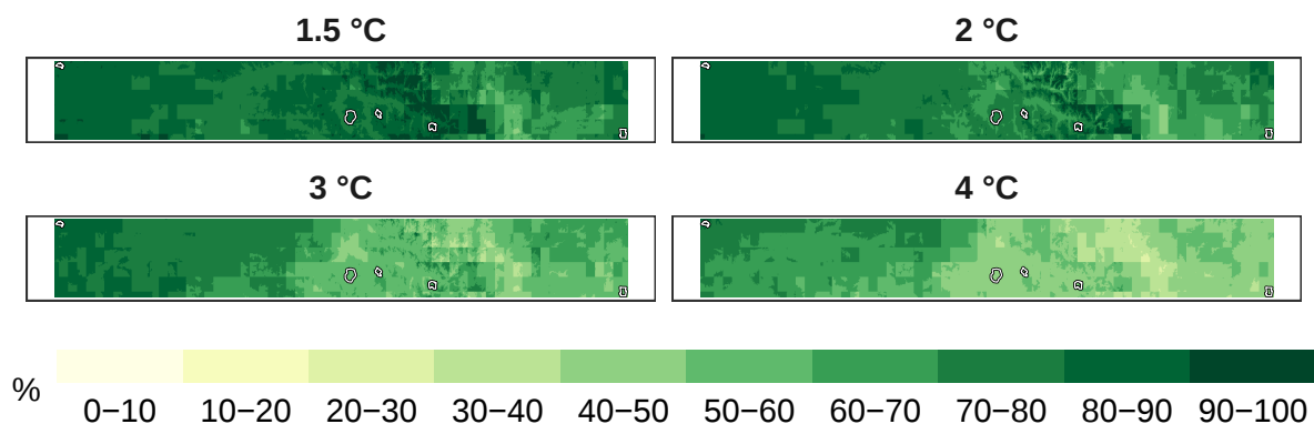
Figure 3: Percent birds remaining at 1 km resolution.
