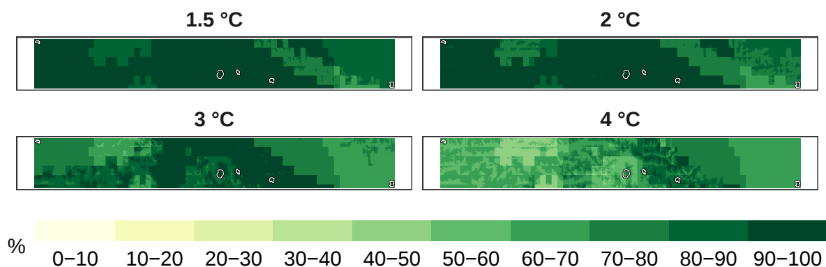
Figure 4: Percent mammals remaining at 1 km resolution.
