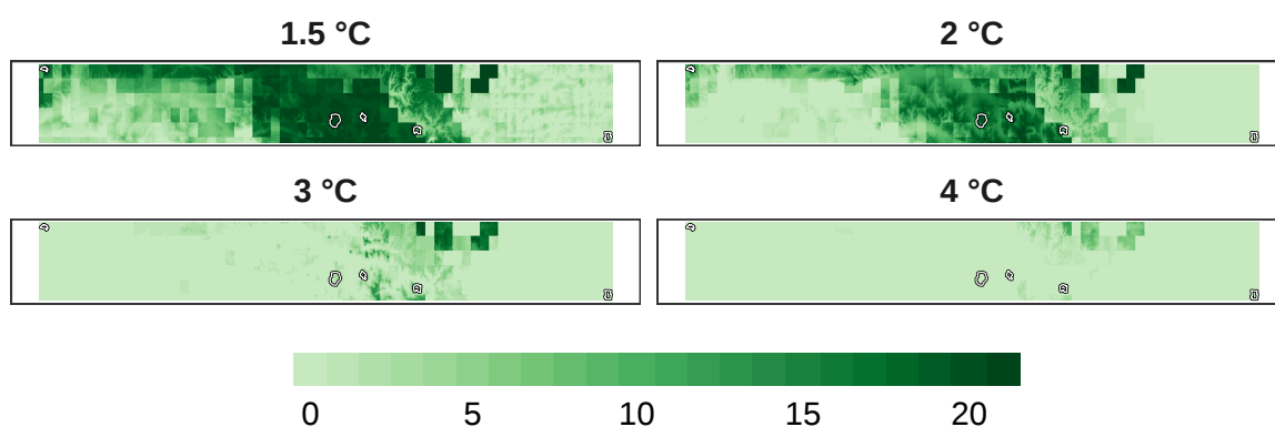
Figure 8: Number of models in agreement for plant refugia at 1 km resolution.
