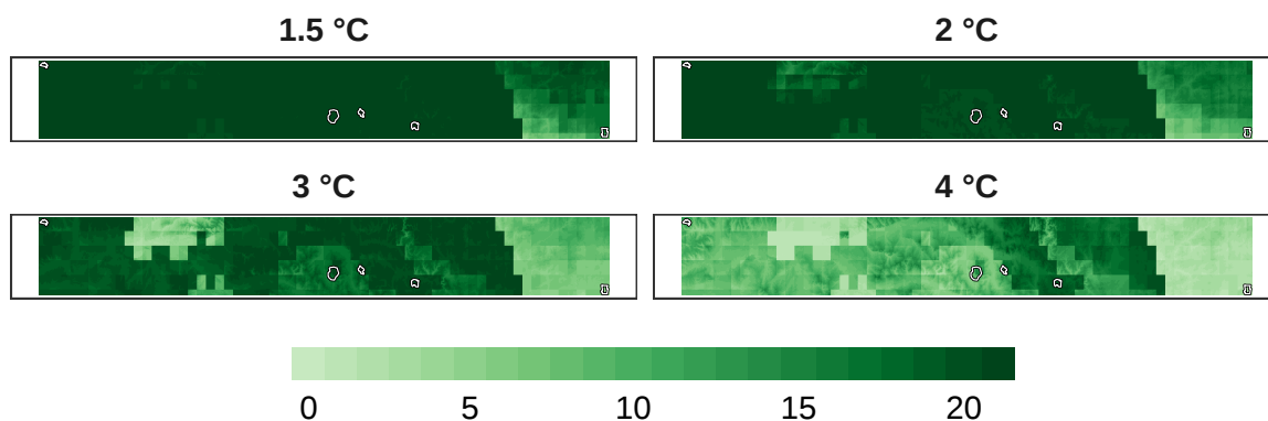
Figure 10: Number of models in agreement for mammal refugia at 1 km resolution.
