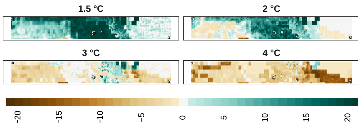
Figure 14: Adaptation effort for plants at 1 km resolution.
