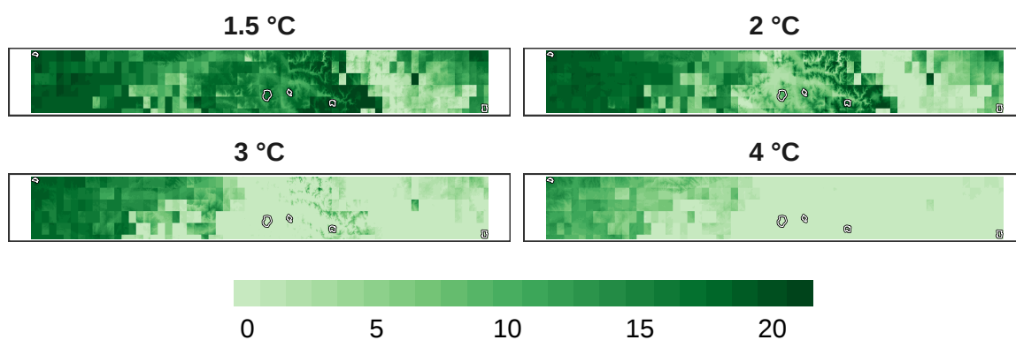
Figure 9: Number of models in agreement for bird refugia.
