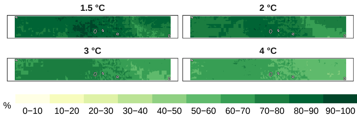
Figure 1: Percent overall biodiversity remaining at 1 km resolution.
