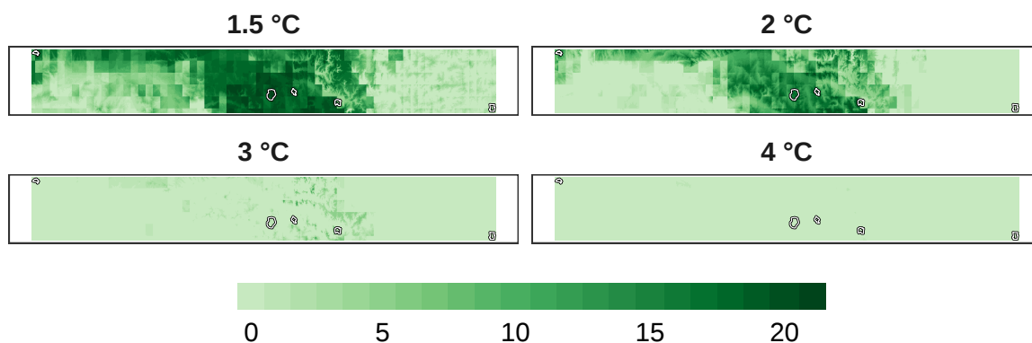
Figure 7: Number of models in agreement for overall biodiversity refugia at 1 km resolution.
