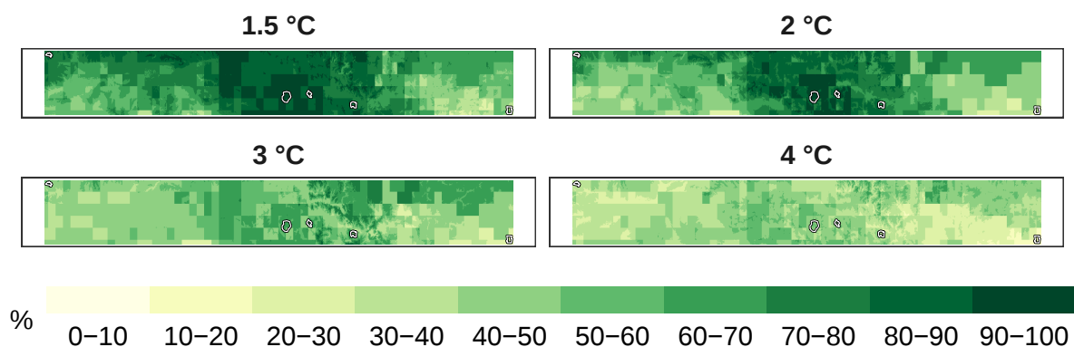
Figure 2: Percent plants remaining at 1 km resolution.
