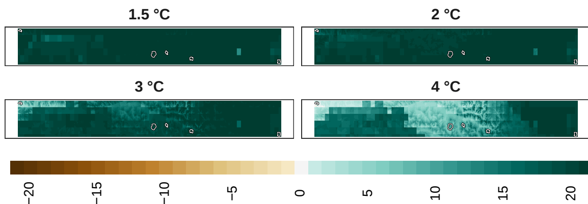
Figure 17: Adaptation effort for reptiles at 1 km resolution.
