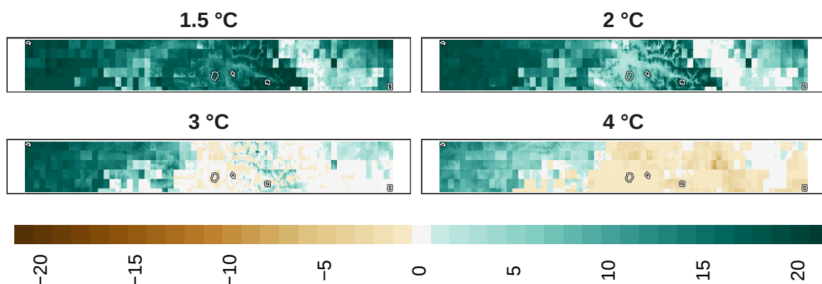
Figure 15: Adaptation effort for birds at 1 km resolution.
