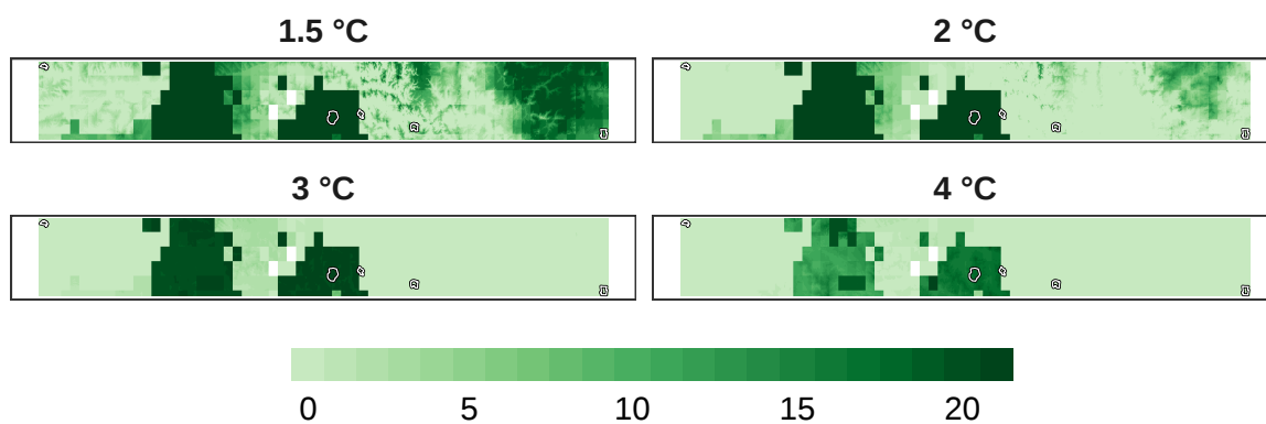
Figure 12: Number of models in agreement for insect refugia at 1 km resolution.
