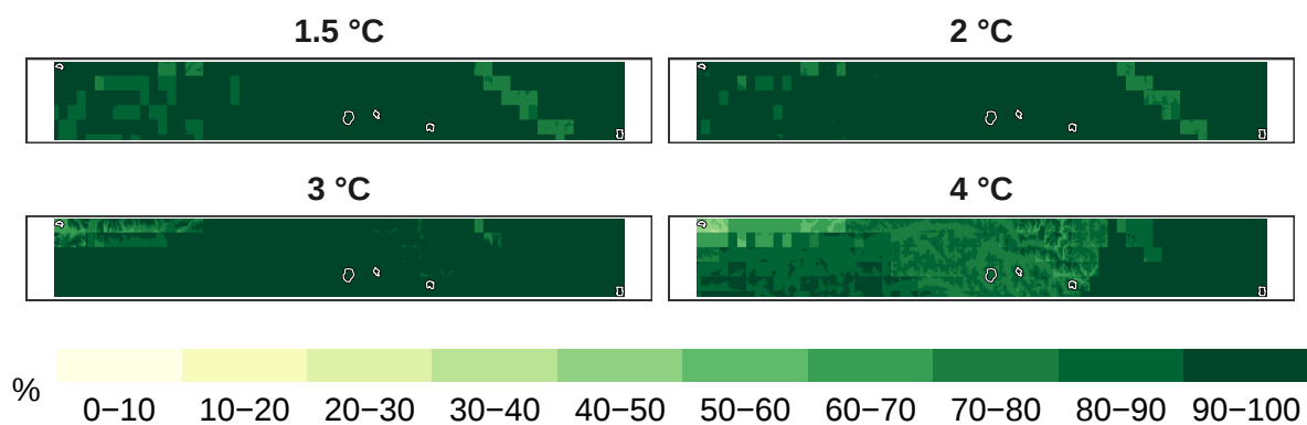
Figure 5: Percent reptiles remaining at 1 km resolution.
