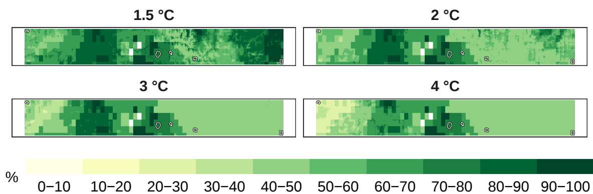
Figure 6: Percent insects remaining at 1 km resolution.
