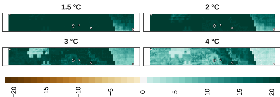
Figure 16: Adaptation effort for mammals at 1 km resolution.
