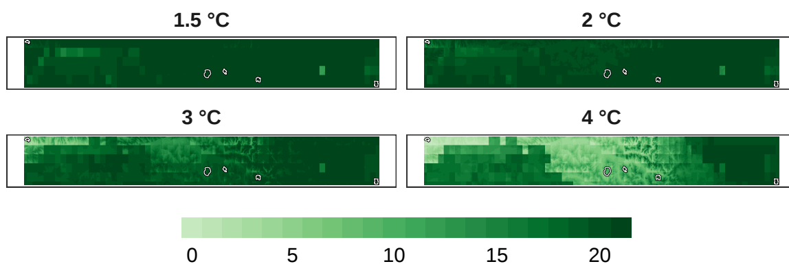
Figure 11: Number of models in agreement for reptile refugia at 1 km resolution.
