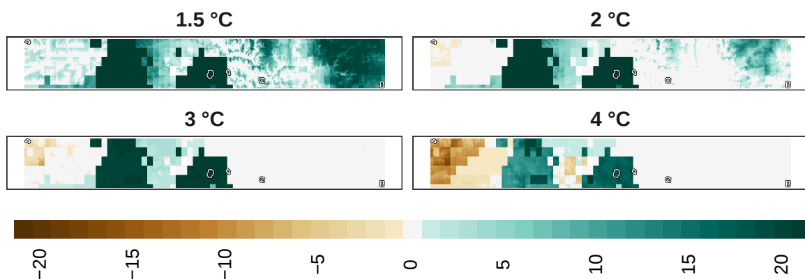
Figure 18: Adaptation effort for insects at 1 km resolution.
