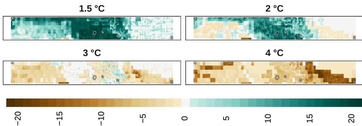
Figure 13: Adaptation effort for overall biodiversity at 1 km resolution.
