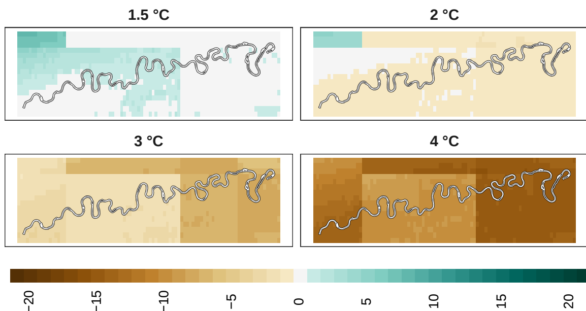
Figure 11: Adaptation effort for overall biodiversity at 1 km resolution.
