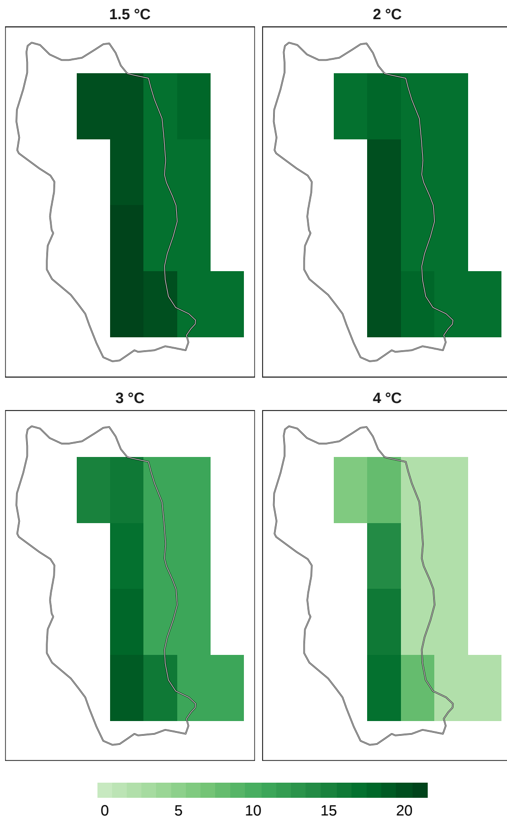
Figure 8: Number of models in agreement for overall biodiversity refugia at 1 km resolution.
