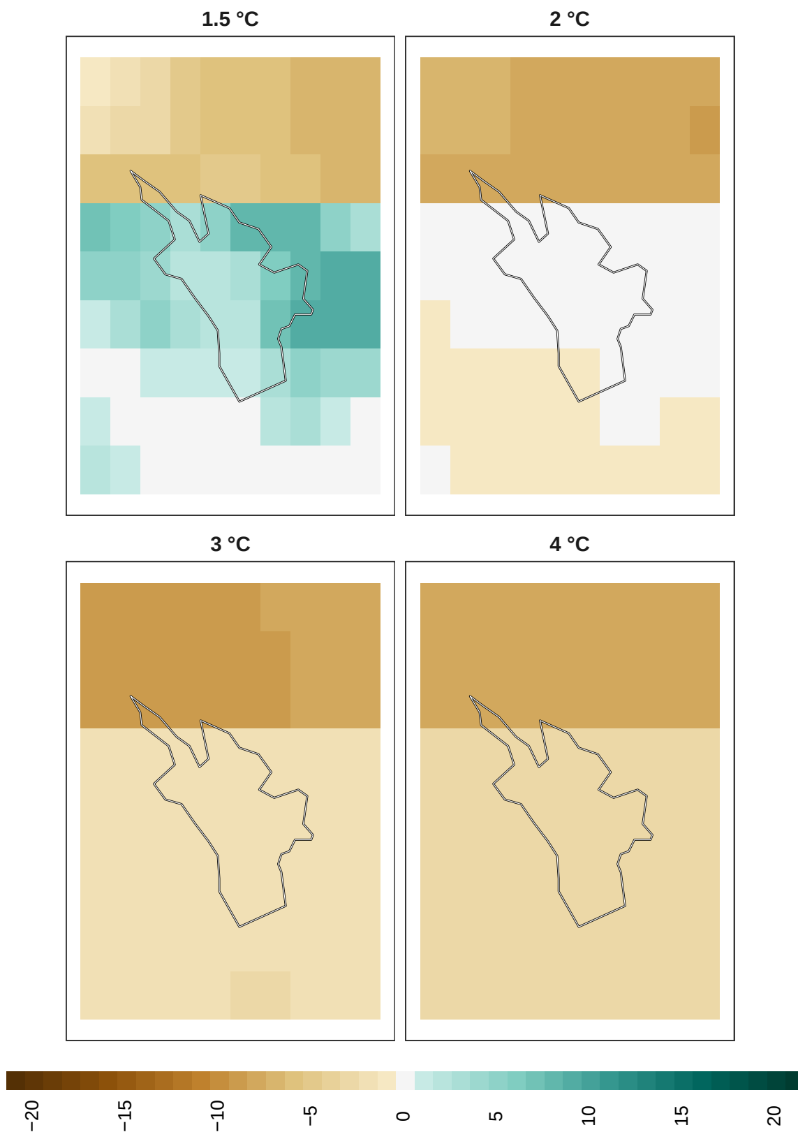
Figure 18: Adaptation effort for reptiles at 1 km resolution.
