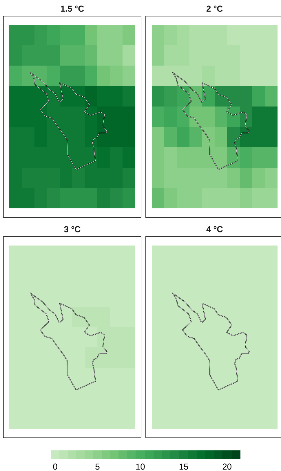
Figure 13: Number of models in agreement for insect refugia at 1 km resolution.
