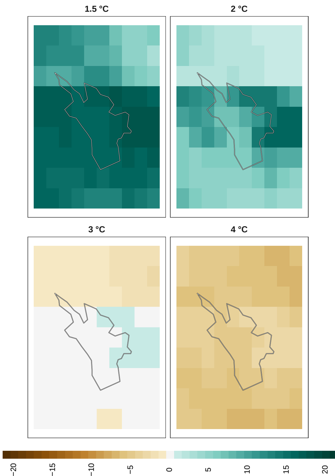
Figure 19: Adaptation effort for insects at 1 km resolution.
