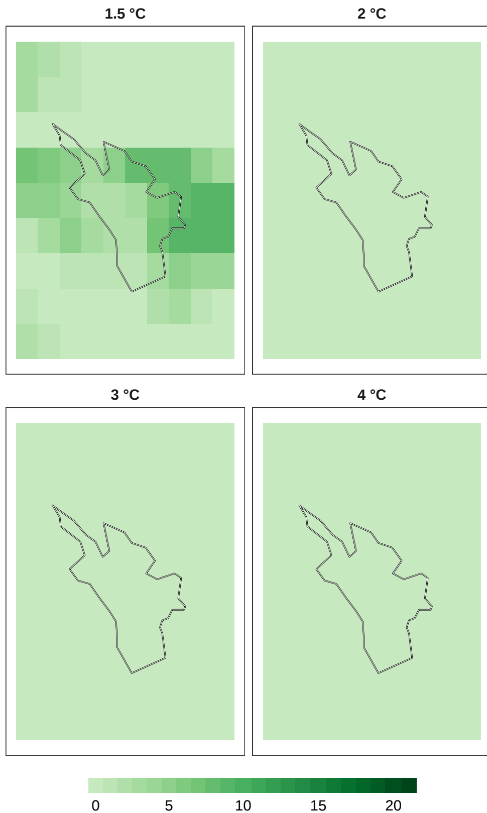
Figure 12: Number of models in agreement for reptile refugia at 1 km resolution.
