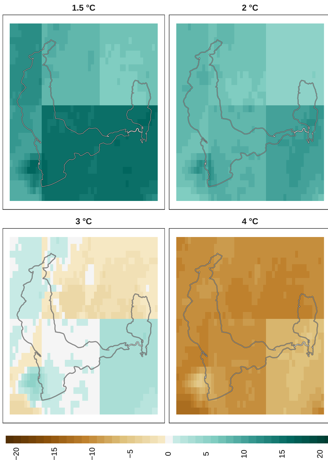
Figure 13: Adaptation effort for mammals at 1 km resolution.
