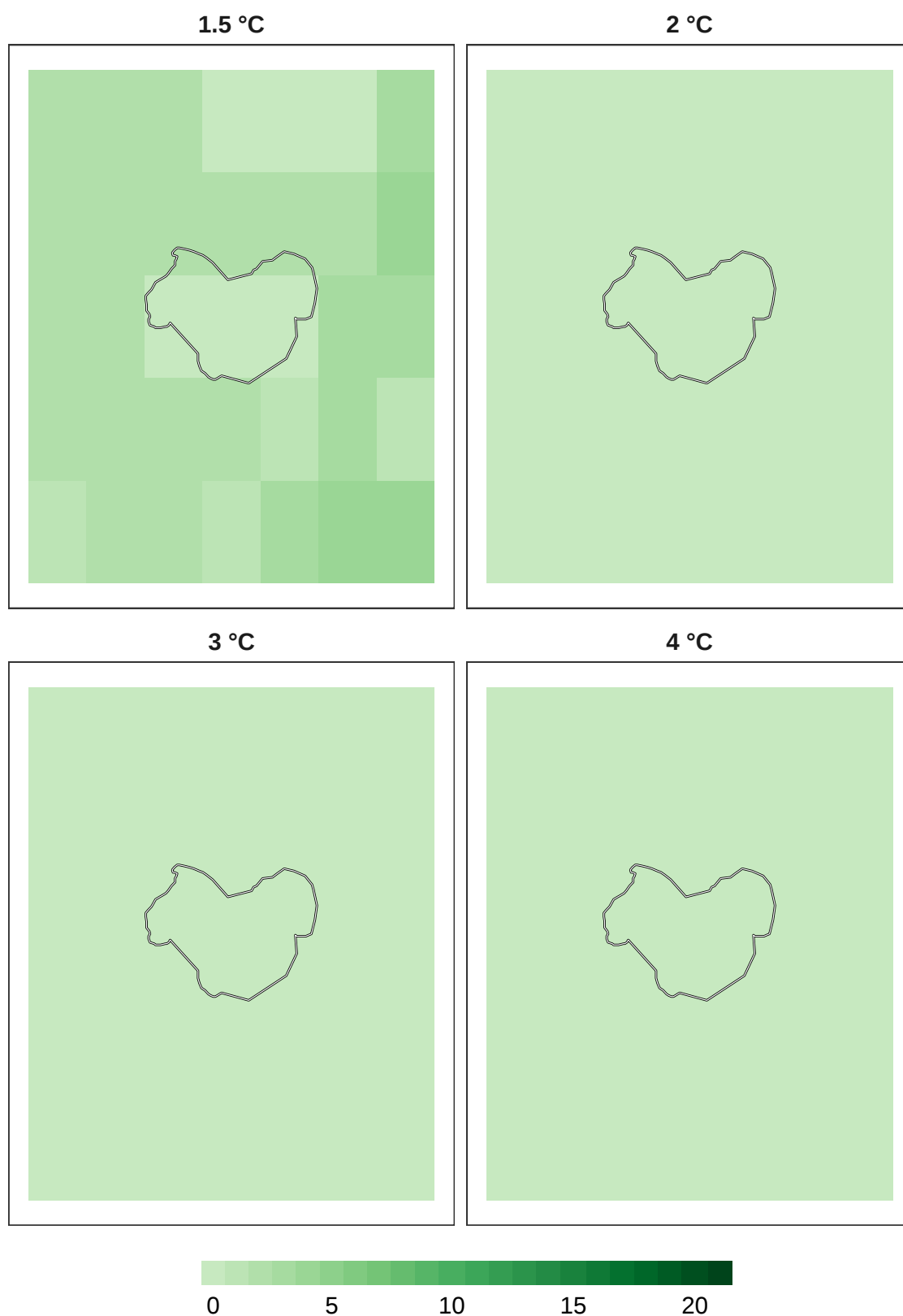
Figure 6: Number of models in agreement for overall biodiversity refugia at 1 km resolution.
