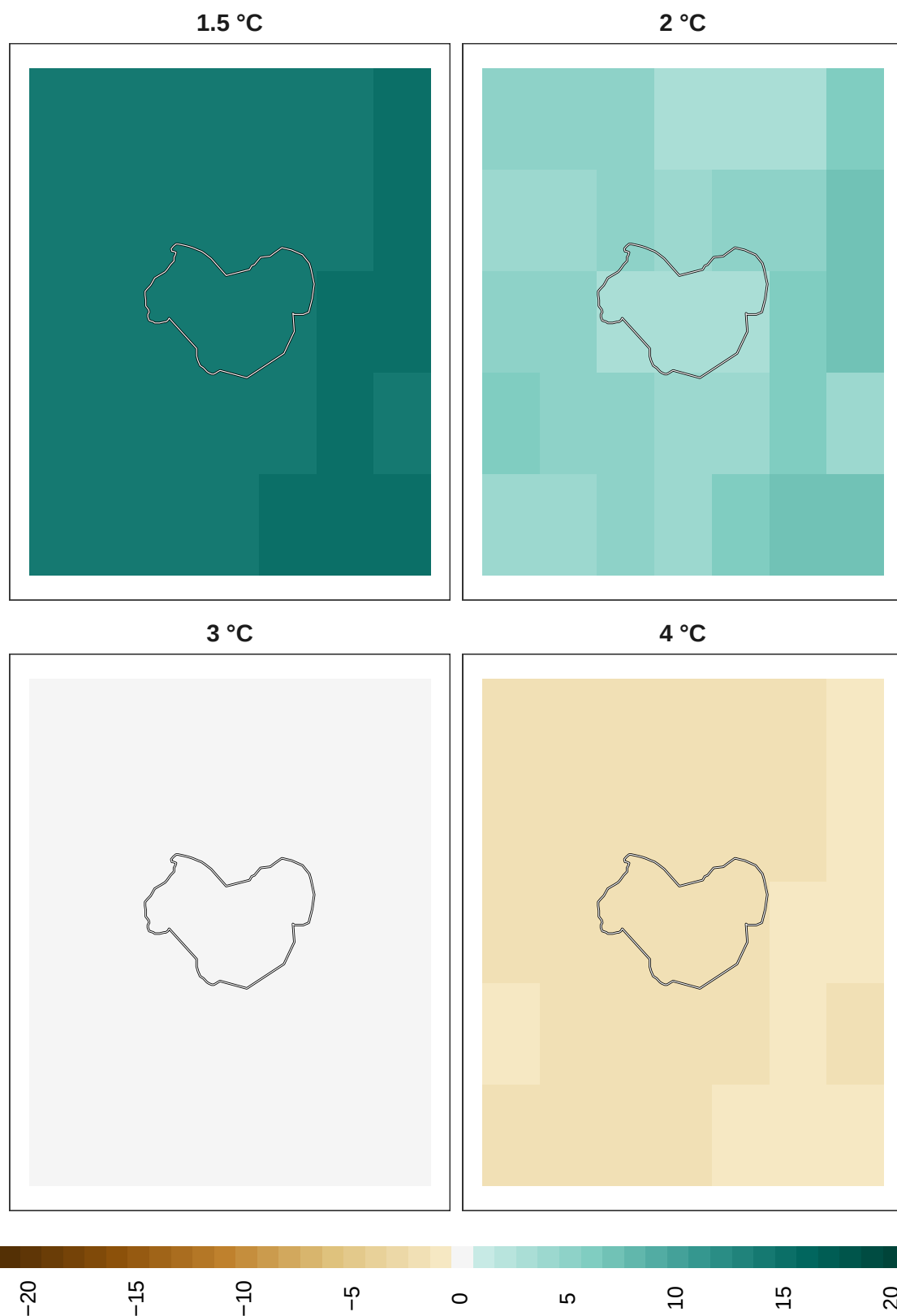
Figure 15: Adaptation effort for insects at 1 km resolution.
