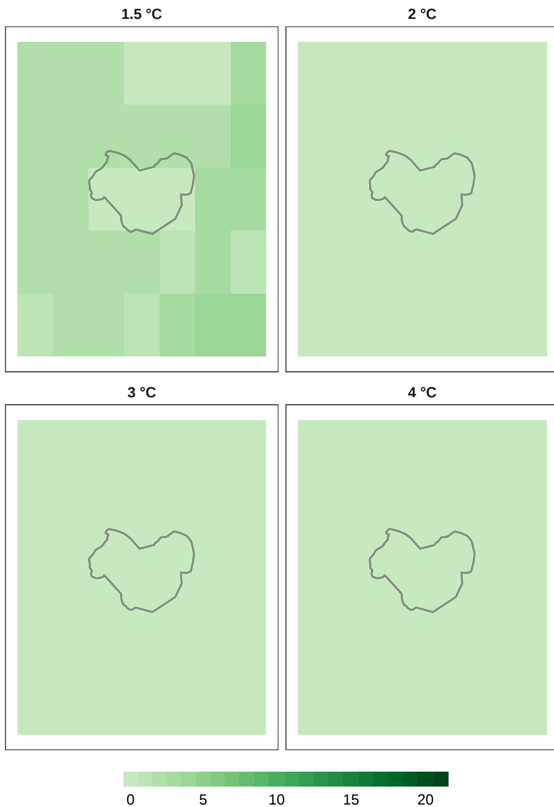
Figure 7: Number of models in agreement for plant refugia at 1 km resolution.
