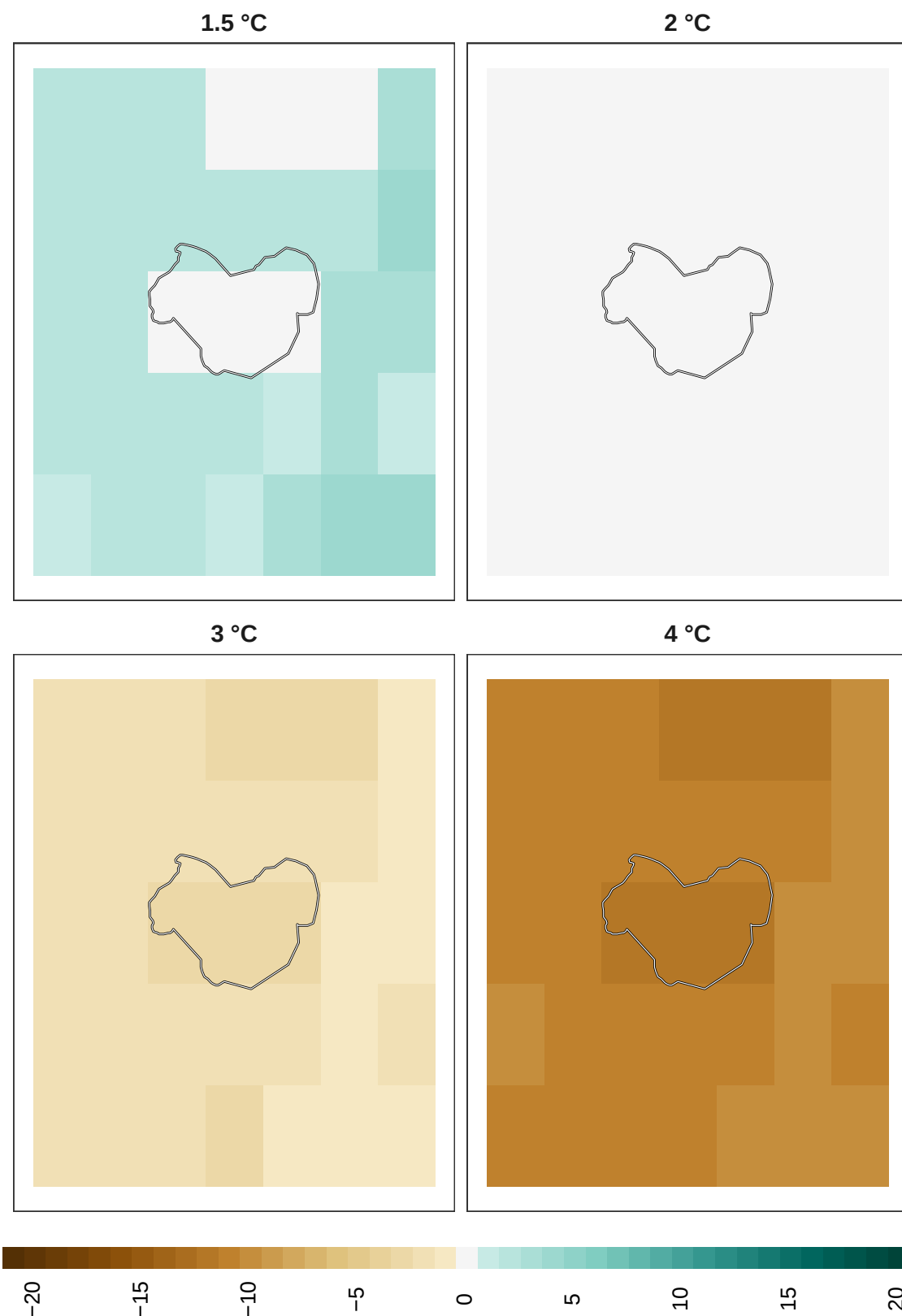
Figure 11: Adaptation effort for overall biodiversity at 1 km resolution.
