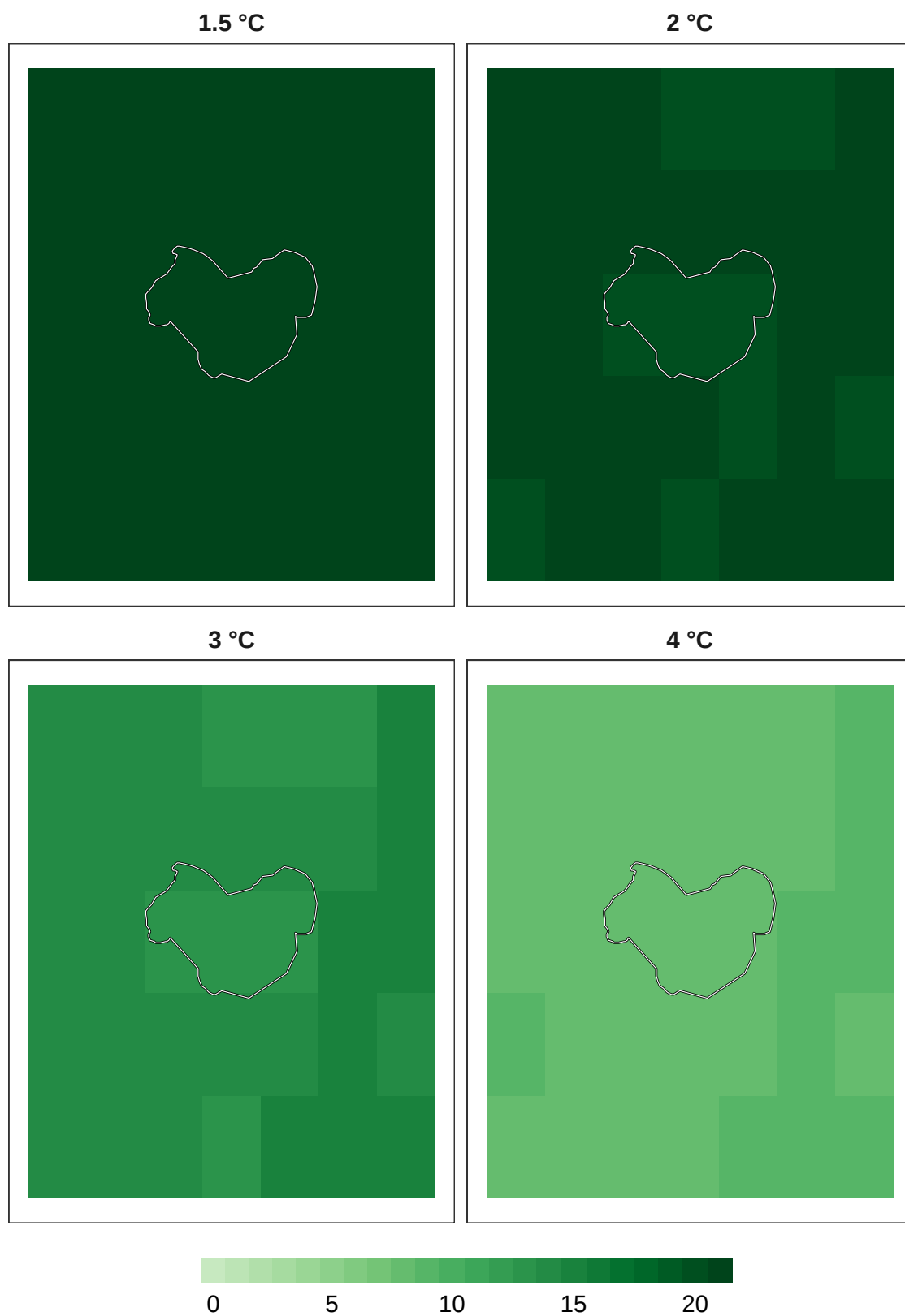
Figure 8: Number of models in agreement for bird refugia.
