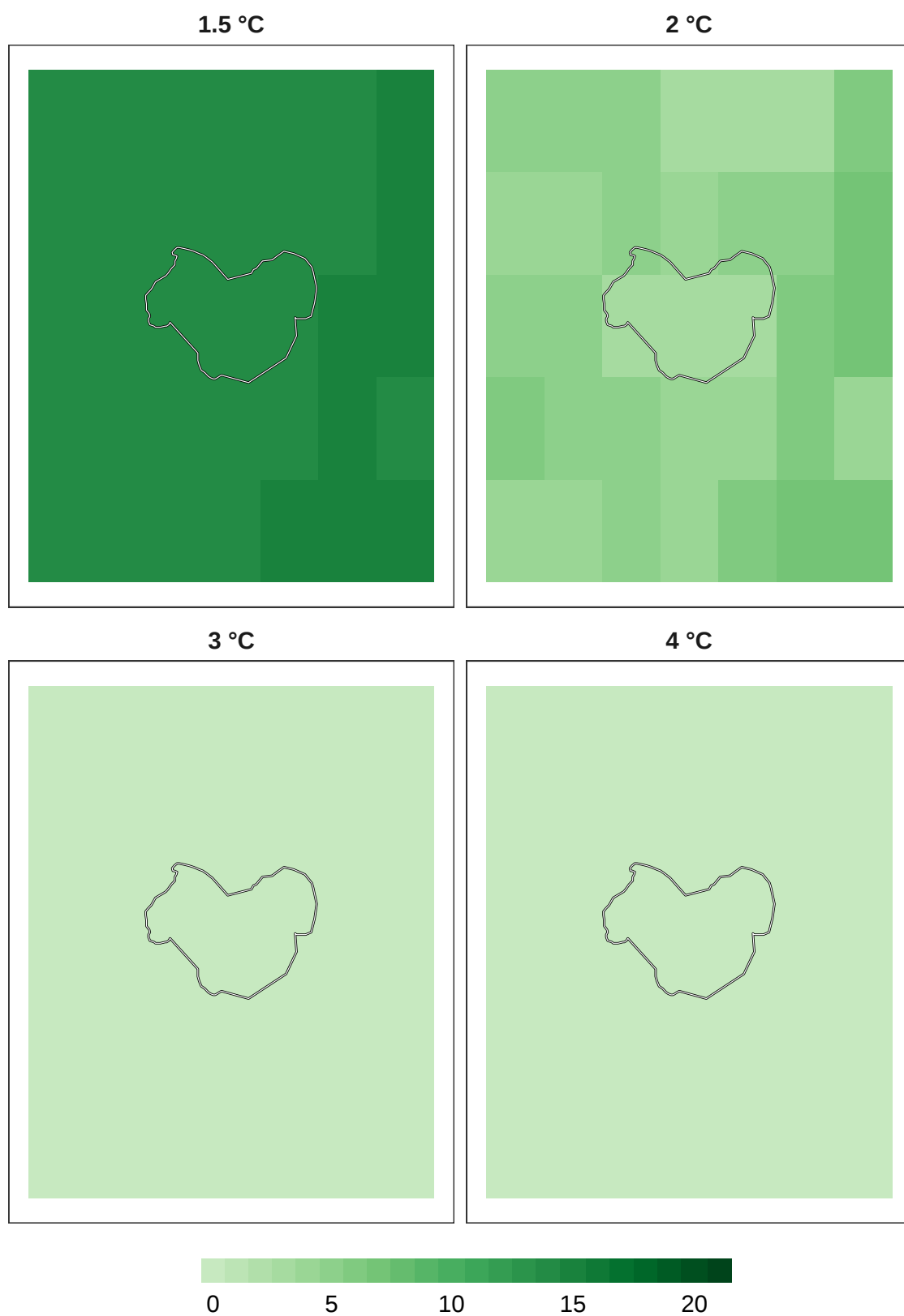
Figure 10: Number of models in agreement for insect refugia at 1 km resolution.
