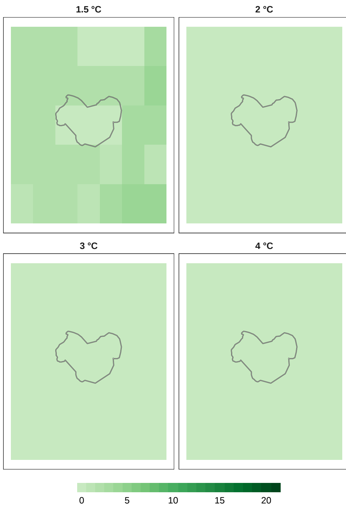
Figure 9: Number of models in agreement for mammal refugia at 1 km resolution.
