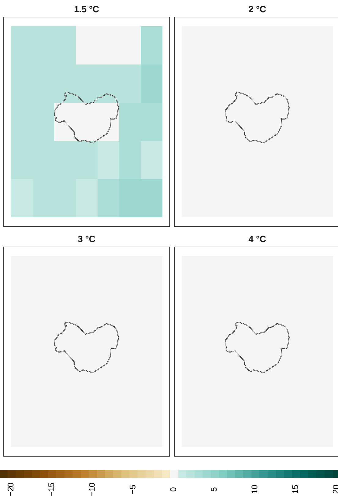
Figure 14: Adaptation effort for mammals at 1 km resolution.
