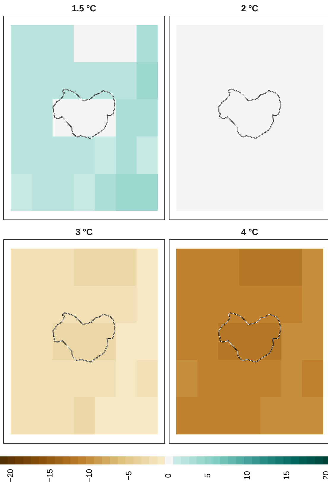
Figure 12: Adaptation effort for plants at 1 km resolution.
