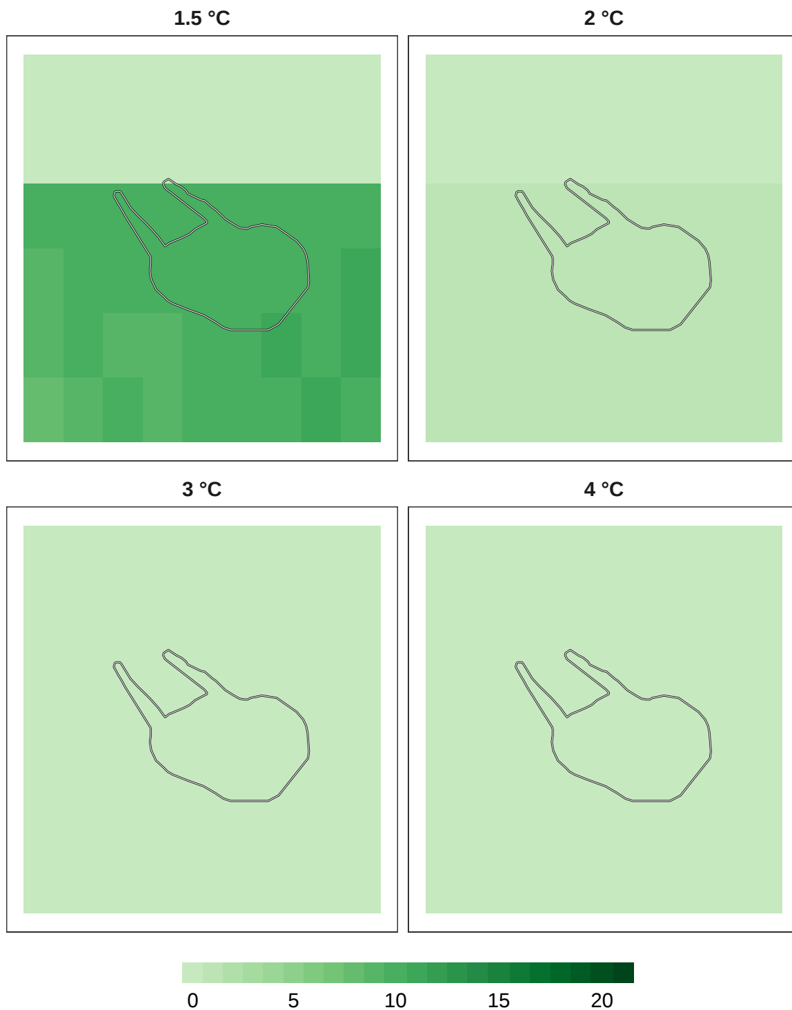
Figure 12: Number of models in agreement for reptile refugia at 1 km resolution.
