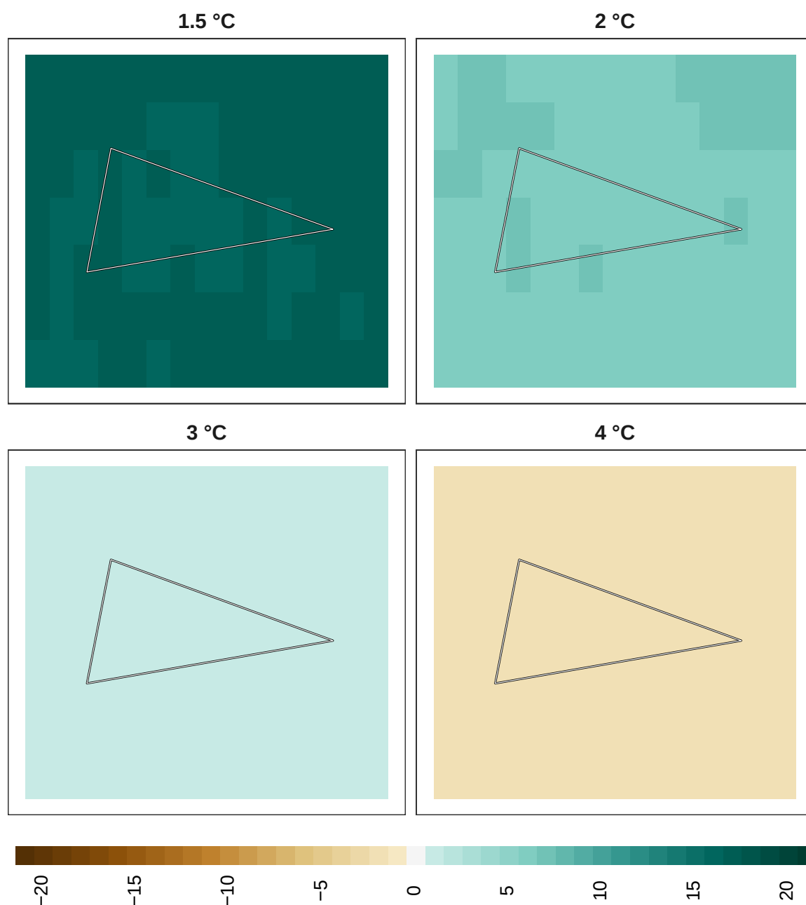
Figure 12: Adaptation effort for mammals at 1 km resolution.
