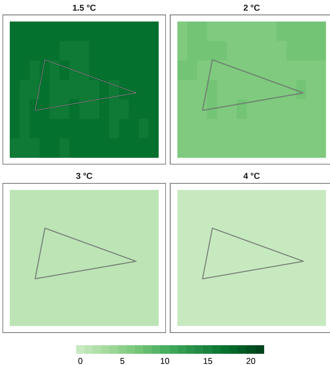
Figure 8: Number of models in agreement for mammal refugia at 1 km resolution.
