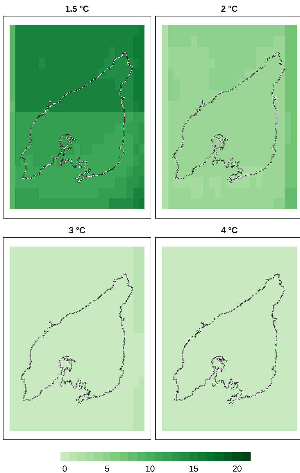
Figure 9: Number of models in agreement for plant refugia at 1 km resolution.
