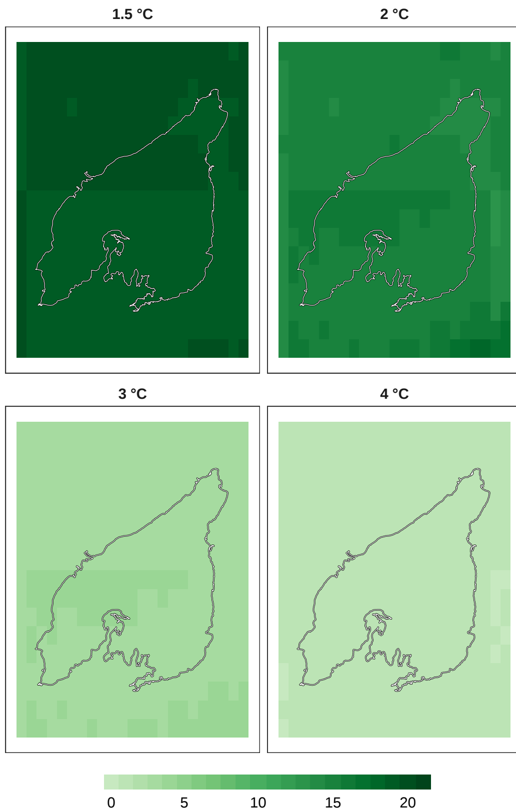
Figure 11: Number of models in agreement for mammal refugia at 1 km resolution.
