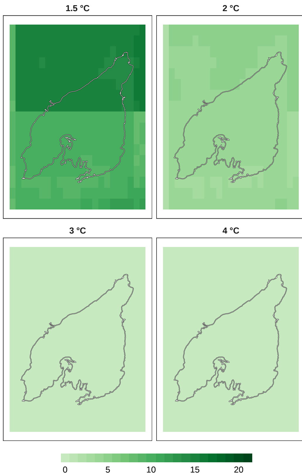
Figure 8: Number of models in agreement for overall biodiversity refugia at 1 km resolution.
