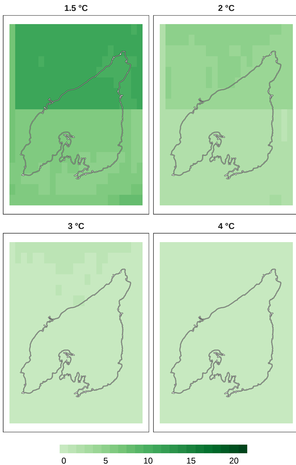
Figure 13: Number of models in agreement for pollinator refugia at 1 km resolution.
