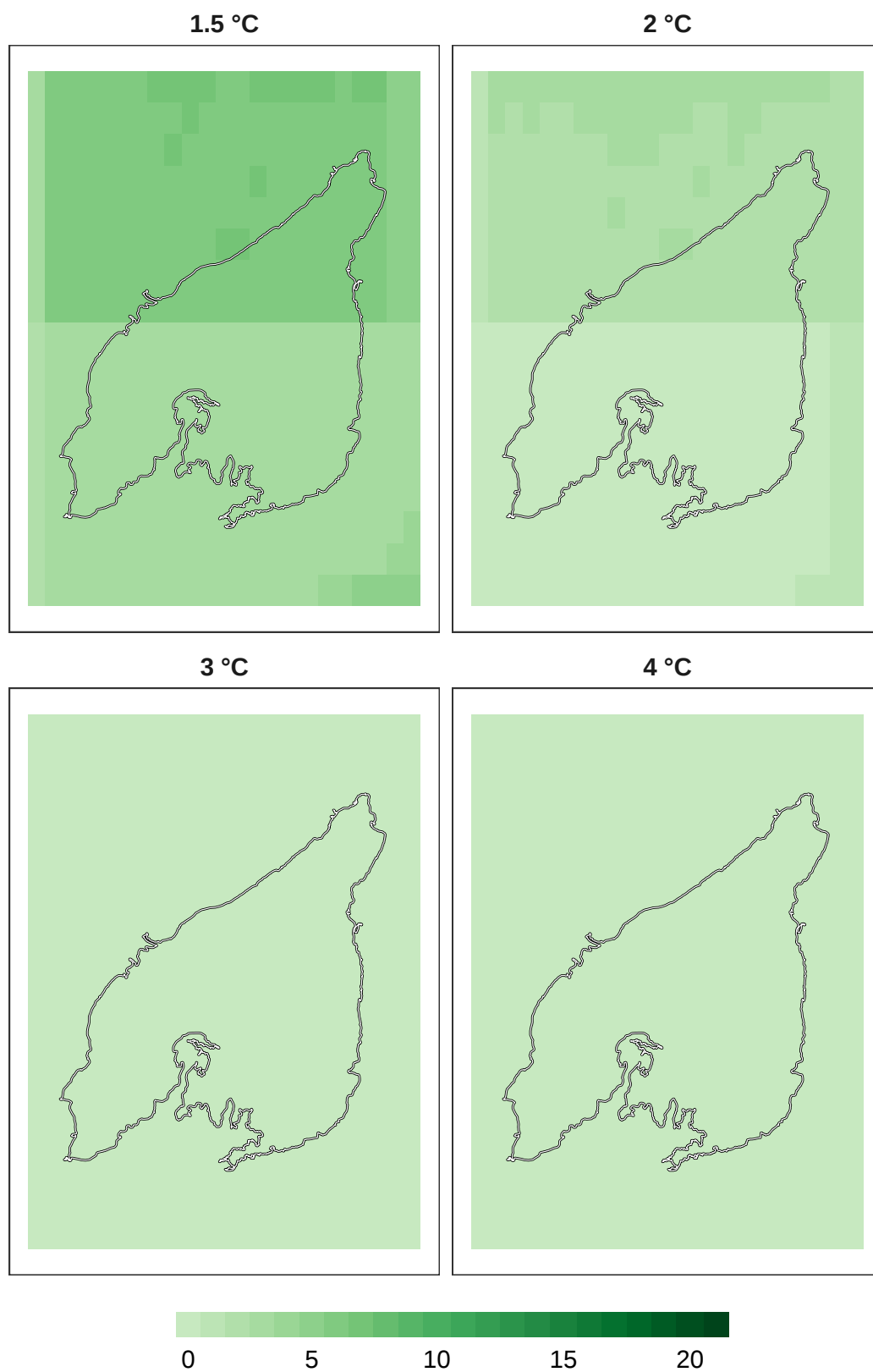
Figure 12: Number of models in agreement for insect refugia at 1 km resolution.
