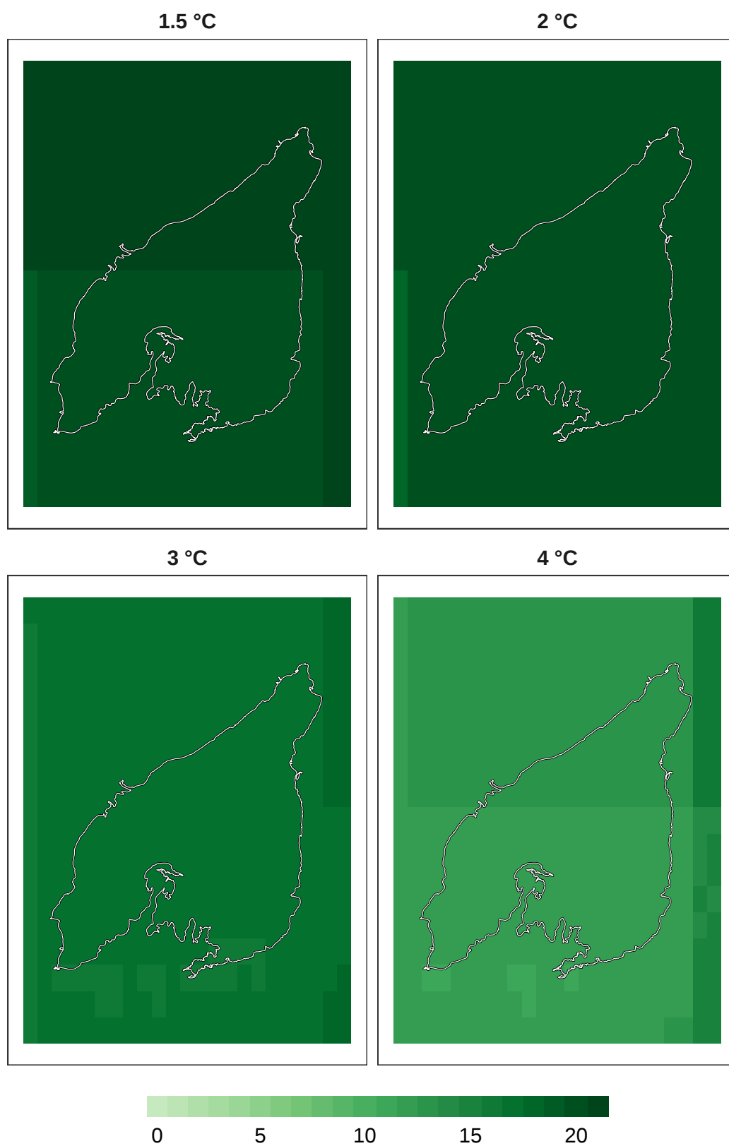
Figure 10: Number of models in agreement for bird refugia.
