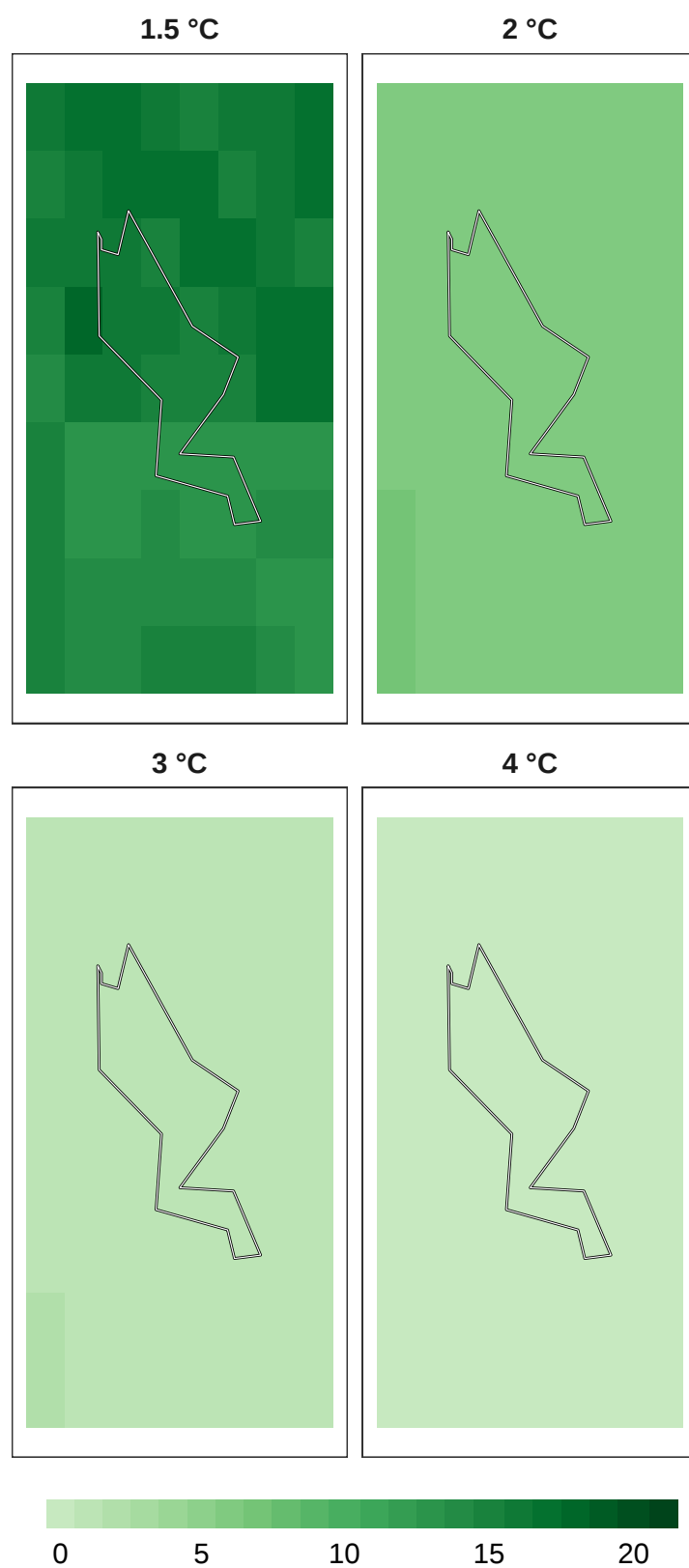
Figure 10: Number of models in agreement for plant refugia at 1 km resolution.
