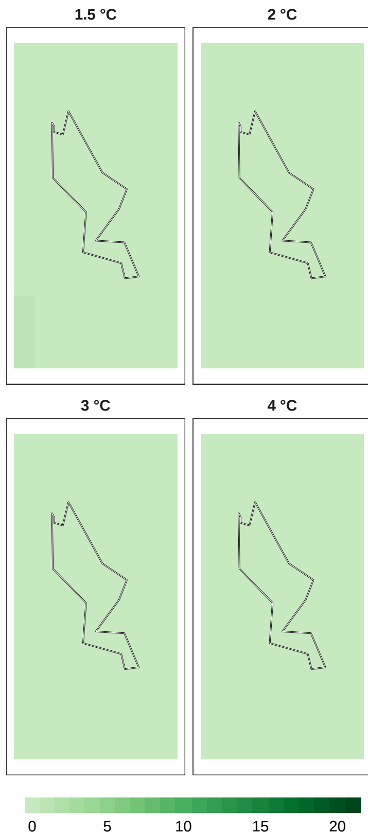
Figure 14: Number of models in agreement for insect refugia at 1 km resolution.
