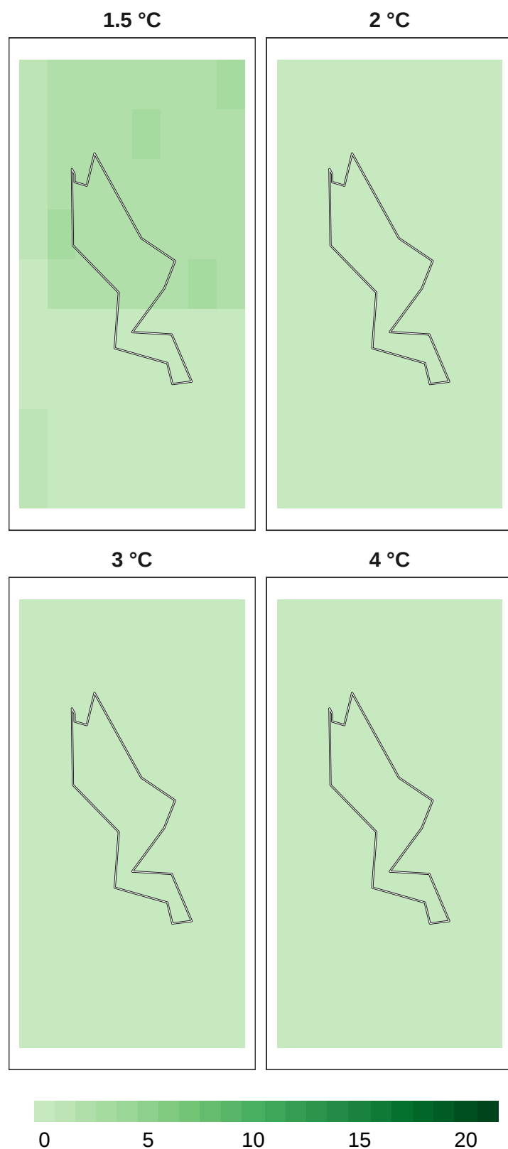
Figure 9: Number of models in agreement for overall biodiversity refugia at 1 km resolution.
