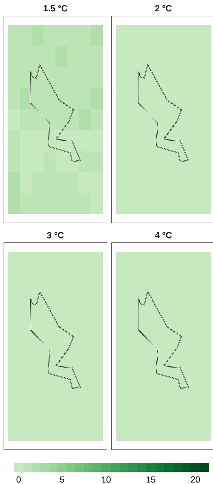
Figure 15: Number of models in agreement for pollinator refugia at 1 km resolution.
