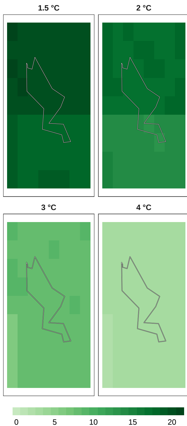
Figure 12: Number of models in agreement for mammal refugia at 1 km resolution.
