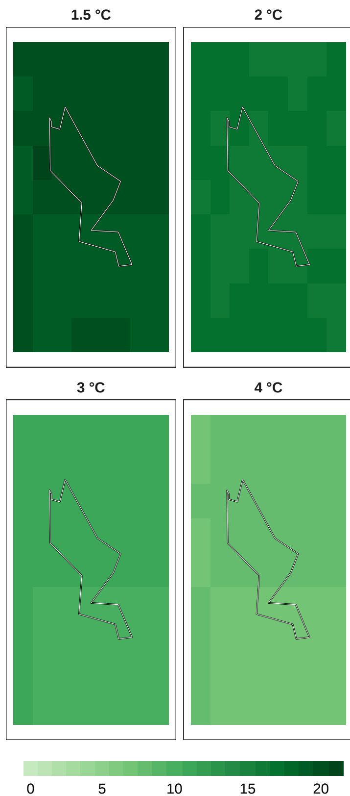
Figure 11: Number of models in agreement for bird refugia.
