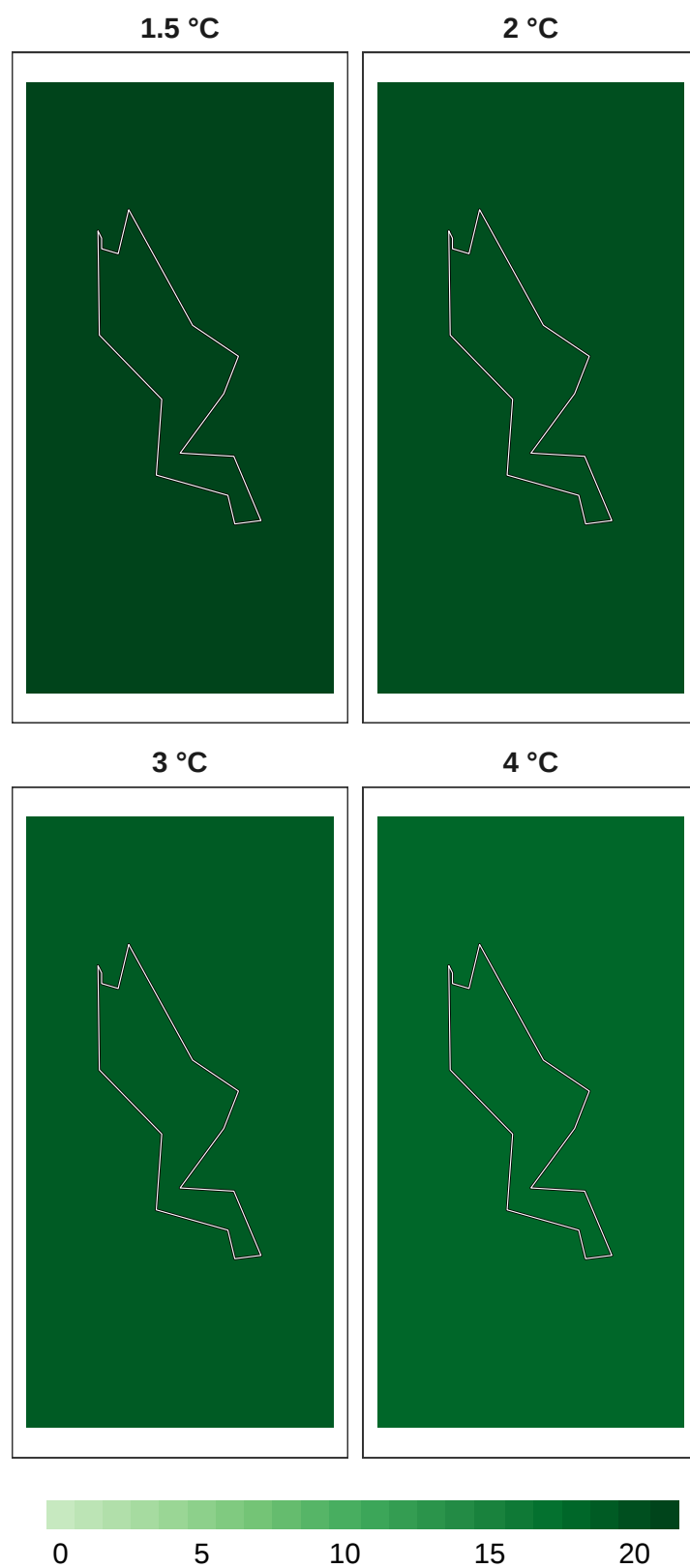
Figure 13: Number of models in agreement for reptile refugia at 1 km resolution.
