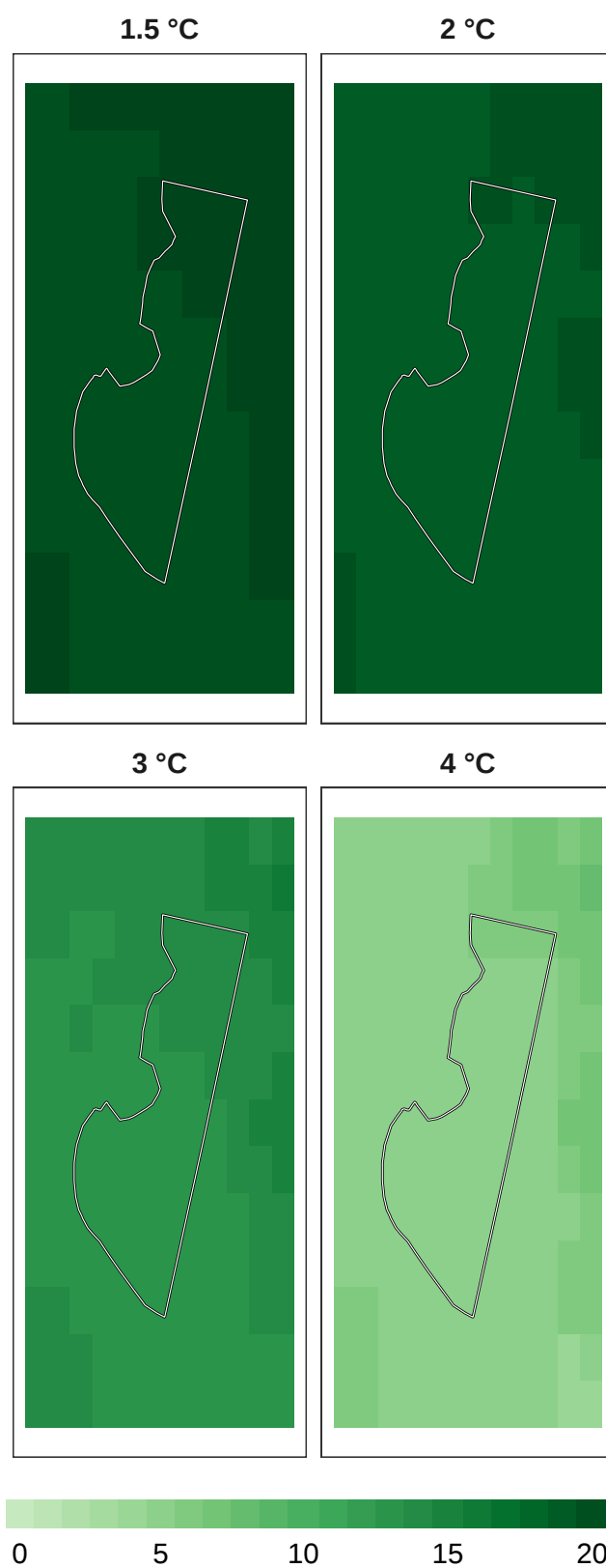
Figure 9: Number of models in agreement for mammal refugia at 1 km resolution.
