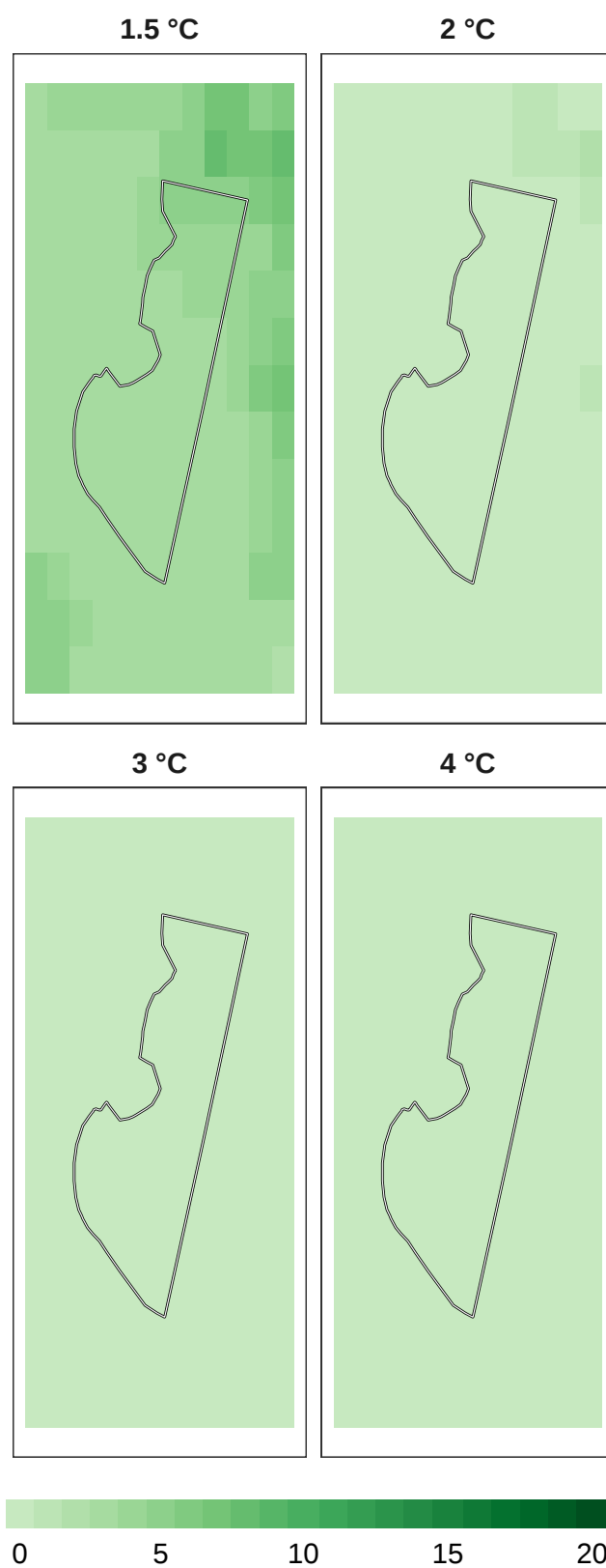
Figure 10: Number of models in agreement for insect refugia at 1 km resolution.
