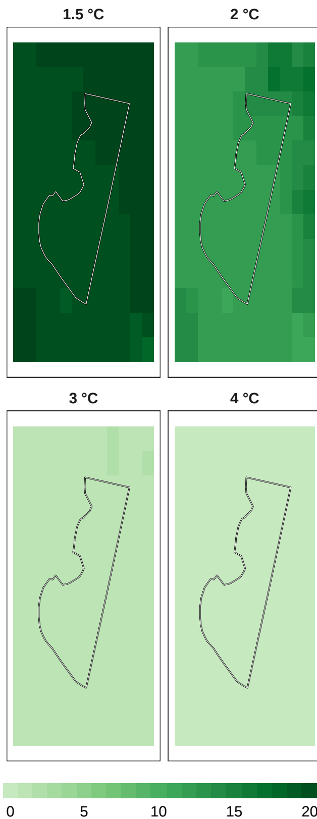
Figure 7: Number of models in agreement for plant refugia at 1 km resolution.
