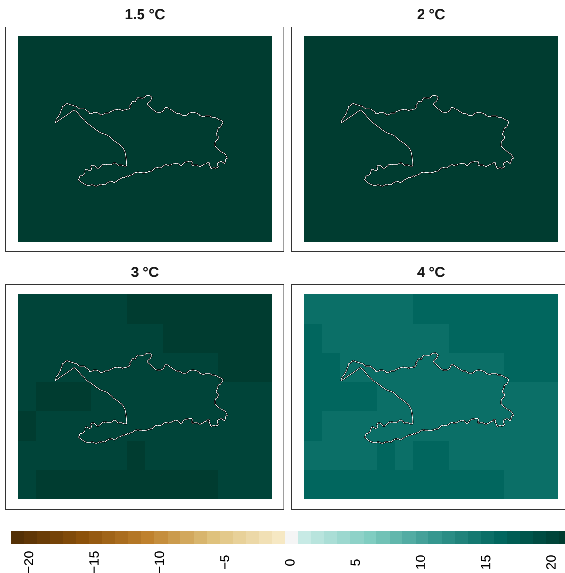
Figure 16: Adaptation effort for mammals at 1 km resolution.
