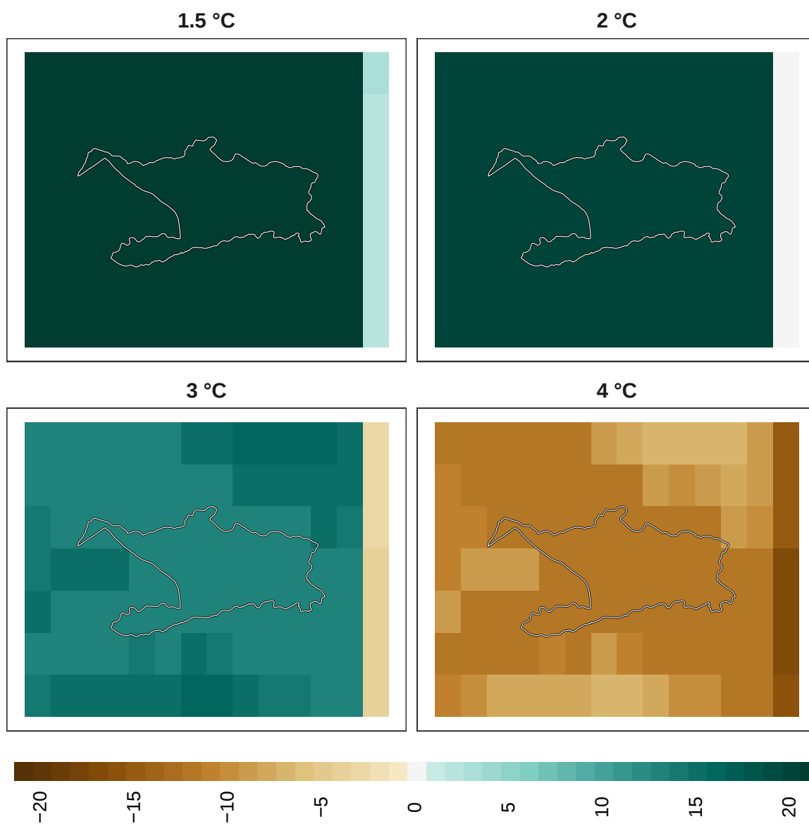
Figure 14: Adaptation effort for plants at 1 km resolution.
