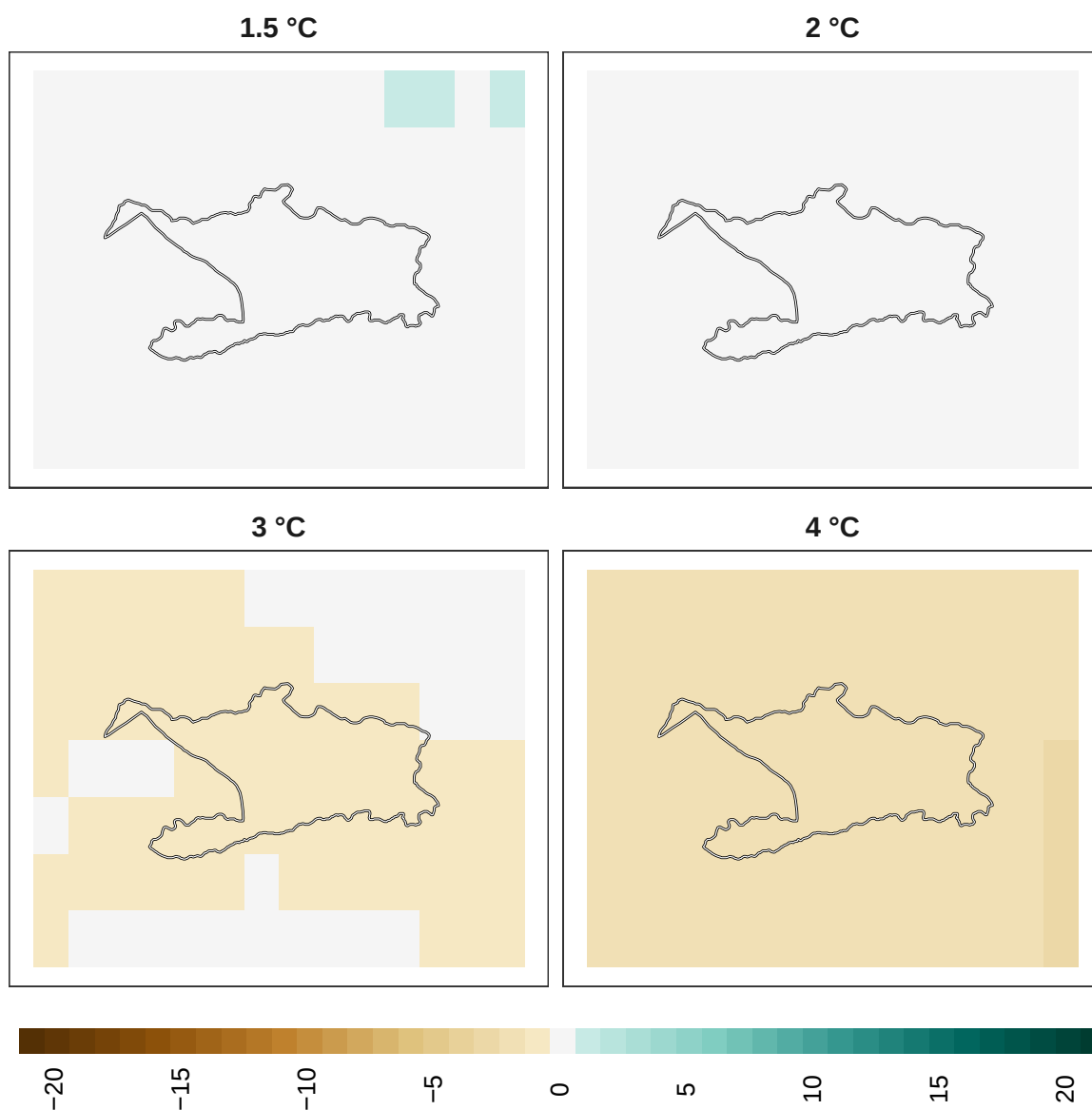
Figure 15: Adaptation effort for birds at 1 km resolution.
