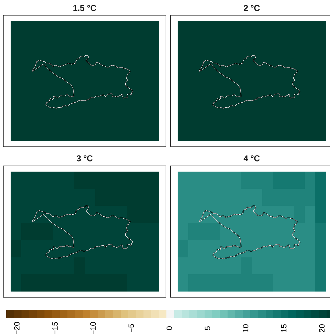
Figure 17: Adaptation effort for reptiles at 1 km resolution.
