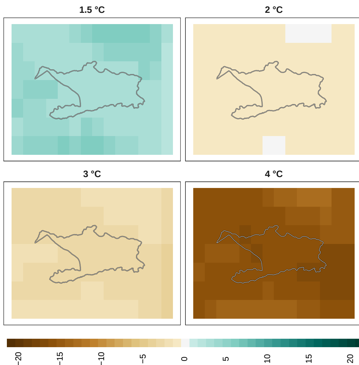
Figure 13: Adaptation effort for overall biodiversity at 1 km resolution.
