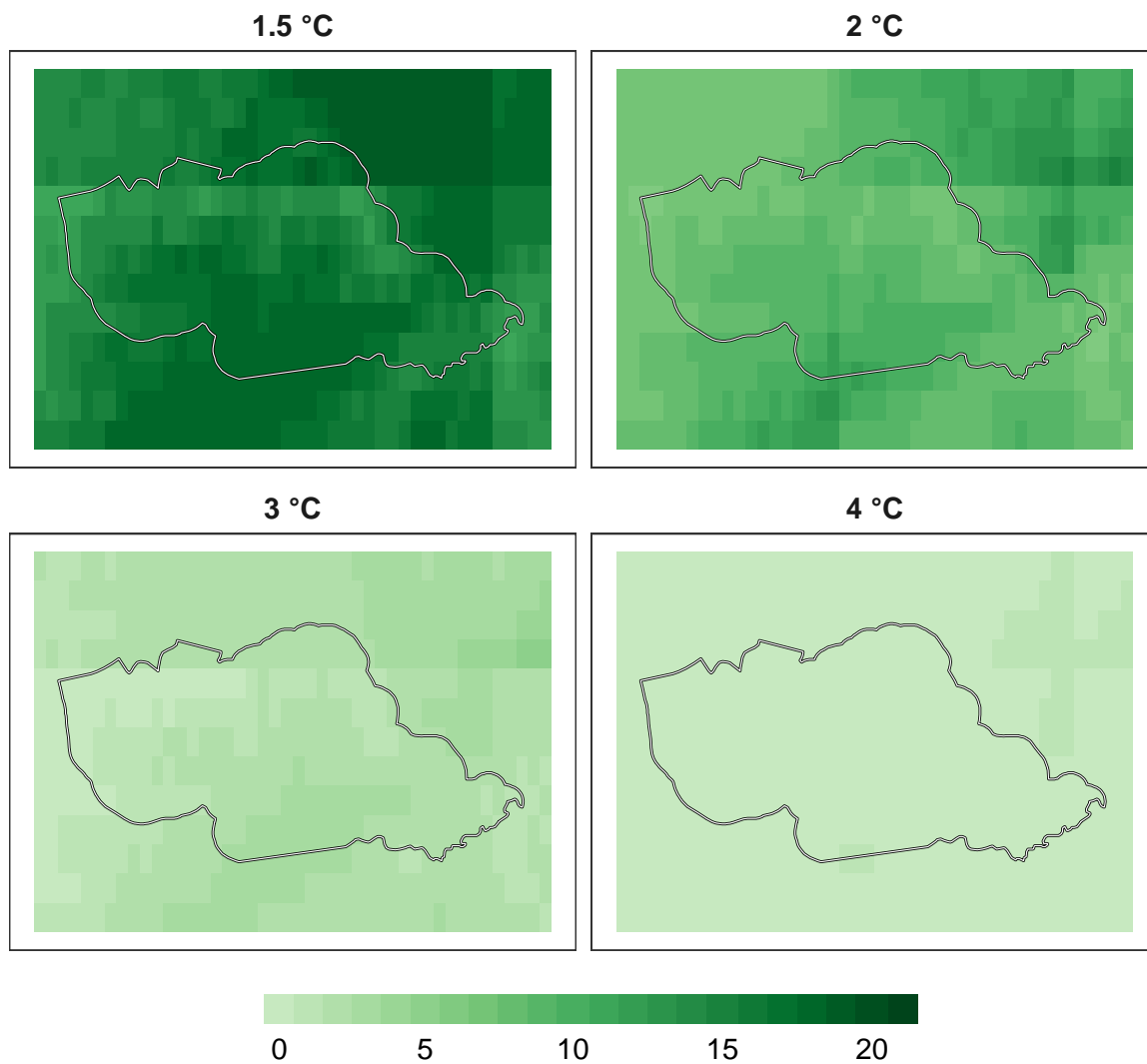
Figure 8: Number of models in agreement for insect refugia at 1 km resolution.
