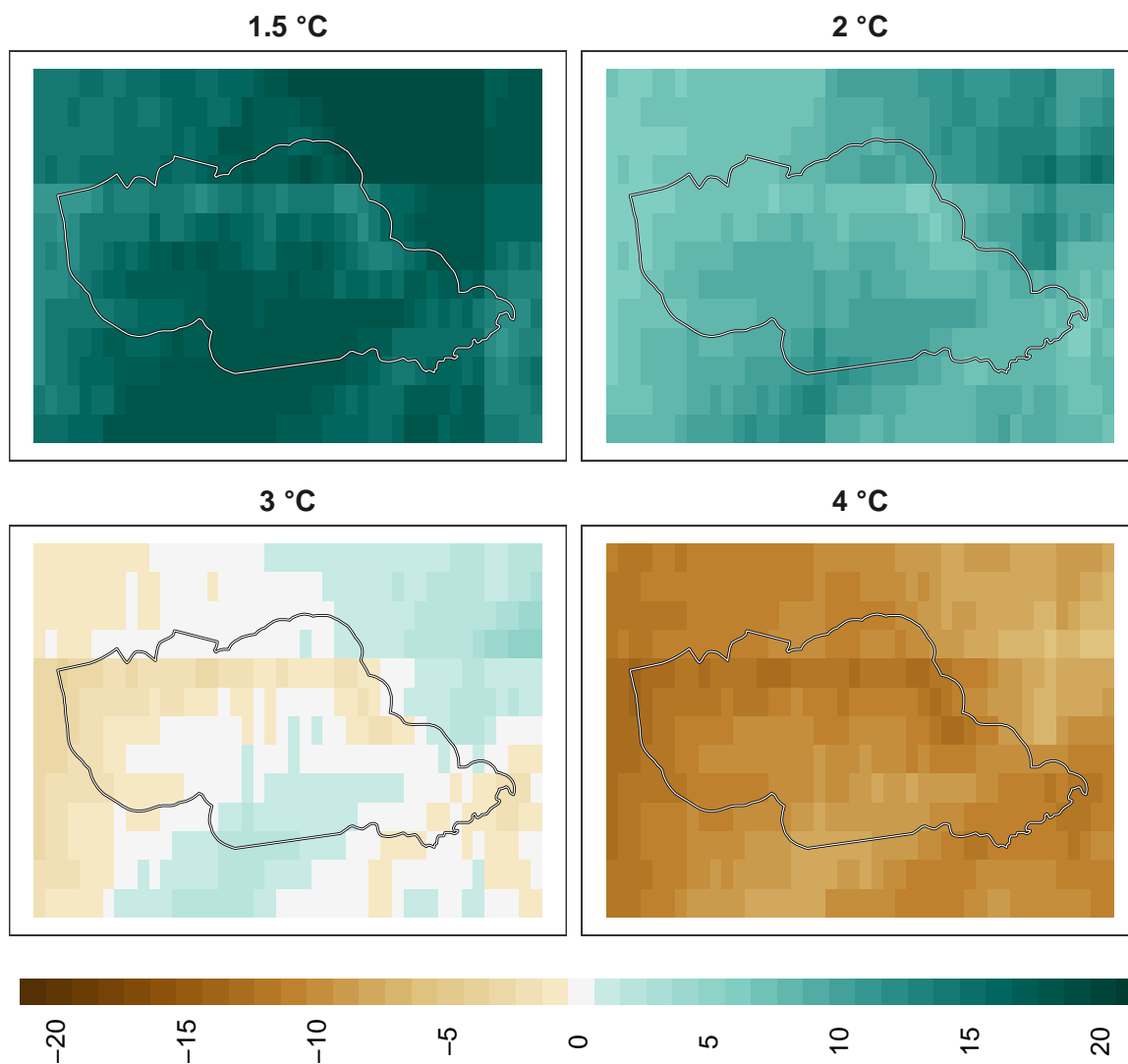
Figure 12: Adaptation effort for insects at 1 km resolution.
