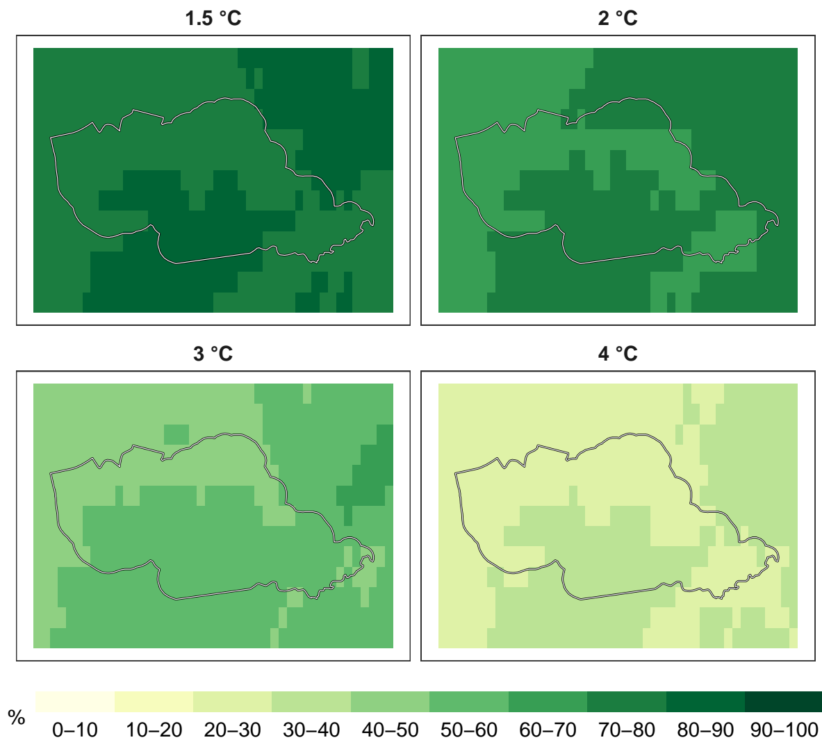
Figure 4: Percent insects remaining at 1 km resolution.
