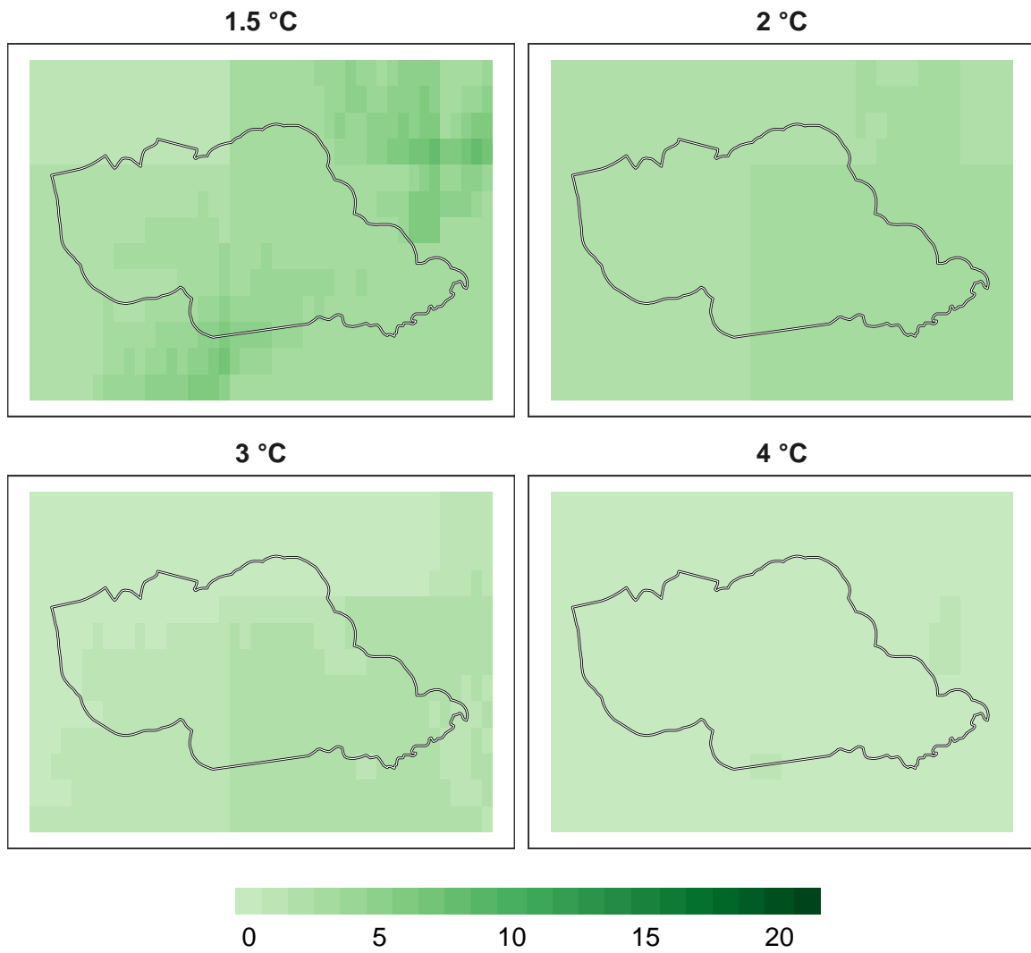
Figure 5: Number of models in agreement for overall biodiversity refugia at 1 km resolution.
