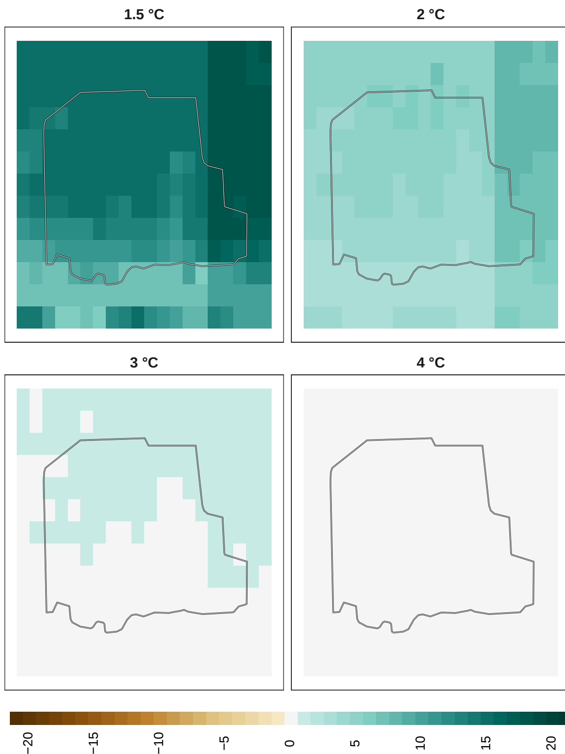
Figure 17: Adaptation effort for mammals at 1 km resolution.
