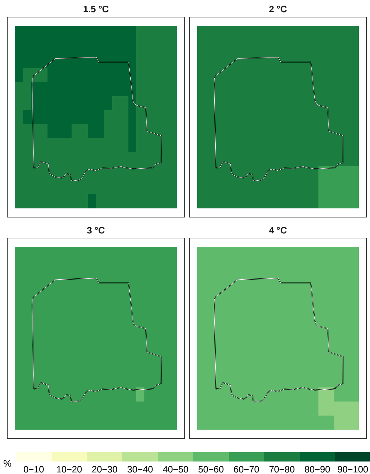
Figure 7: Percent timber species remaining at 1 km resolution.
