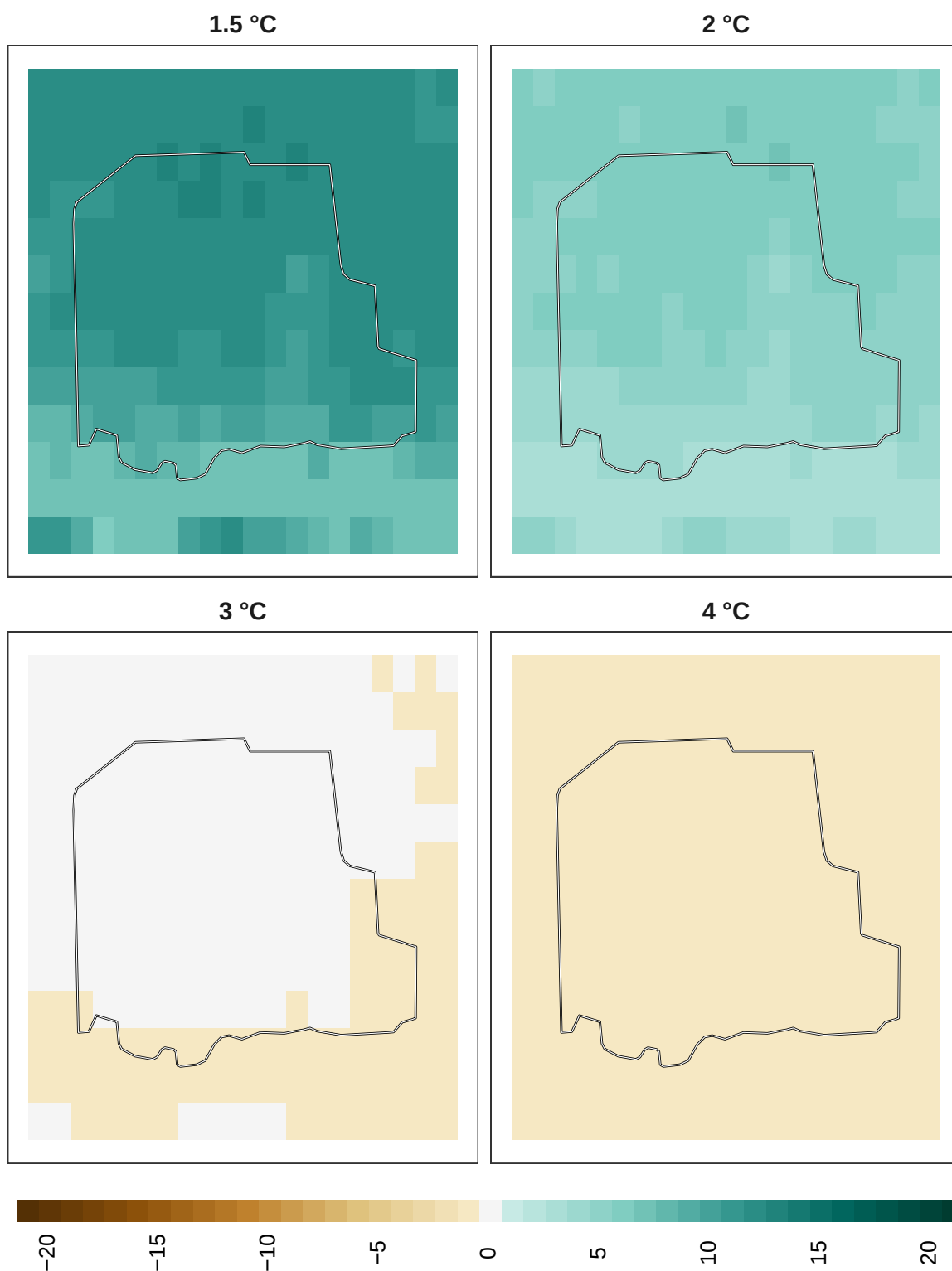
Figure 15: Adaptation effort for plants at 1 km resolution.
