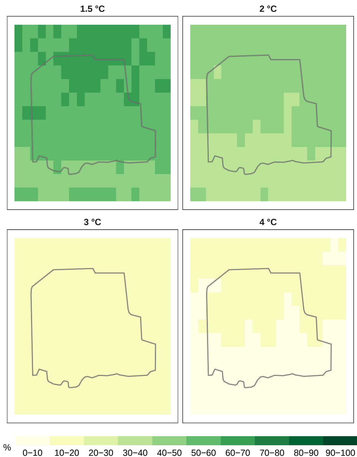
Figure 6: Percent pollinators remaining at 1 km resolution.
