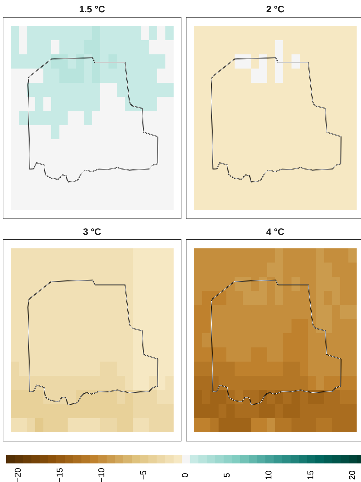
Figure 18: Adaptation effort for insects at 1 km resolution.
