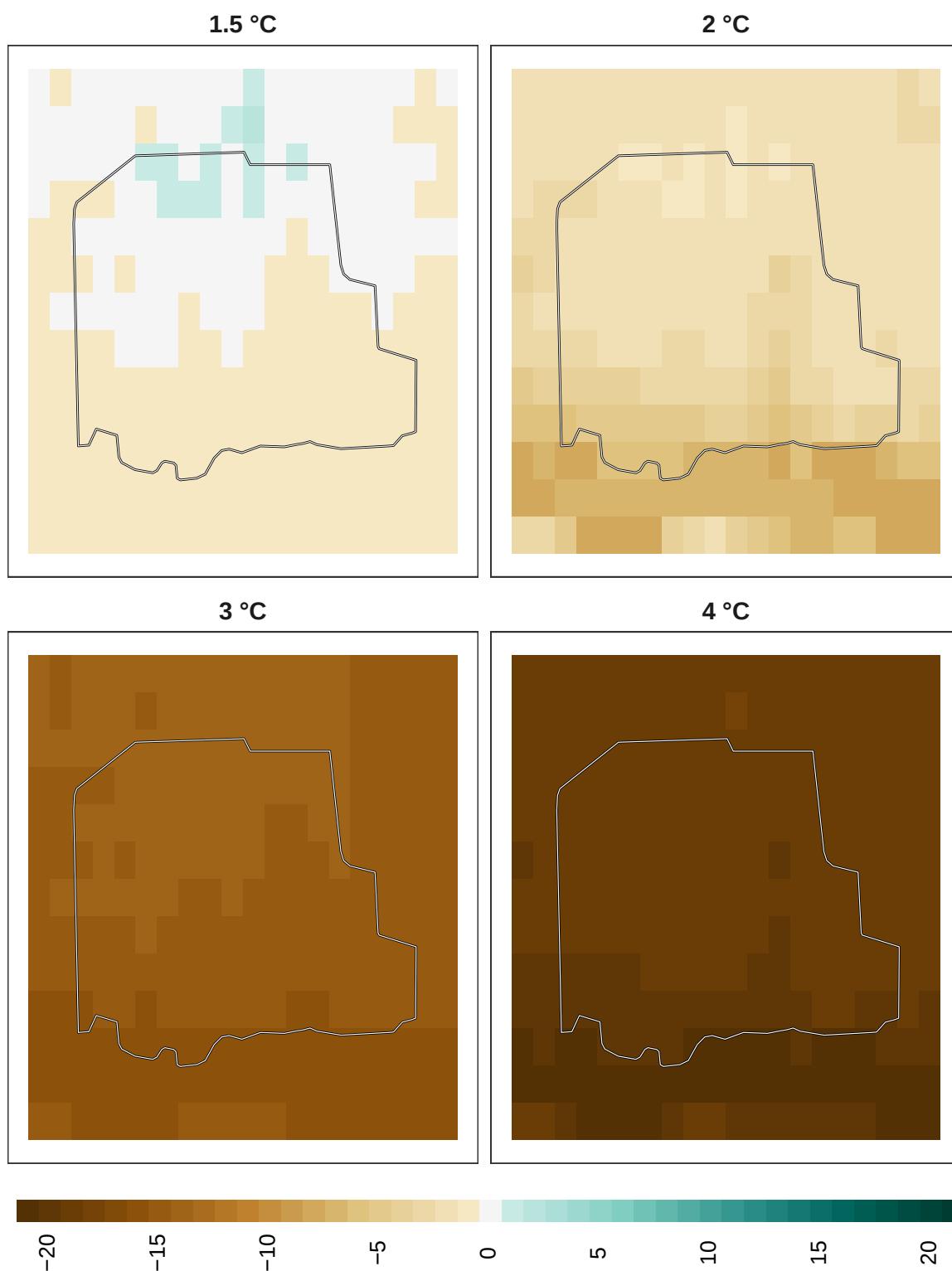
Figure 19: Adaptation effort for pollinators at 1 km resolution.
