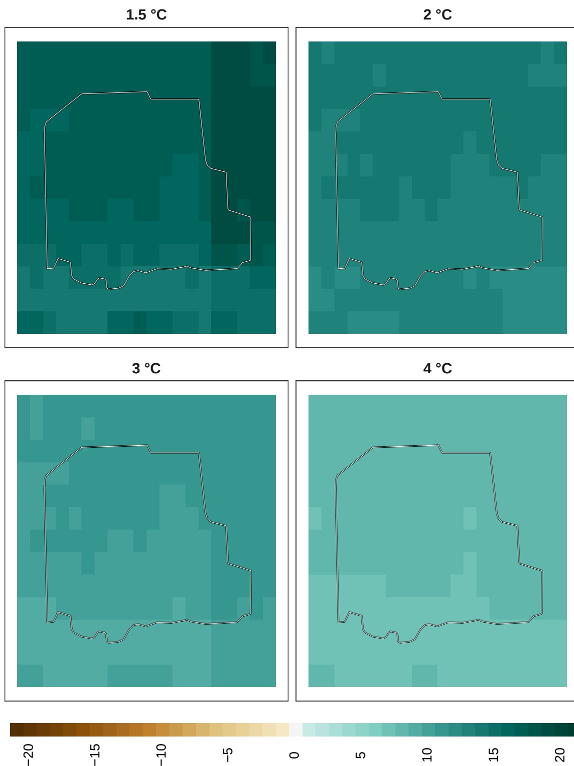
Figure 16: Adaptation effort for birds at 1 km resolution.
