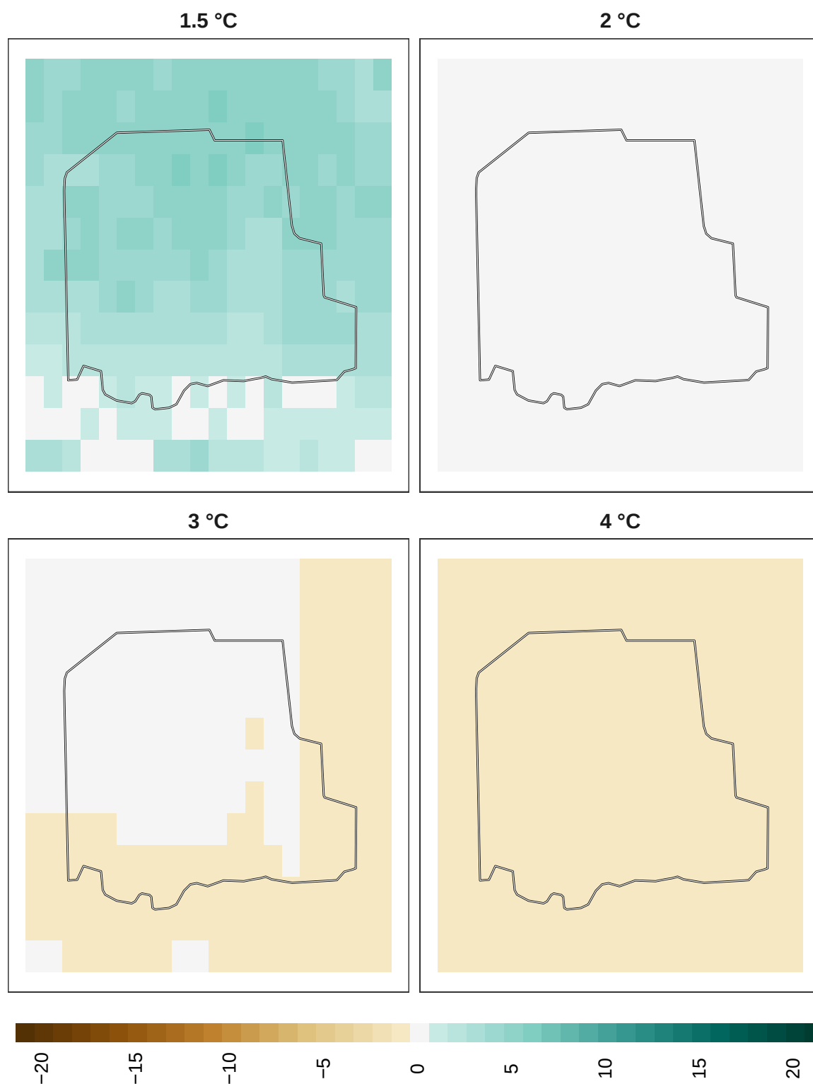
Figure 14: Adaptation effort for overall biodiversity at 1 km resolution.
