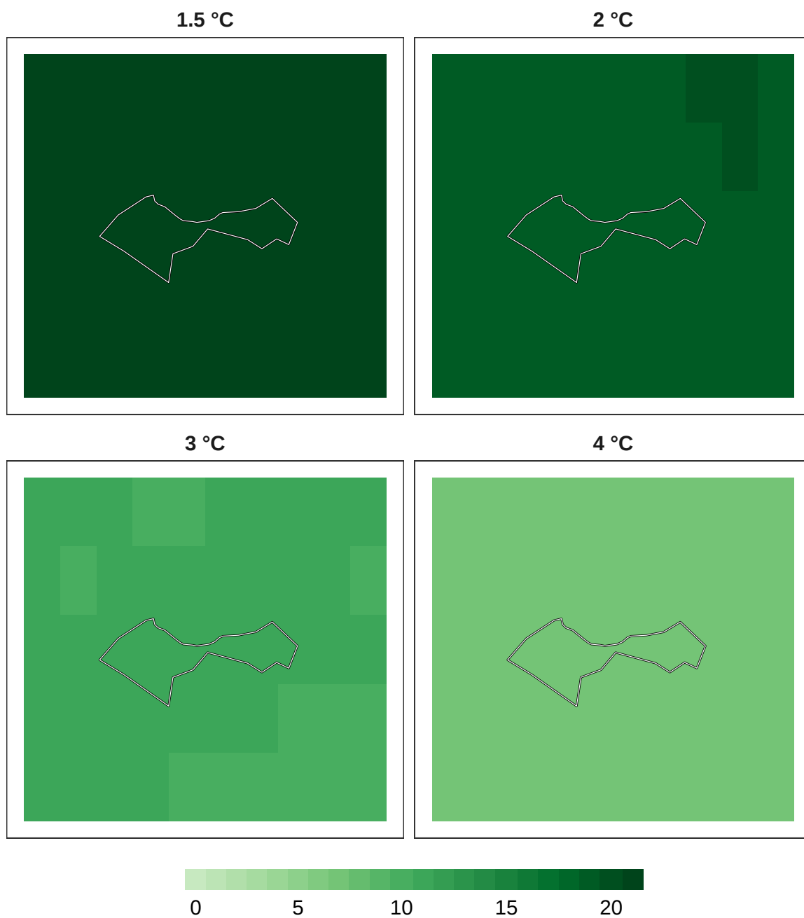
Figure 11: Number of models in agreement for bird refugia.
