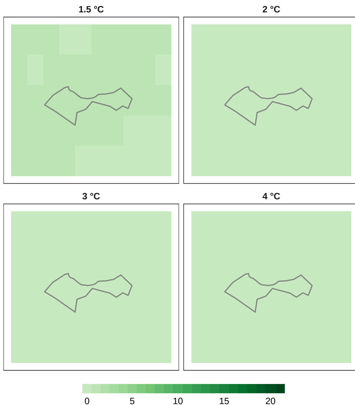
Figure 9: Number of models in agreement for overall biodiversity refugia at 1 km resolution.
