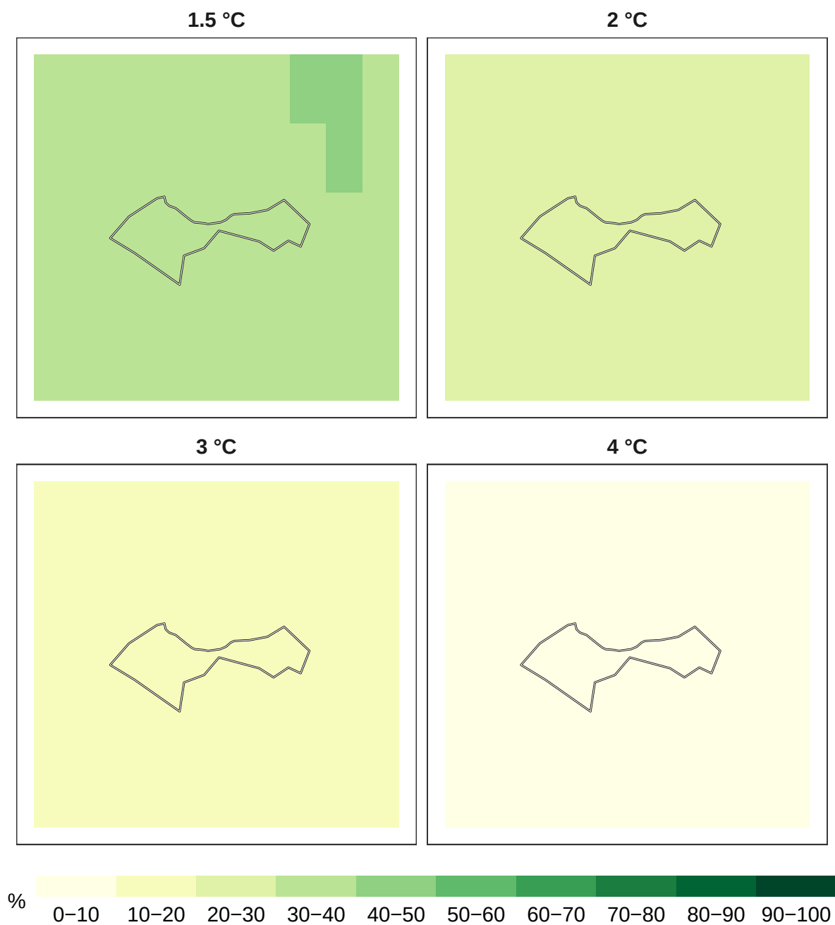
Figure 7: Percent pollinators remaining at 1 km resolution.
