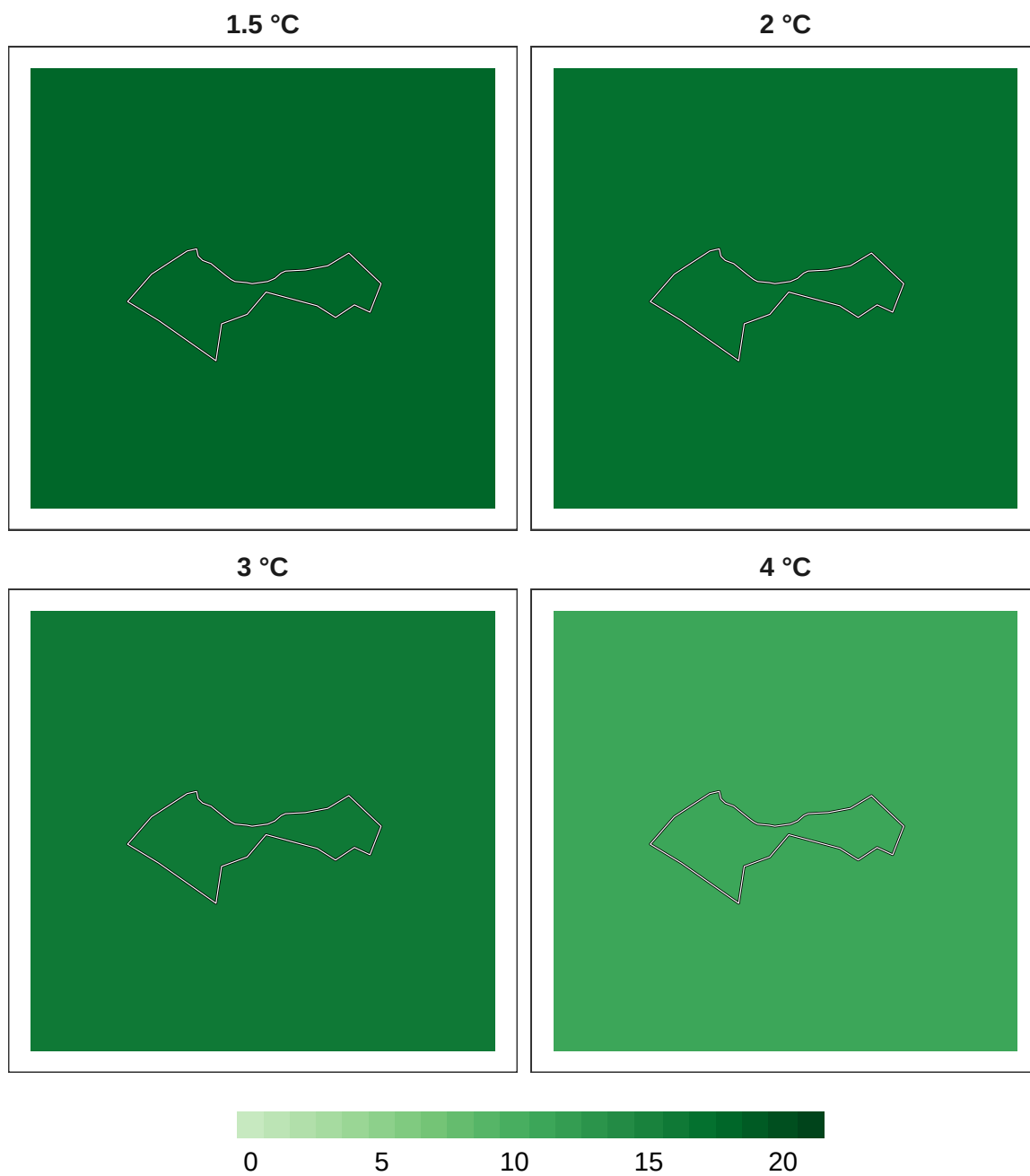
Figure 13: Number of models in agreement for reptile refugia at 1 km resolution.
