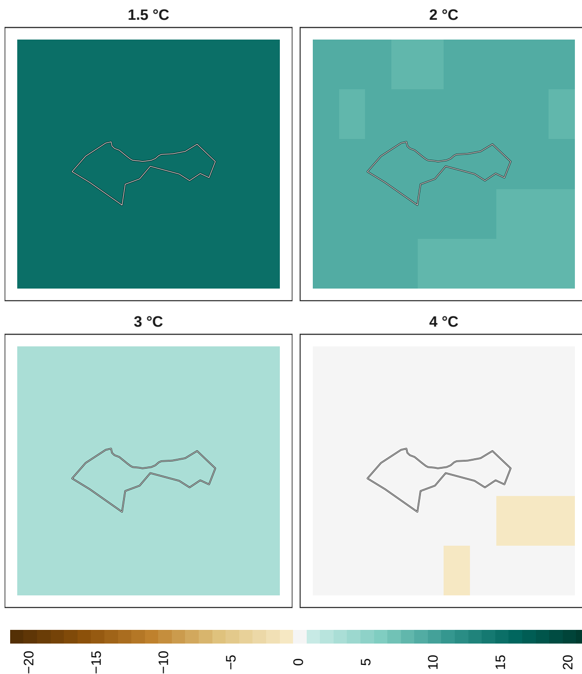
Figure 17: Adaptation effort for plants at 1 km resolution.
