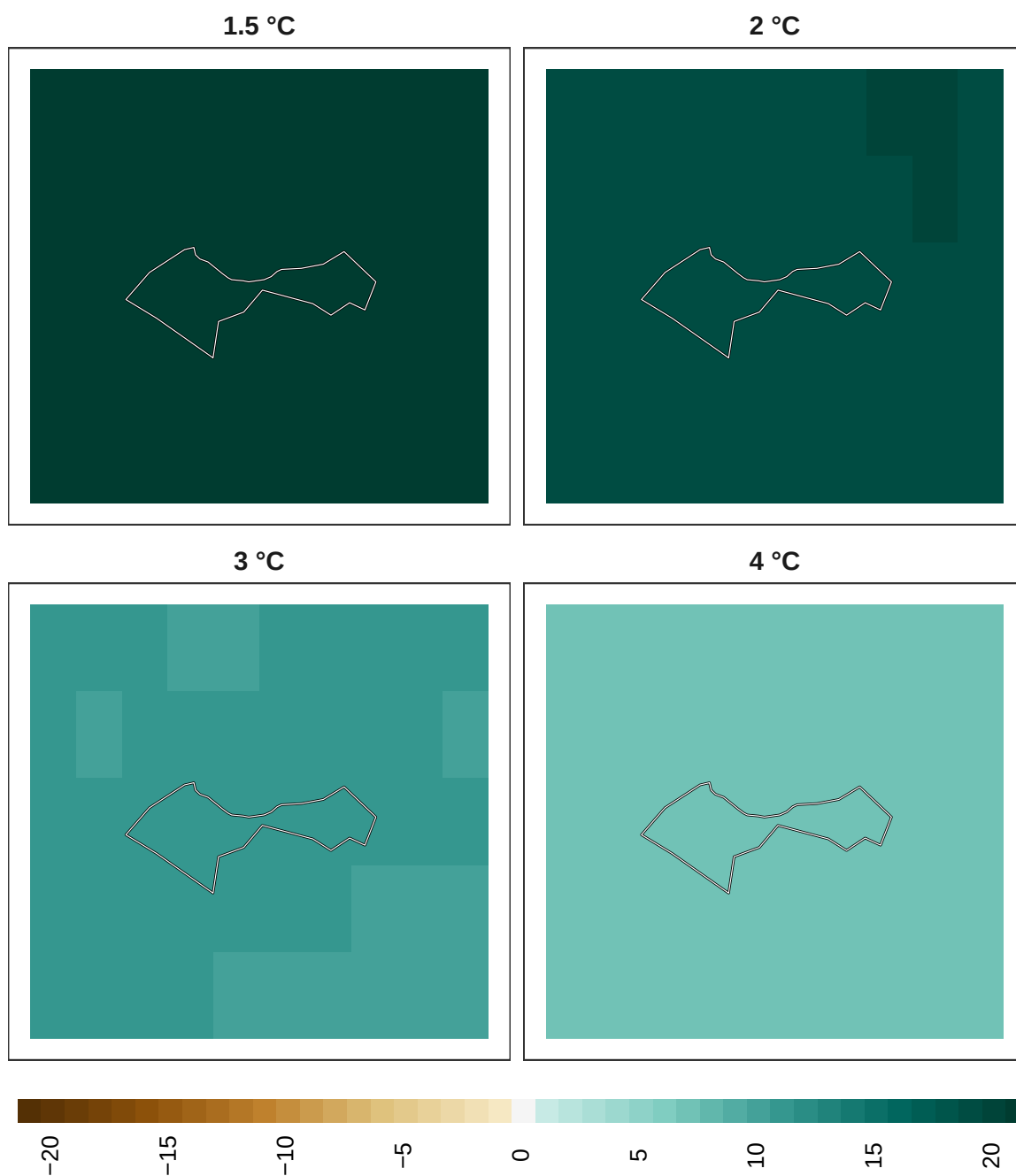
Figure 18: Adaptation effort for birds at 1 km resolution.
