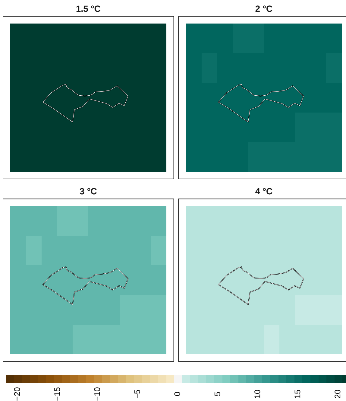
Figure 19: Adaptation effort for mammals at 1 km resolution.
