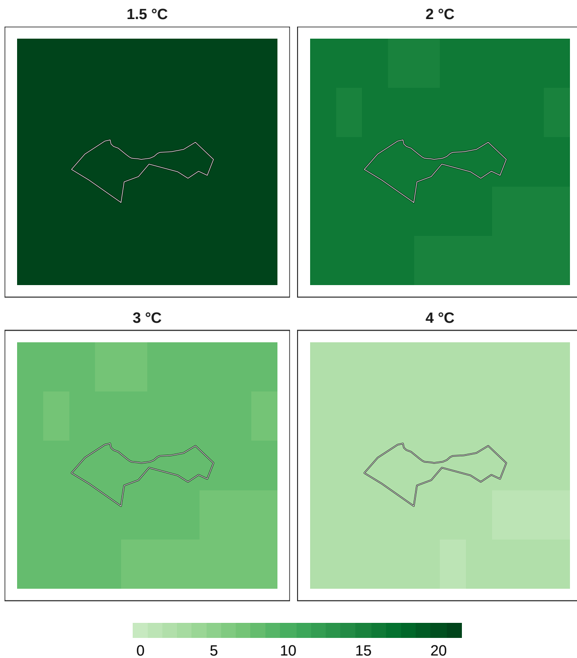
Figure 12: Number of models in agreement for mammal refugia at 1 km resolution.
