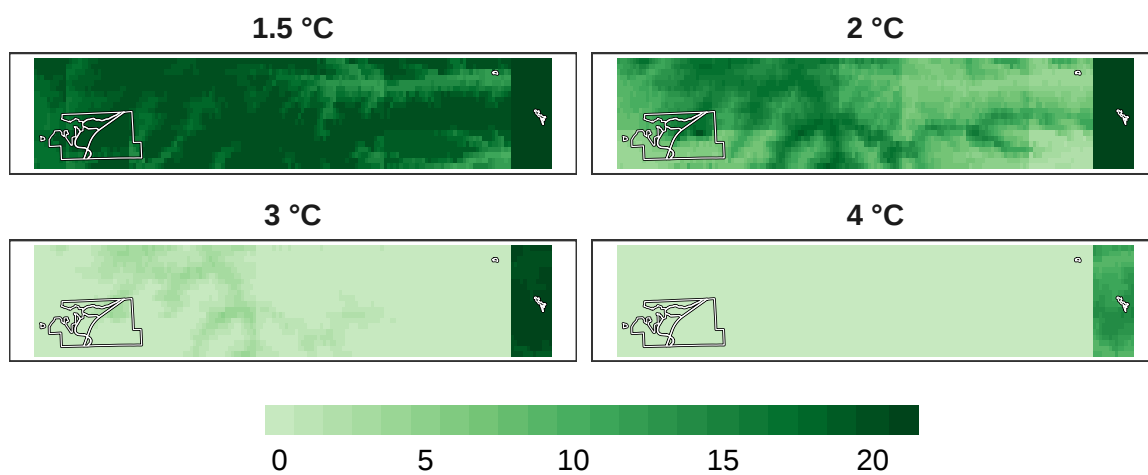
Figure 9: Number of models in agreement for mammal refugia at 1 km resolution.
