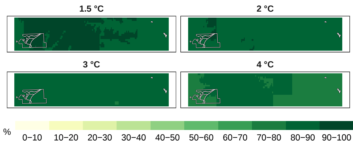
Figure 3: Percent birds remaining at 1 km resolution.
