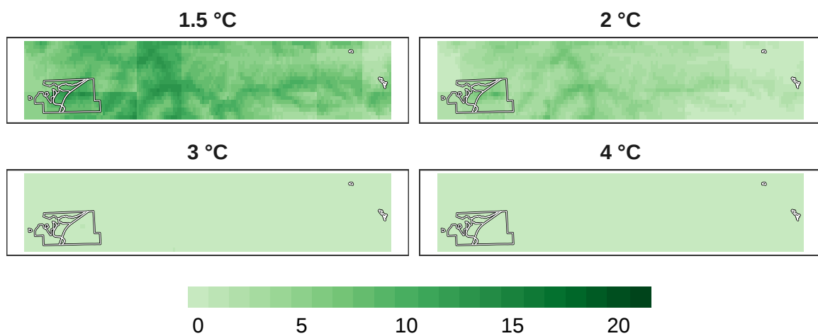
Figure 7: Number of models in agreement for plant refugia at 1 km resolution.
