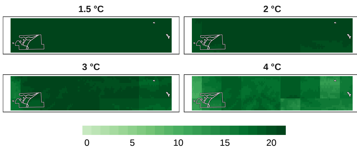
Figure 8: Number of models in agreement for bird refugia.
