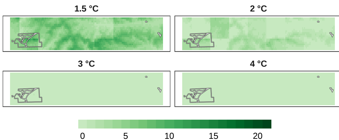
Figure 10: Number of models in agreement for insect refugia at 1 km resolution.
