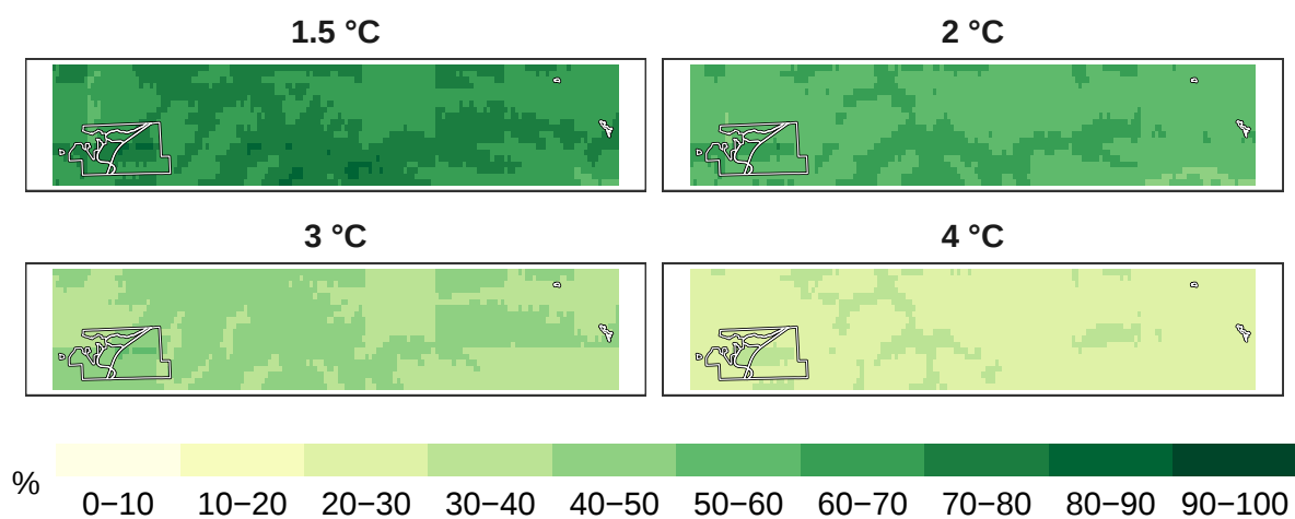
Figure 5: Percent insects remaining at 1 km resolution.
