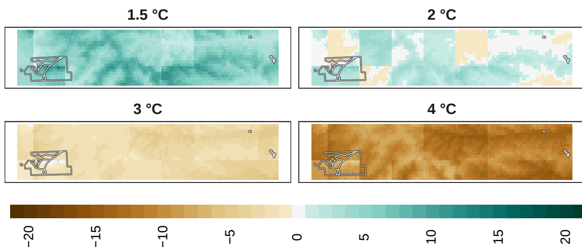
Figure 15: Adaptation effort for insects at 1 km resolution.
