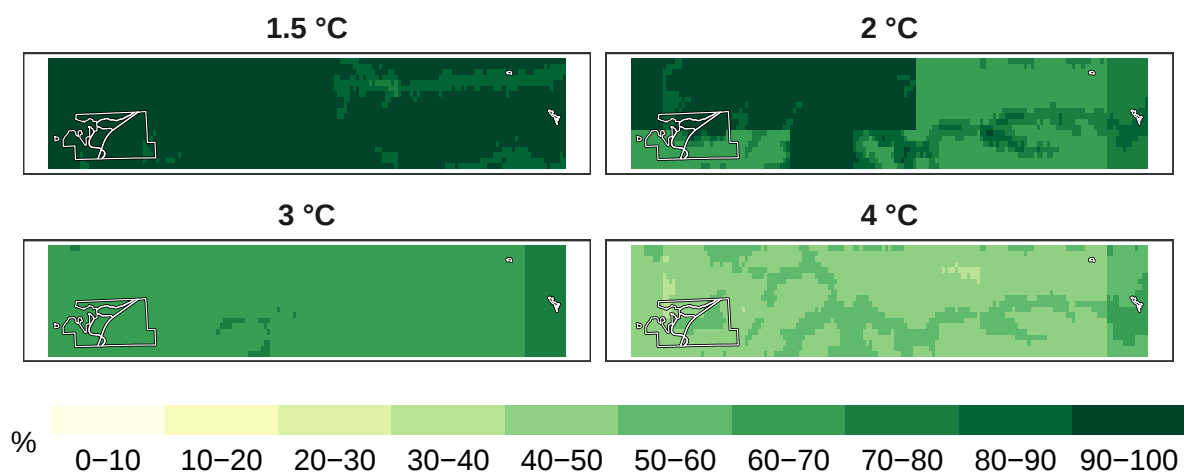
Figure 4: Percent mammals remaining at 1 km resolution.
