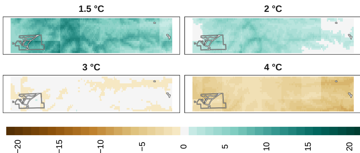
Figure 11: Adaptation effort for overall biodiversity at 1 km resolution.
