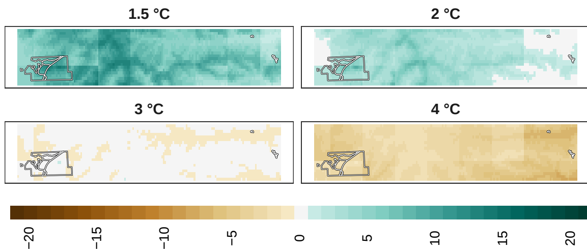
Figure 12: Adaptation effort for plants at 1 km resolution.
