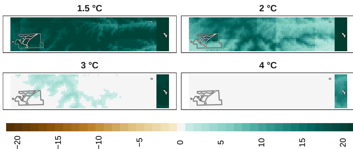
Figure 14: Adaptation effort for mammals at 1 km resolution.
