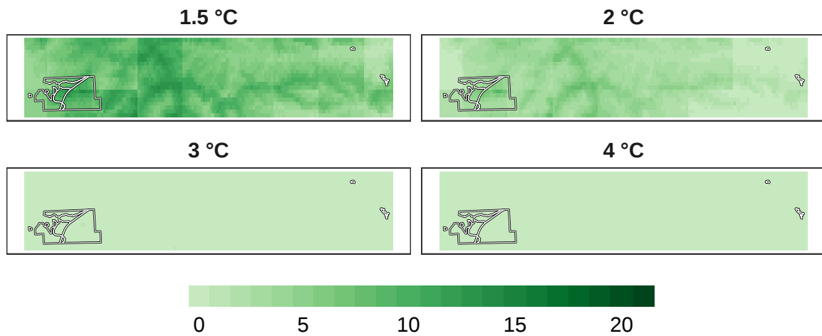
Figure 6: Number of models in agreement for overall biodiversity refugia at 1 km resolution.
