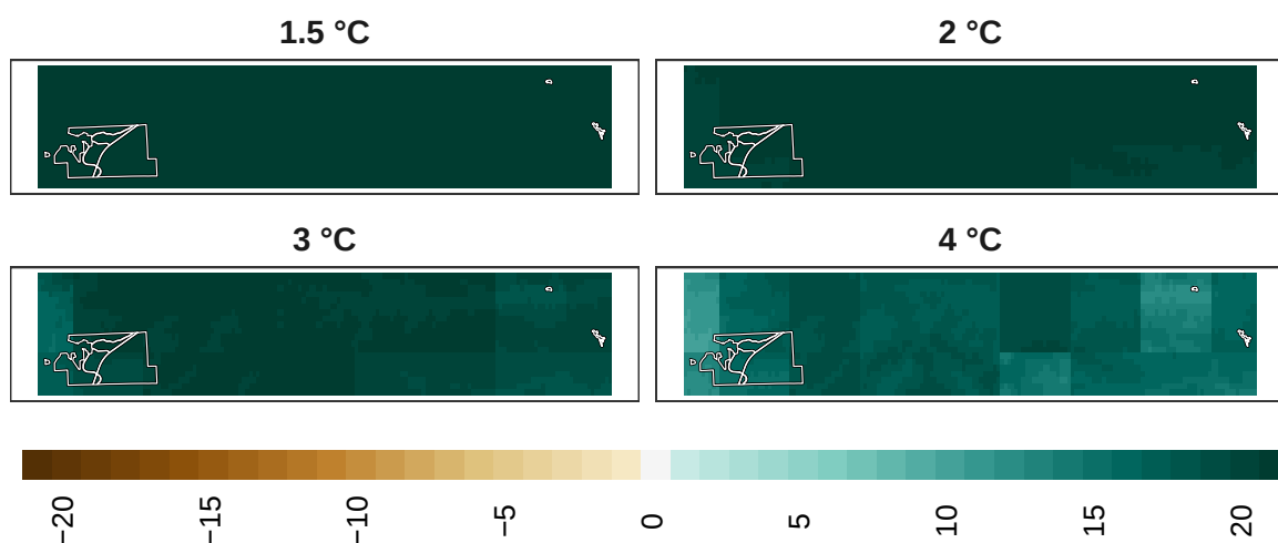
Figure 13: Adaptation effort for birds at 1 km resolution.
