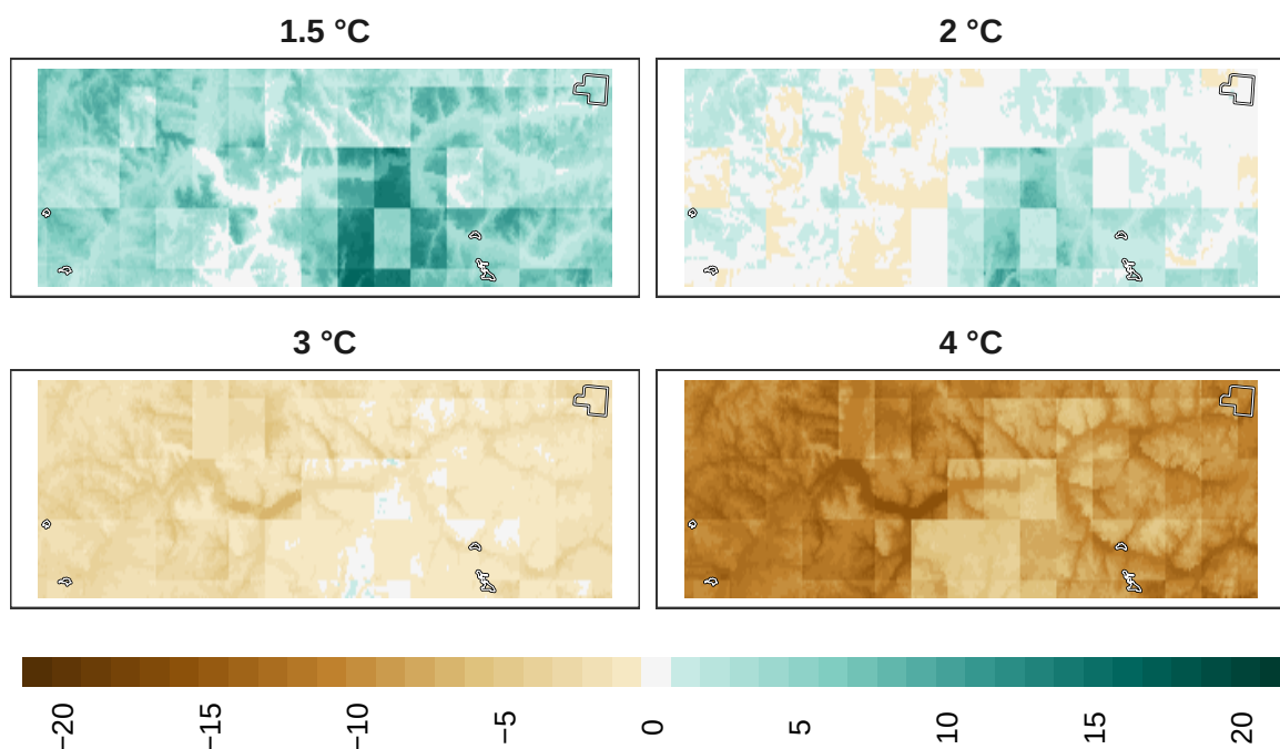
Figure 18: Adaptation effort for insects at 1 km resolution.
