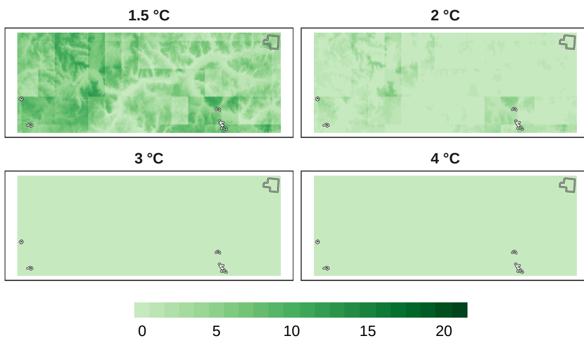
Figure 9: Number of models in agreement for plant refugia at 1 km resolution.
