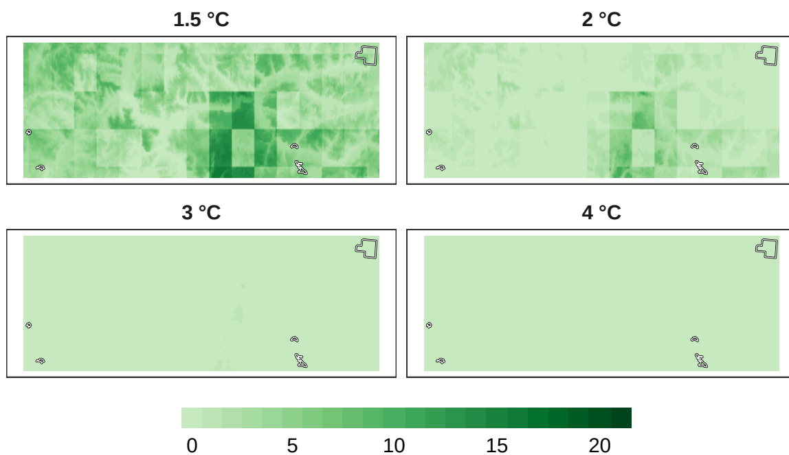
Figure 12: Number of models in agreement for insect refugia at 1 km resolution.
