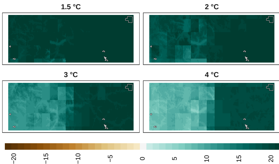
Figure 16: Adaptation effort for birds at 1 km resolution.
