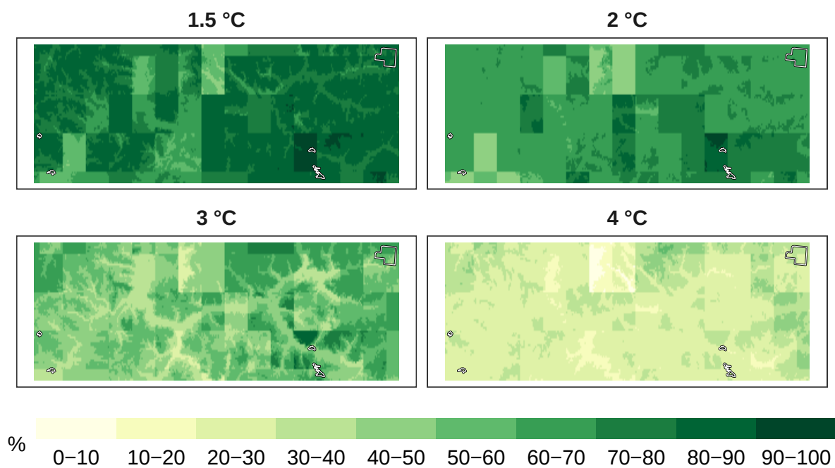
Figure 7: Percent timber species remaining at 1 km resolution.
