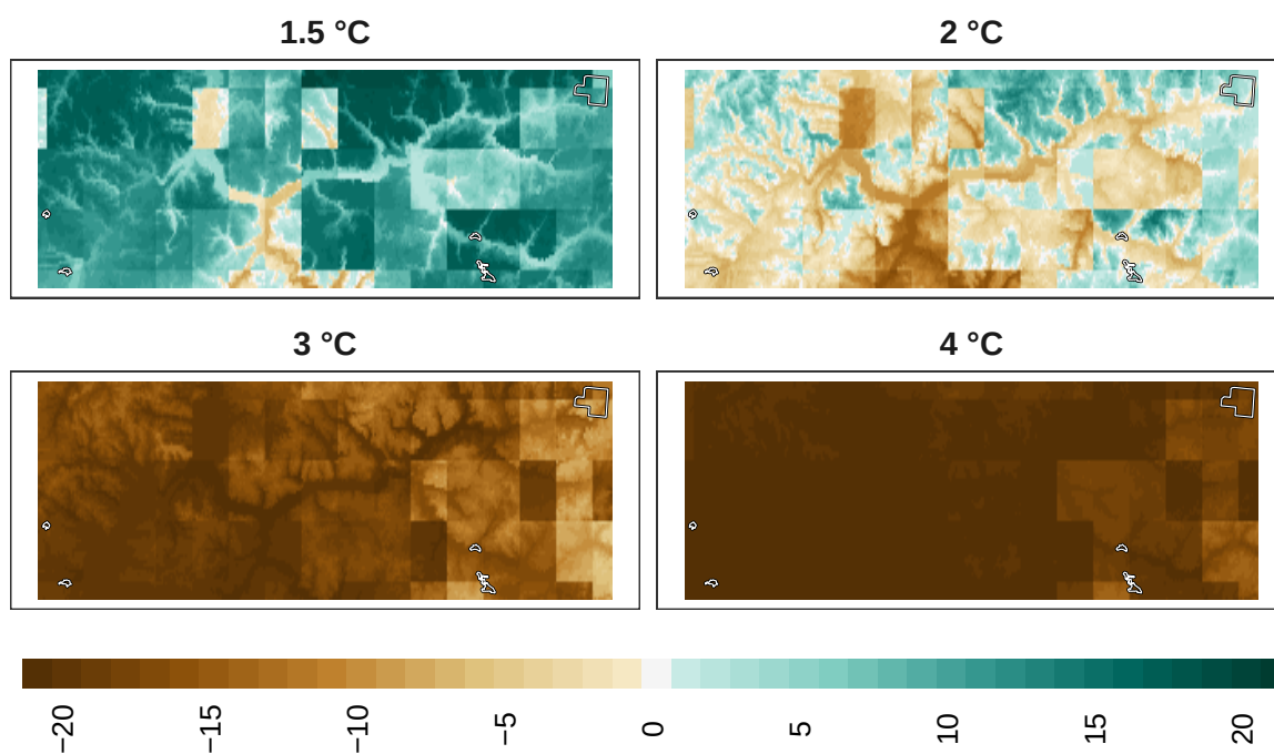
Figure 19: Adaptation effort for pollinators at 1 km resolution.
