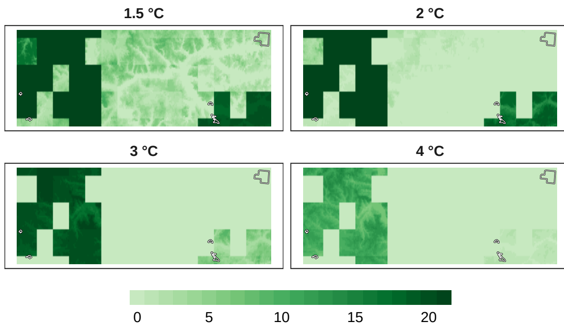
Figure 11: Number of models in agreement for mammal refugia at 1 km resolution.
