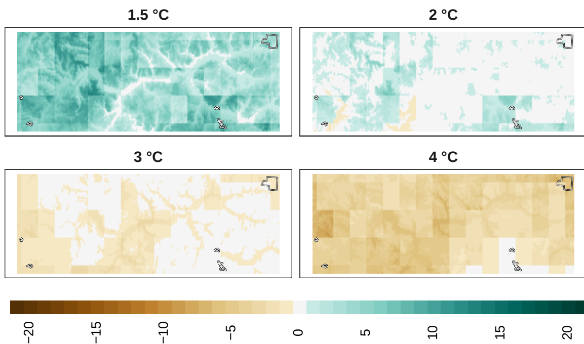
Figure 15: Adaptation effort for plants at 1 km resolution.
