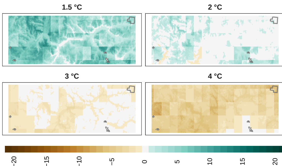
Figure 14: Adaptation effort for overall biodiversity at 1 km resolution.
