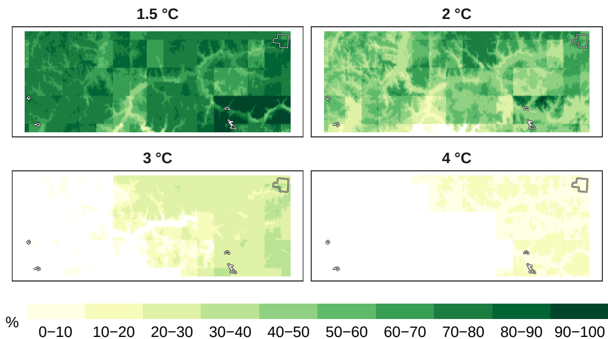
Figure 6: Percent pollinators remaining at 1 km resolution.
