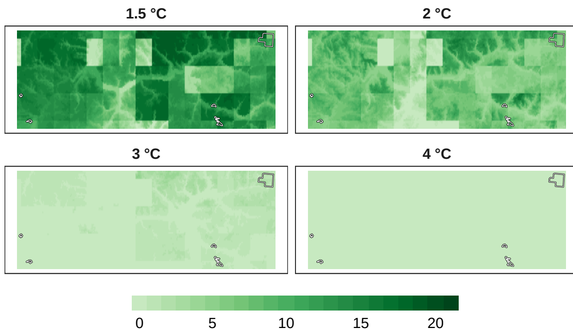
Figure 13: Number of models in agreement for pollinator refugia at 1 km resolution.
