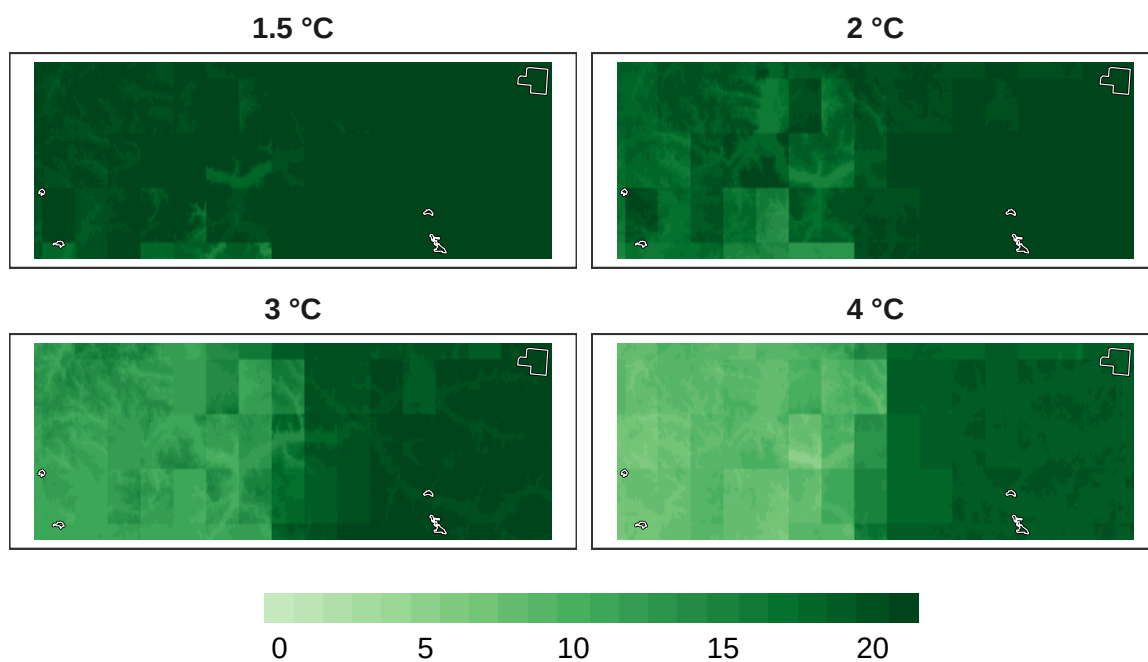
Figure 10: Number of models in agreement for bird refugia.
