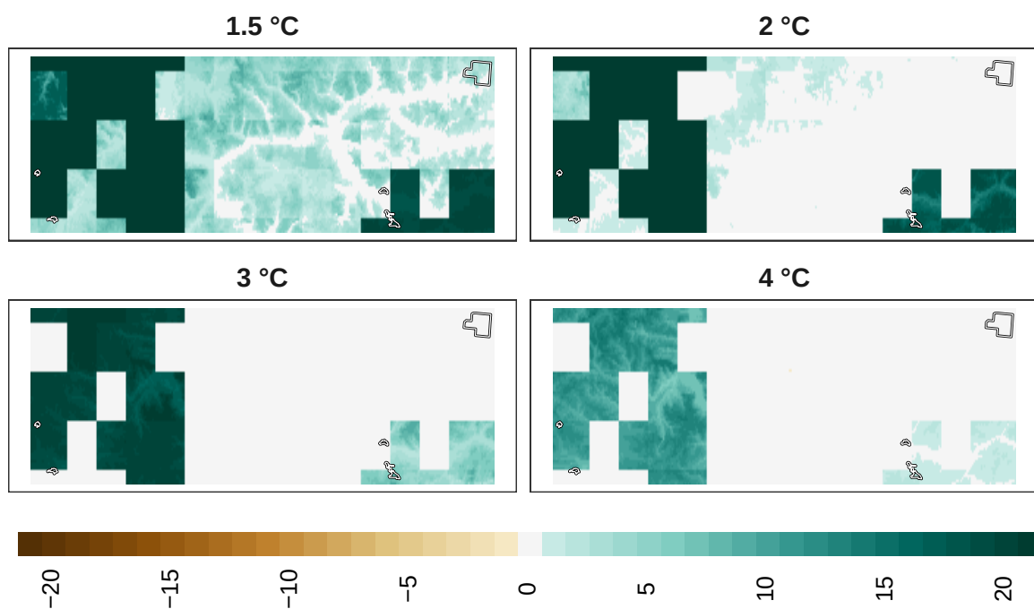
Figure 17: Adaptation effort for mammals at 1 km resolution.
