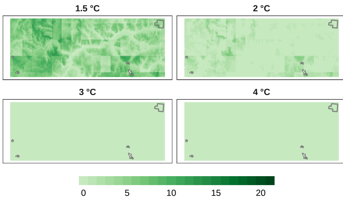
Figure 8: Number of models in agreement for overall biodiversity refugia at 1 km resolution.
