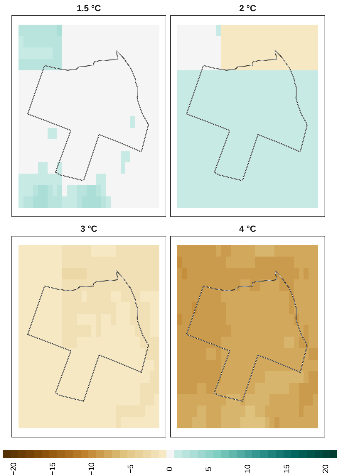
Figure 9: Adaptation effort for overall biodiversity at 1 km resolution.
