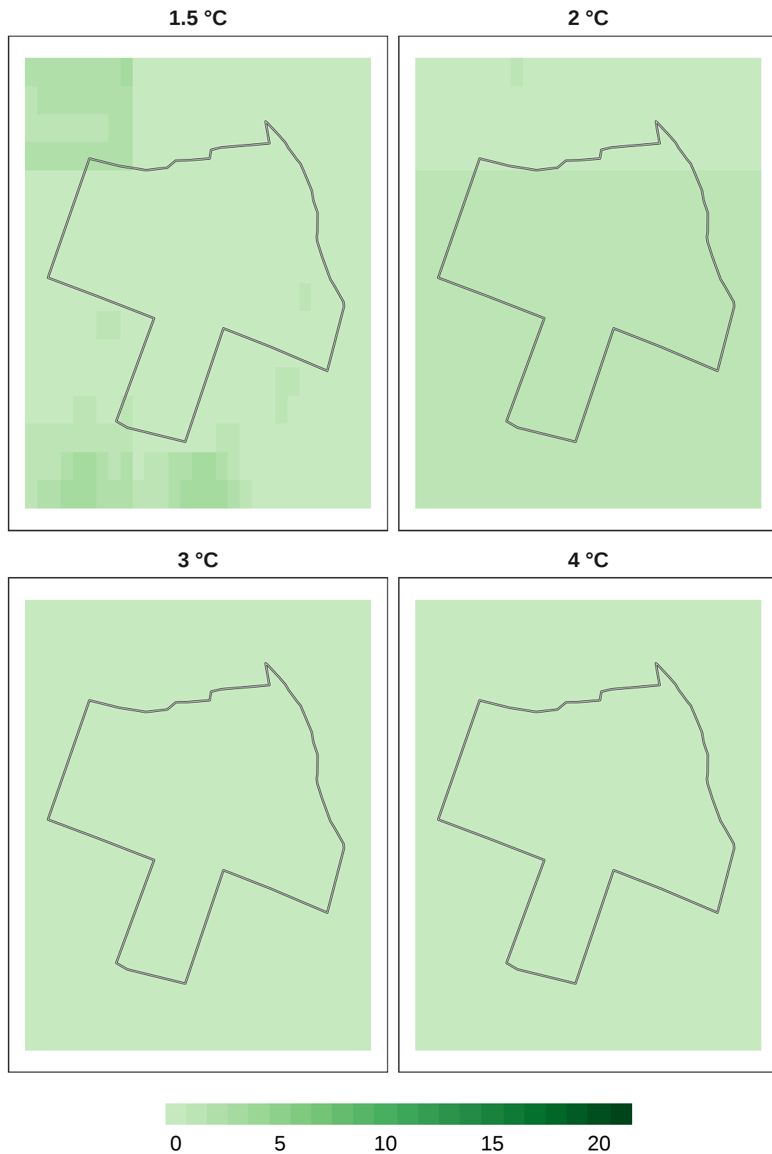
Figure 6: Number of models in agreement for plant refugia at 1 km resolution.
