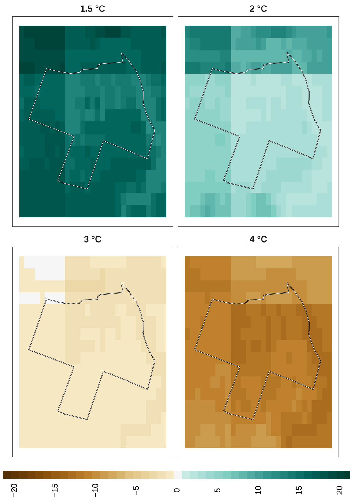
Figure 12: Adaptation effort for insects at 1 km resolution.
