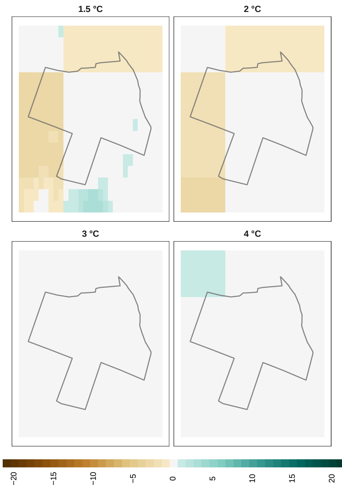
Figure 11: Adaptation effort for birds at 1 km resolution.
