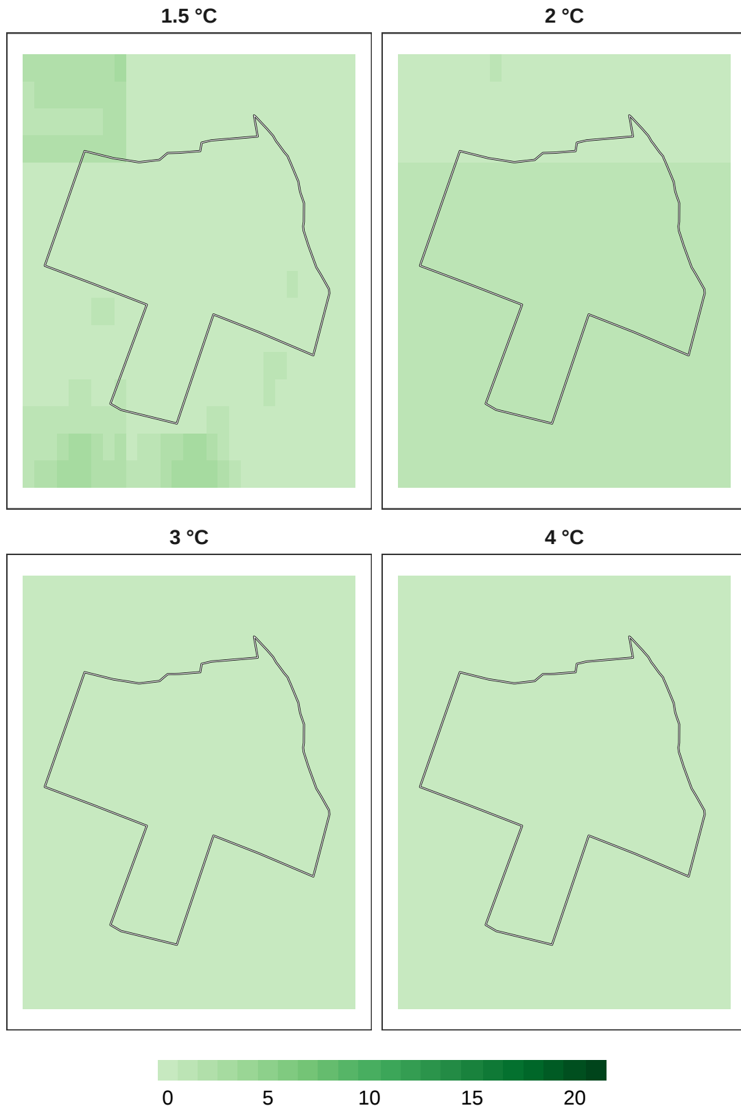
Figure 5: Number of models in agreement for overall biodiversity refugia at 1 km resolution.
