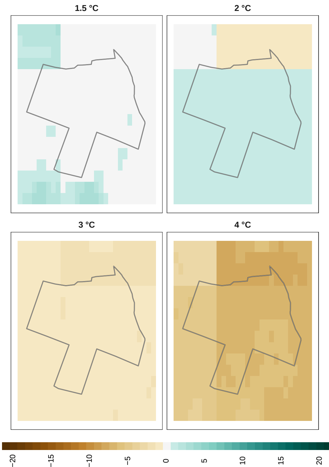
Figure 10: Adaptation effort for plants at 1 km resolution.
