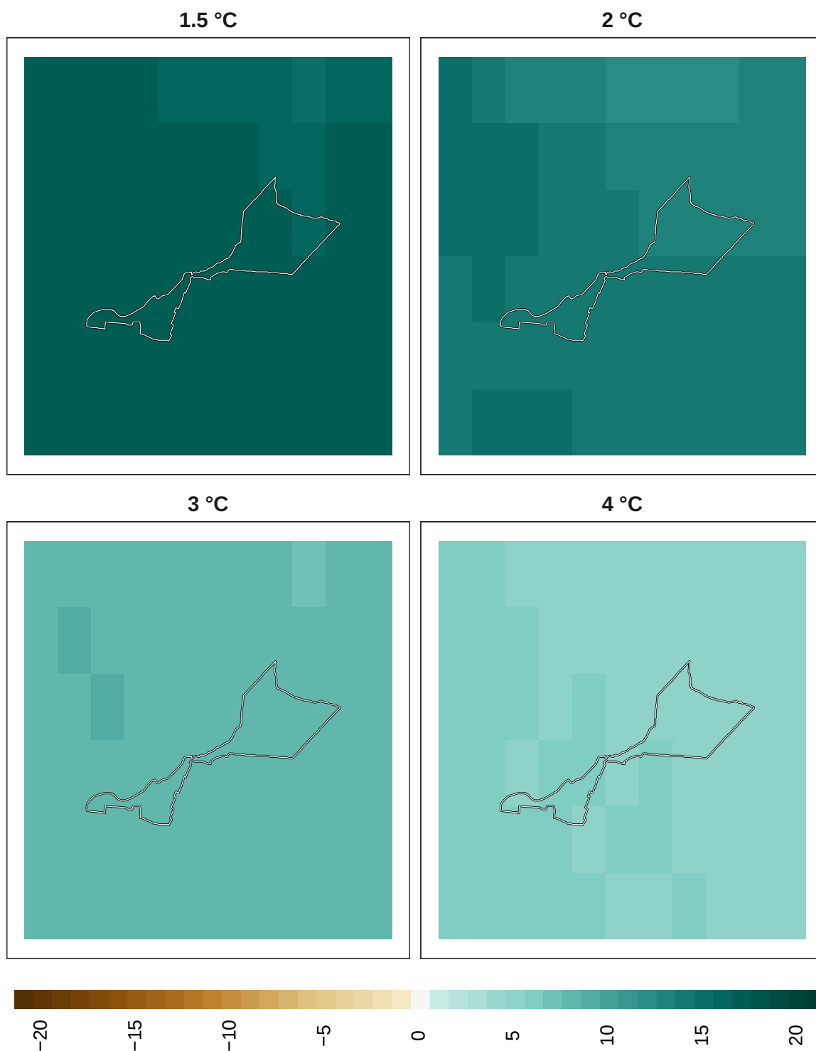
Figure 18: Adaptation effort for birds at 1 km resolution.
