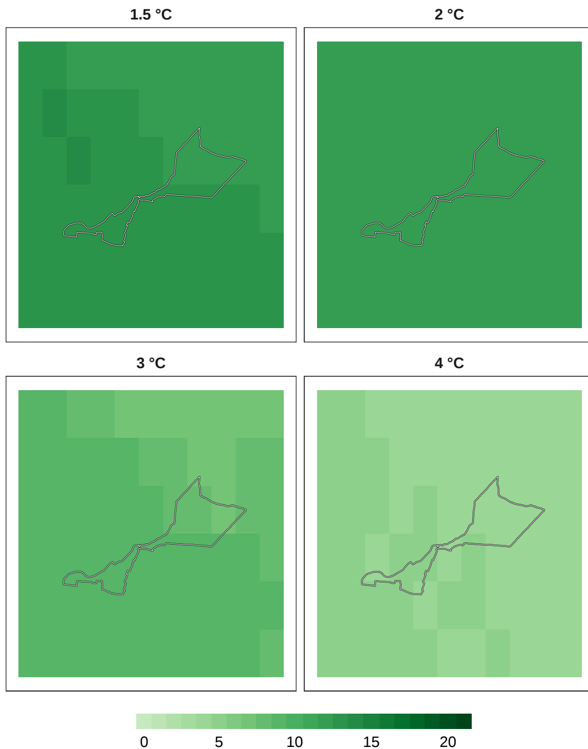
Figure 13: Number of models in agreement for reptile refugia at 1 km resolution.
