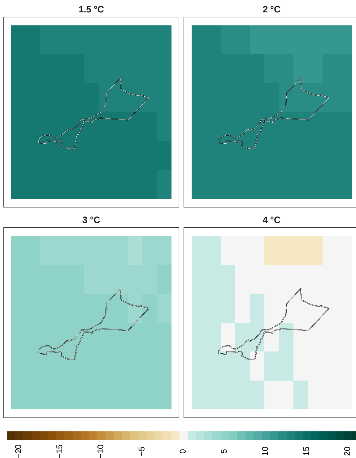
Figure 19: Adaptation effort for mammals at 1 km resolution.
