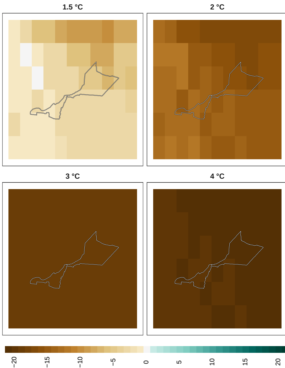
Figure 22: Adaptation effort for pollinators at 1 km resolution.
