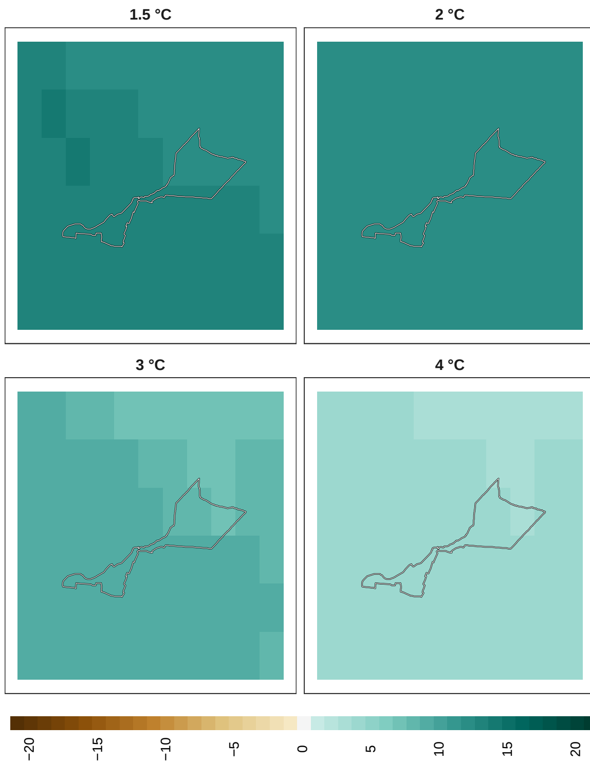
Figure 20: Adaptation effort for reptiles at 1 km resolution.
