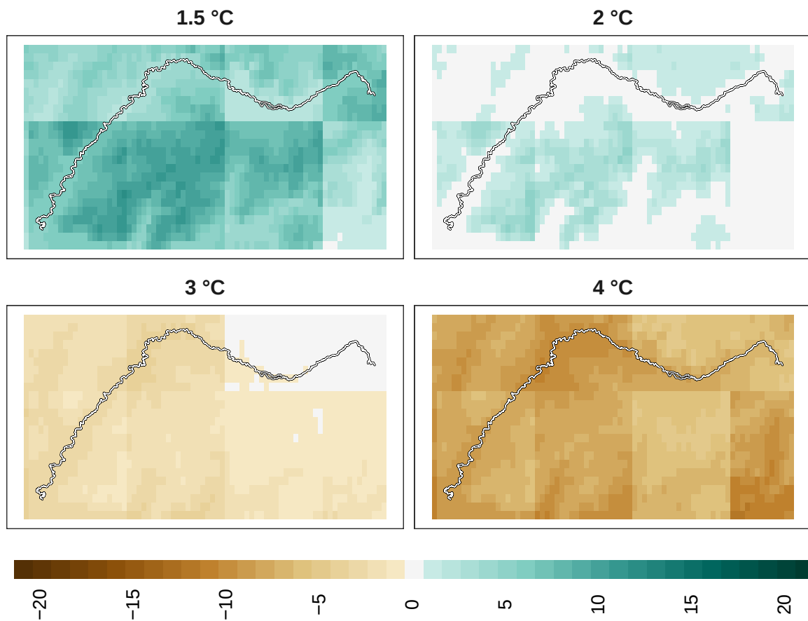
Figure 15: Adaptation effort for plants at 1 km resolution.
