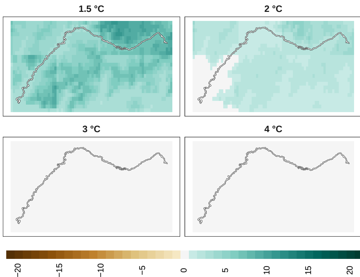
Figure 17: Adaptation effort for mammals at 1 km resolution.
