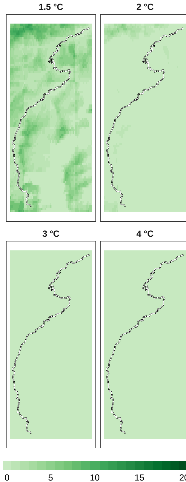
Figure 7: Number of models in agreement for overall biodiversity refugia at 1 km resolution.
