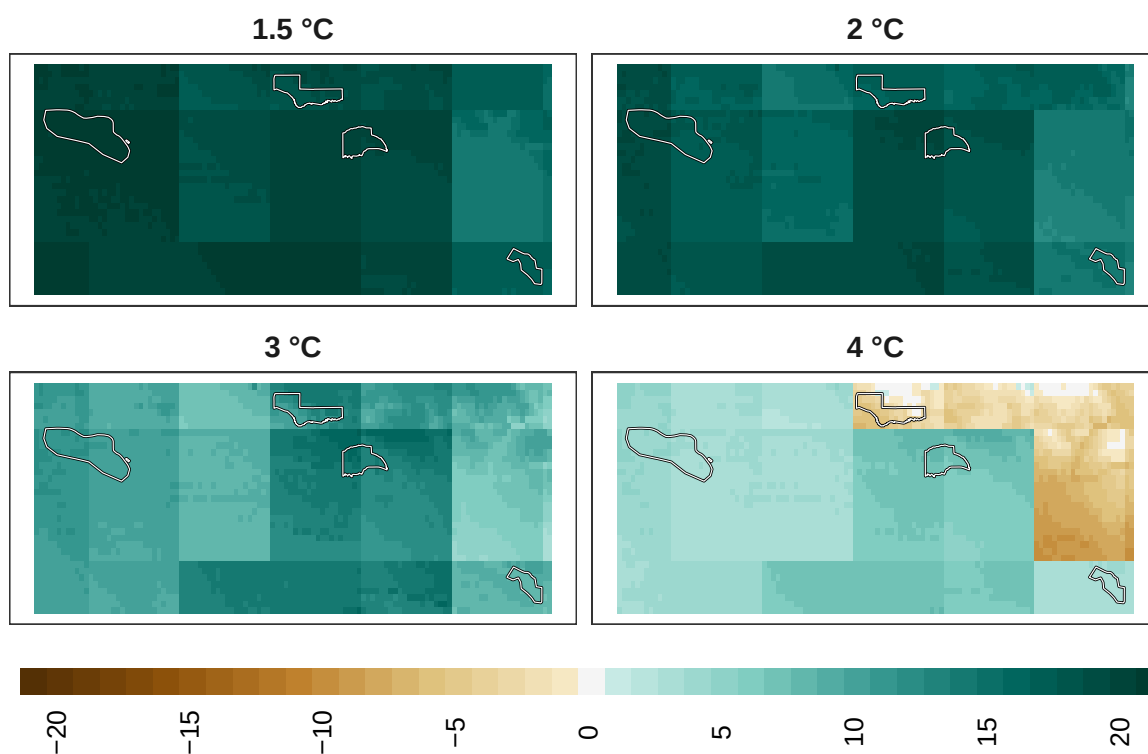
Figure 22: Adaptation effort for pollinators at 1 km resolution.
