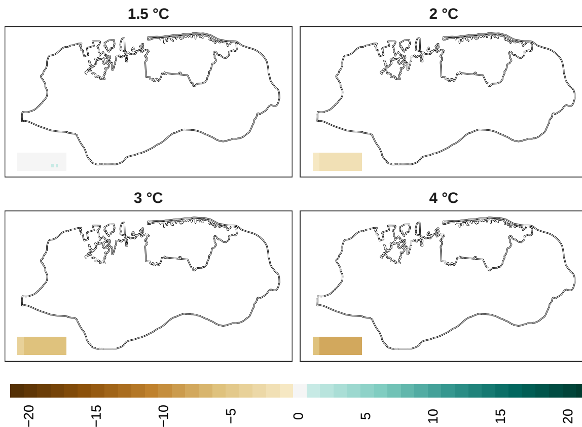
Figure 20: Adaptation effort for reptiles at 1 km resolution.
