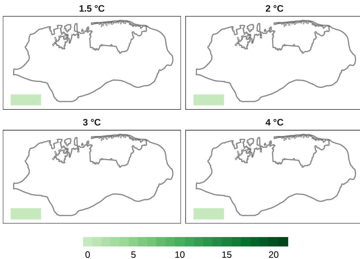
Figure 13: Number of models in agreement for reptile refugia at 1 km resolution.
