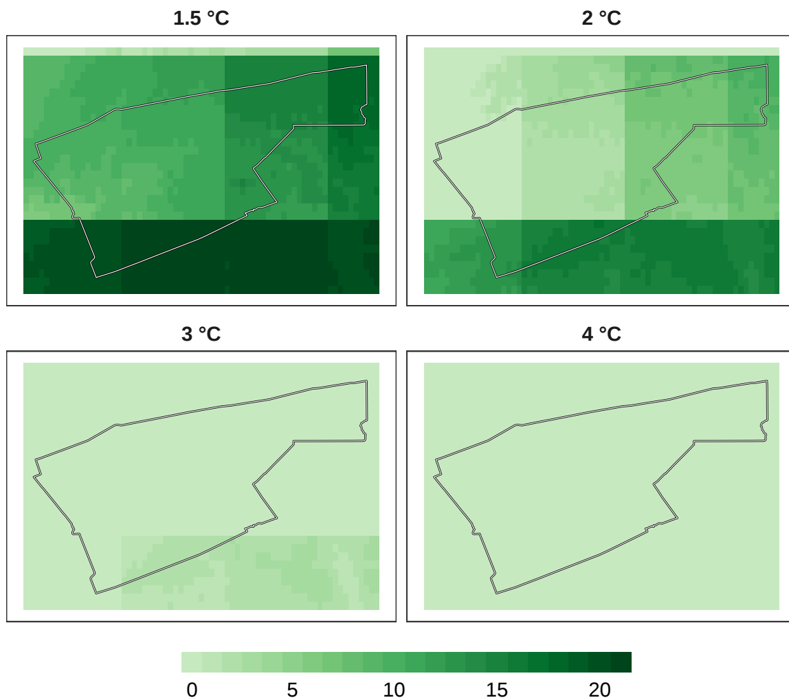
Figure 12: Number of models in agreement for reptile refugia at 1 km resolution.
