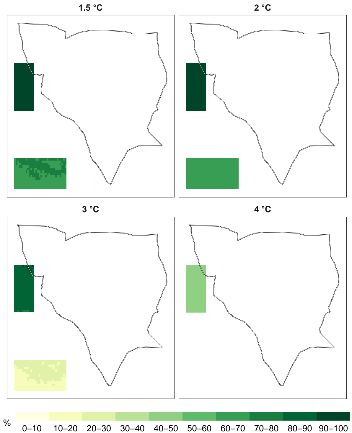
Figure 7: Percent timber species remaining at 1 km resolution.
