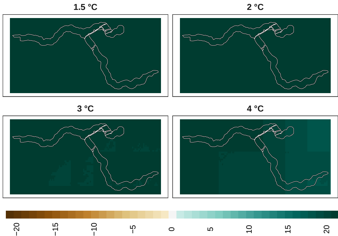
Figure 14: Adaptation effort for birds at 1 km resolution.
