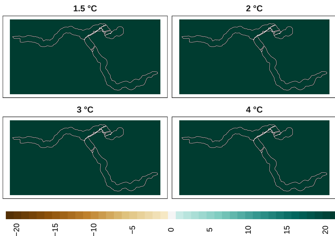
Figure 13: Adaptation effort for plants at 1 km resolution.
