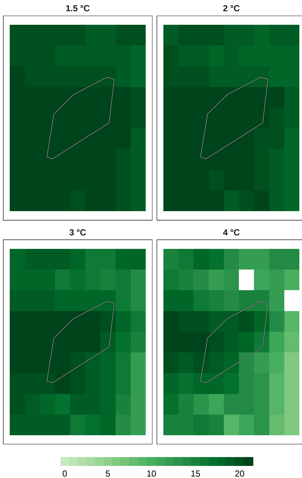
Figure 11: Number of models in agreement for insect refugia at 1 km resolution.
