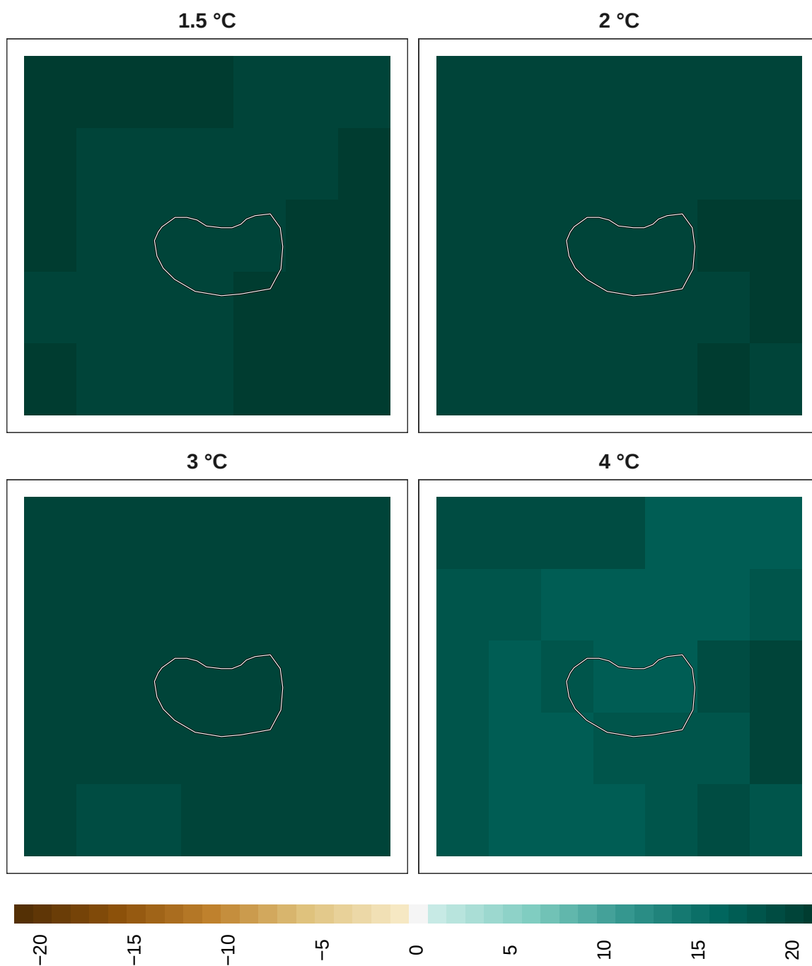
Figure 14: Adaptation effort for birds at 1 km resolution.
