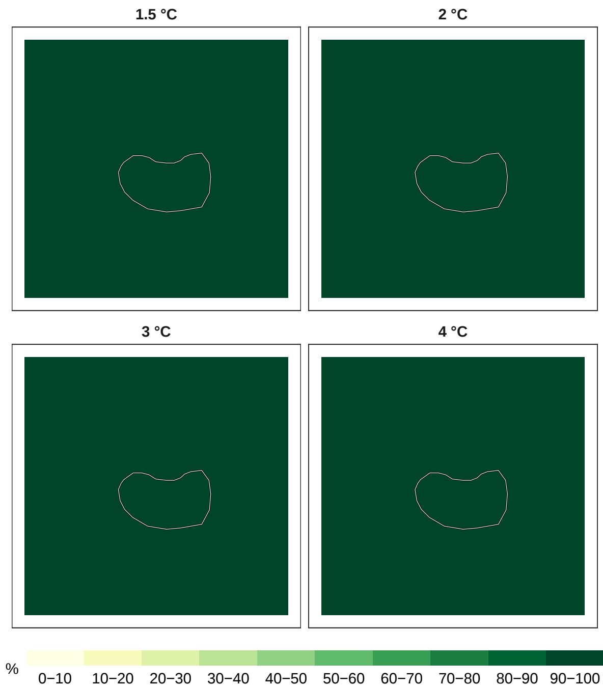
Figure 6: Percent timber species remaining at 1 km resolution.
