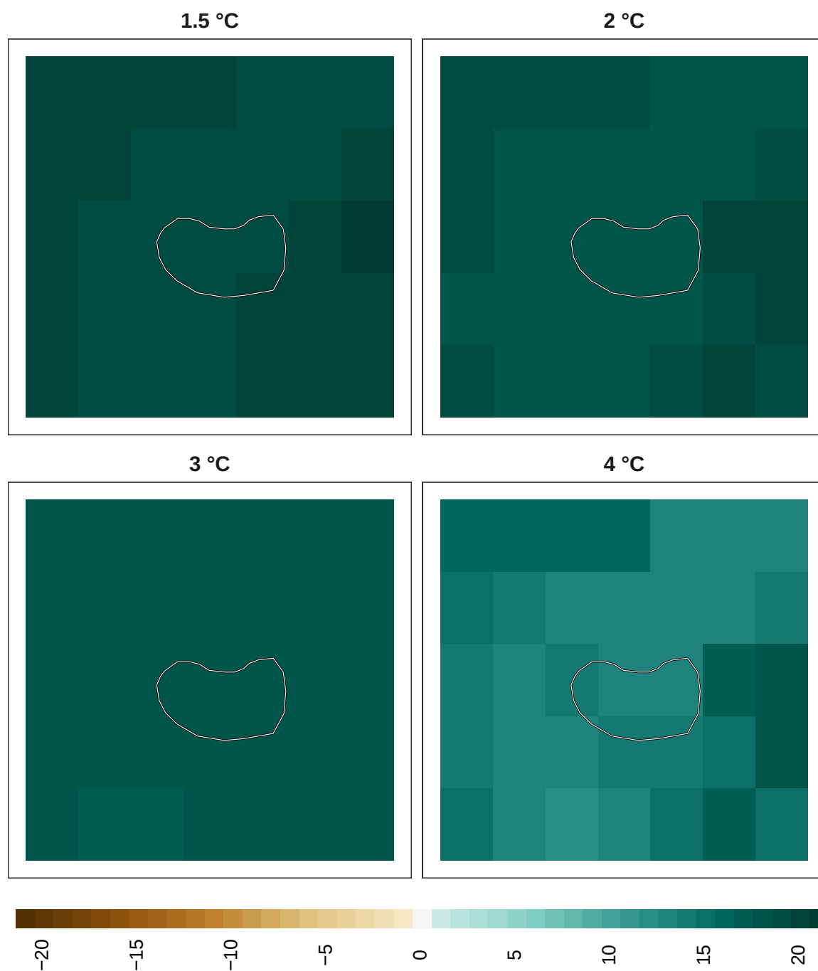
Figure 13: Adaptation effort for plants at 1 km resolution.
