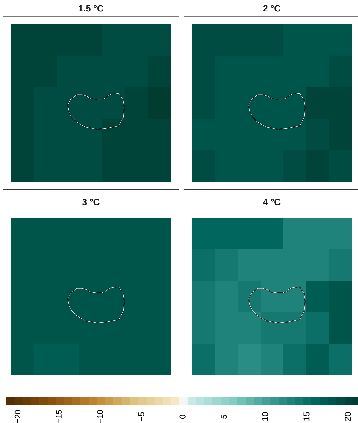
Figure 12: Adaptation effort for overall biodiversity at 1 km resolution.
