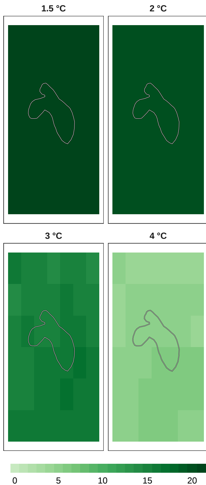
Figure 4: Number of models in agreement for plant refugia at 1 km resolution.
