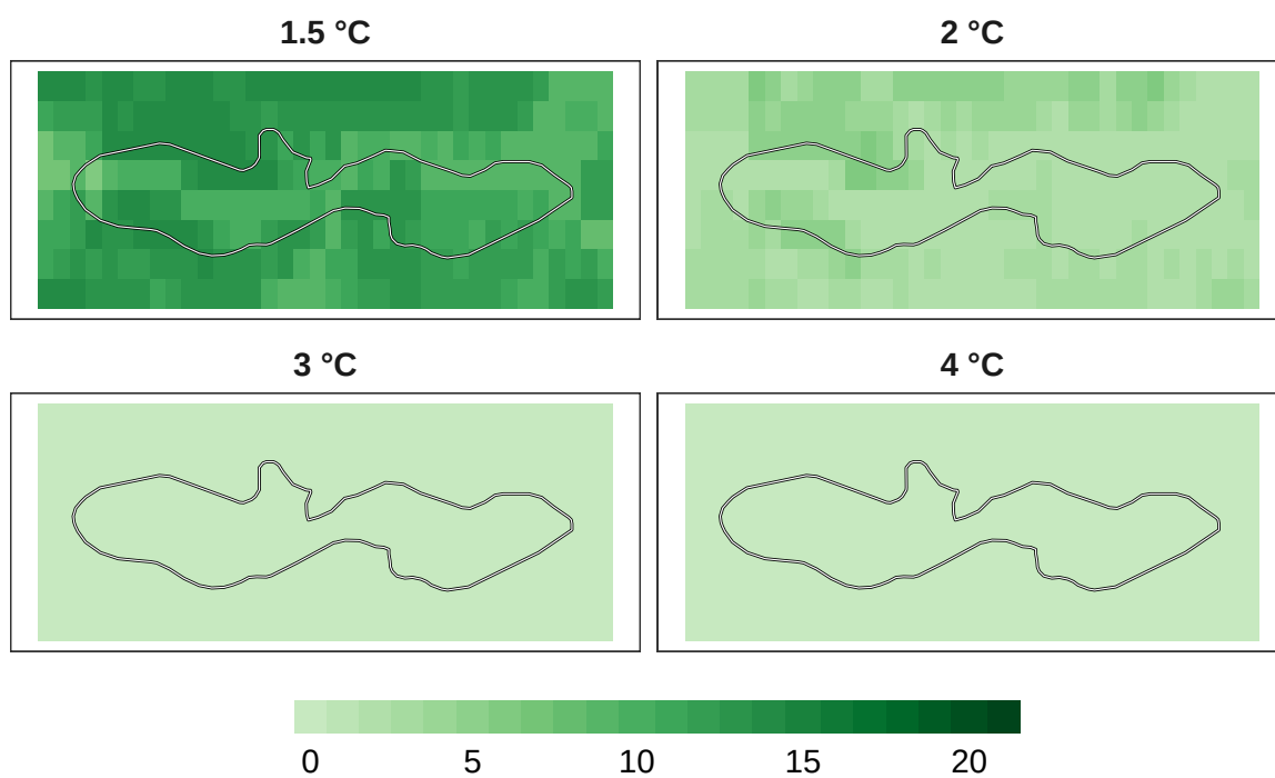
Figure 13: Number of models in agreement for pollinator refugia at 1 km resolution.
