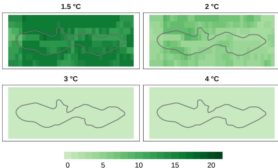
Figure 9: Number of models in agreement for plant refugia at 1 km resolution.
