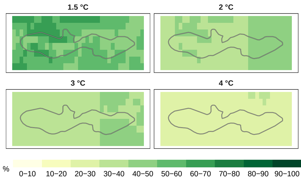
Figure 7: Percent timber species remaining at 1 km resolution.
