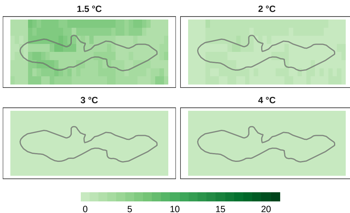
Figure 12: Number of models in agreement for insect refugia at 1 km resolution.
