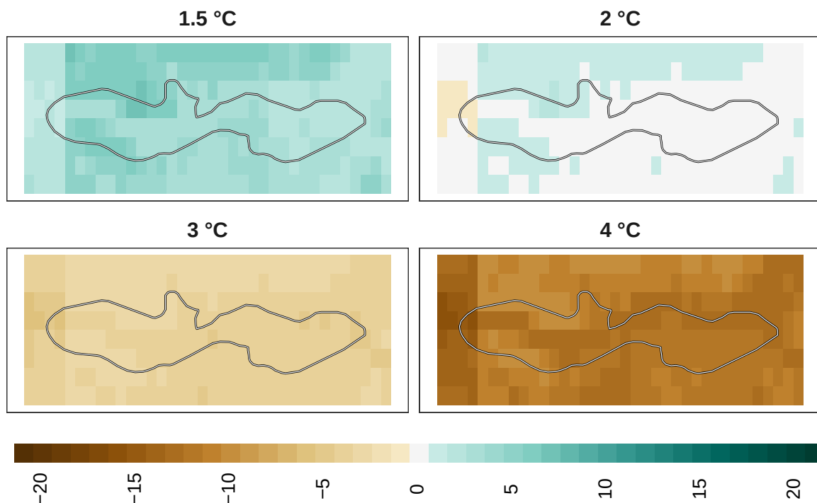
Figure 18: Adaptation effort for insects at 1 km resolution.
