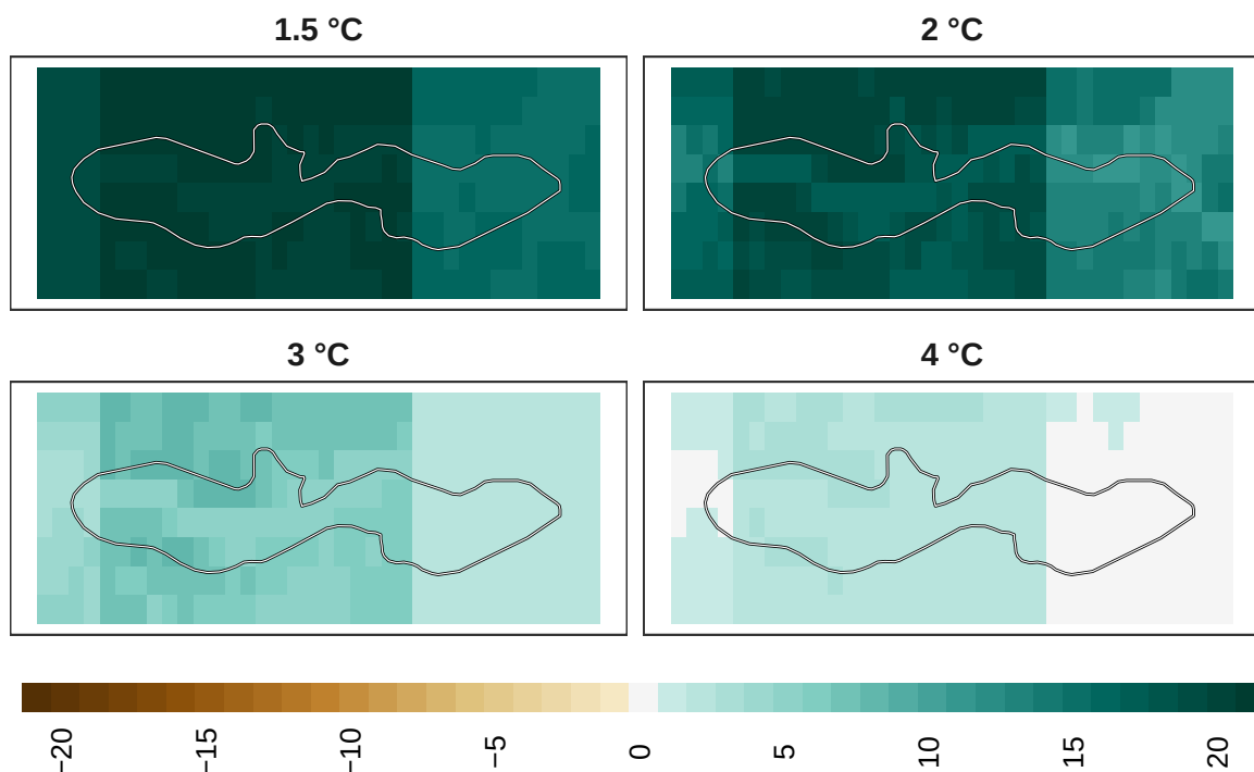
Figure 17: Adaptation effort for mammals at 1 km resolution.
