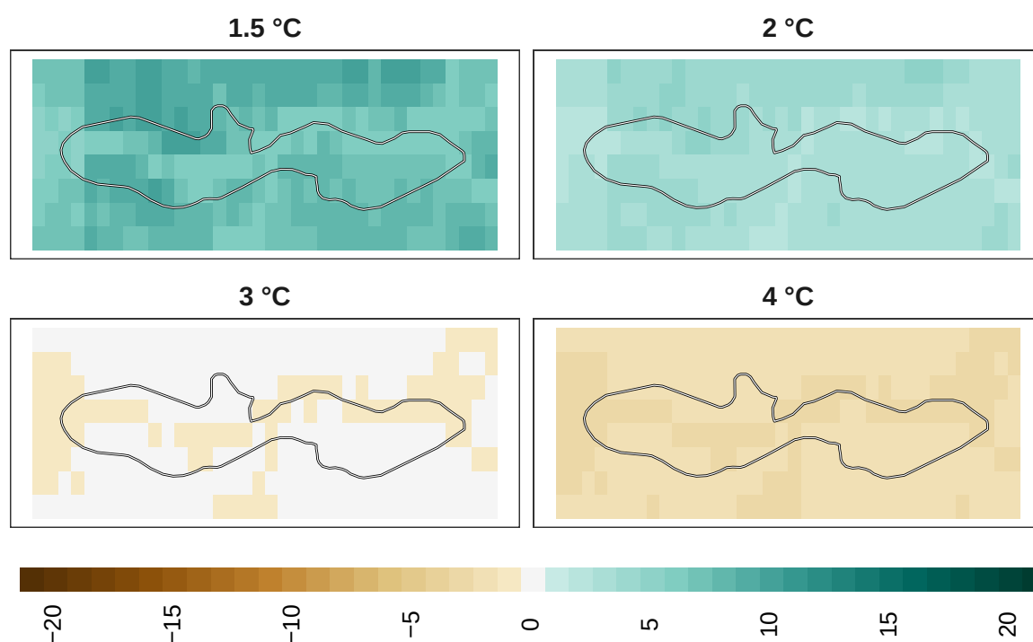
Figure 14: Adaptation effort for overall biodiversity at 1 km resolution.
