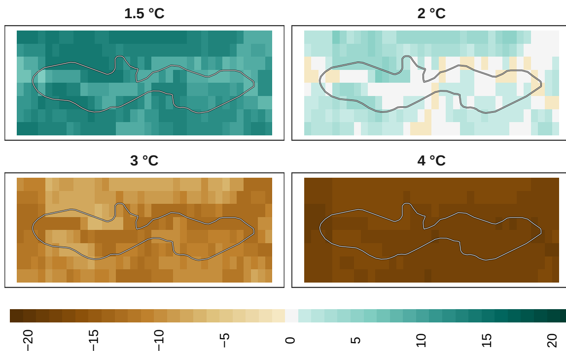
Figure 19: Adaptation effort for pollinators at 1 km resolution.
