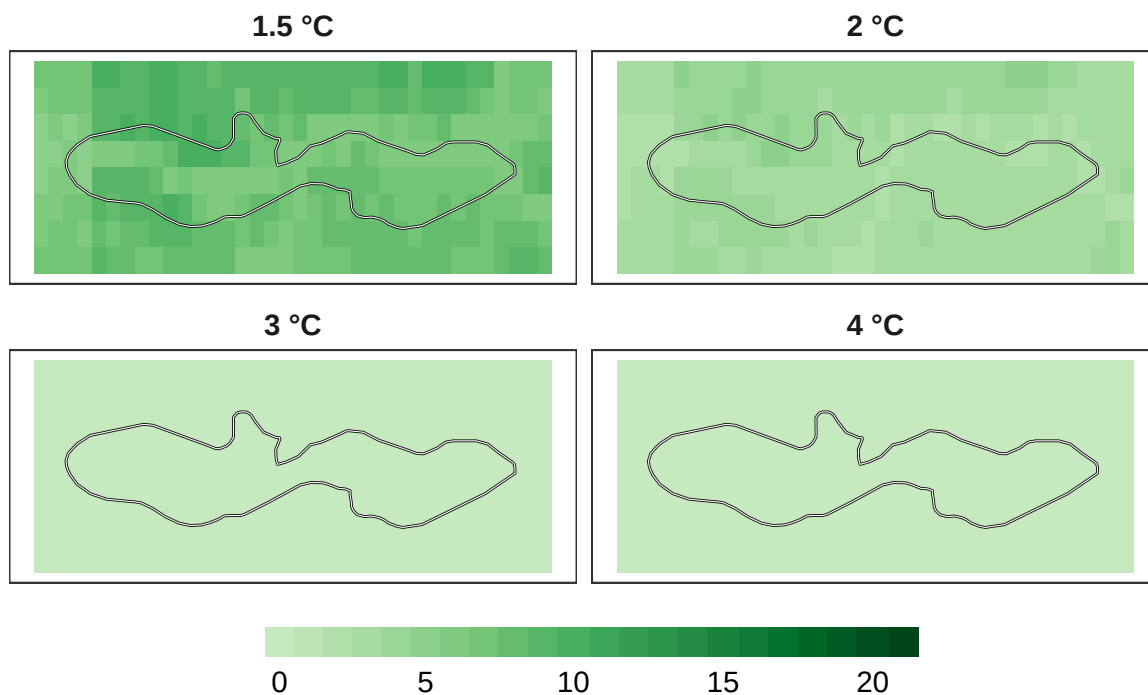
Figure 8: Number of models in agreement for overall biodiversity refugia at 1 km resolution.
