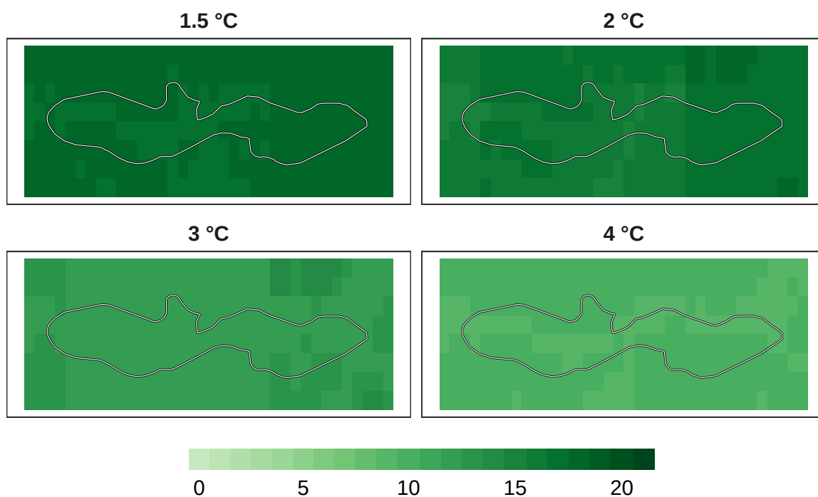
Figure 10: Number of models in agreement for bird refugia.
