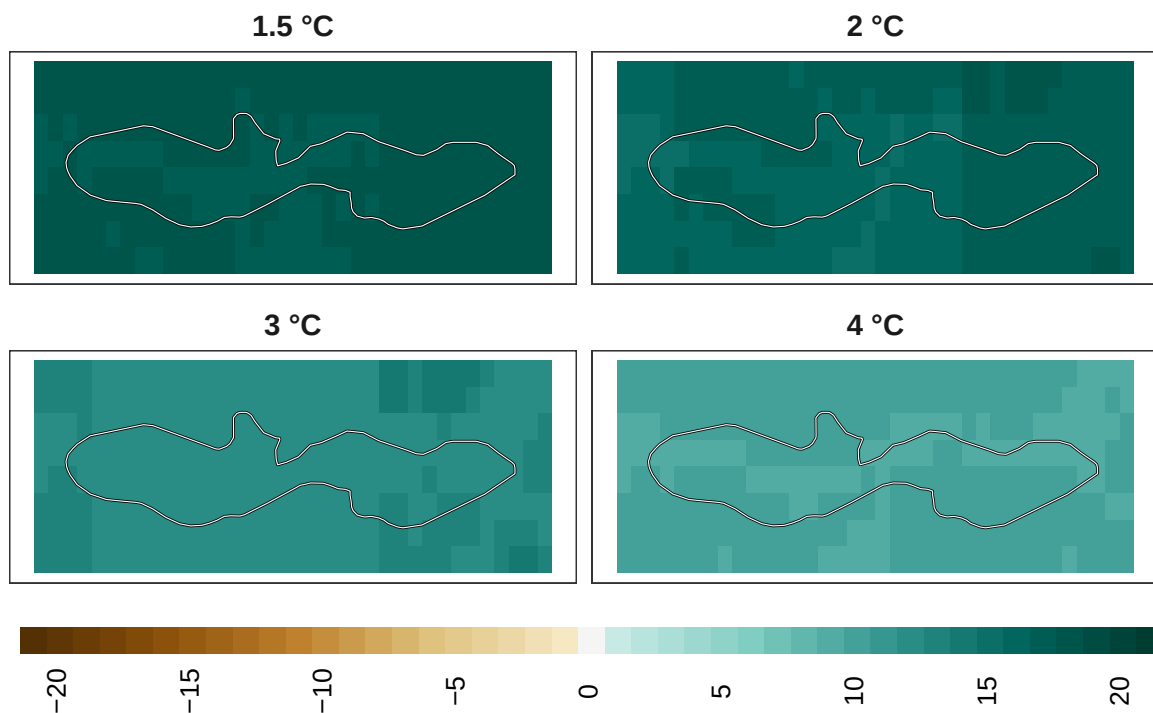
Figure 16: Adaptation effort for birds at 1 km resolution.
