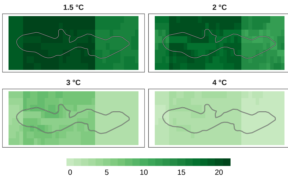
Figure 11: Number of models in agreement for mammal refugia at 1 km resolution.
