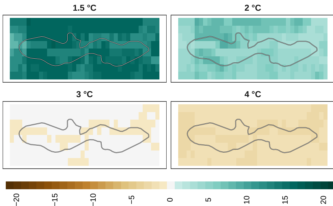
Figure 15: Adaptation effort for plants at 1 km resolution.
