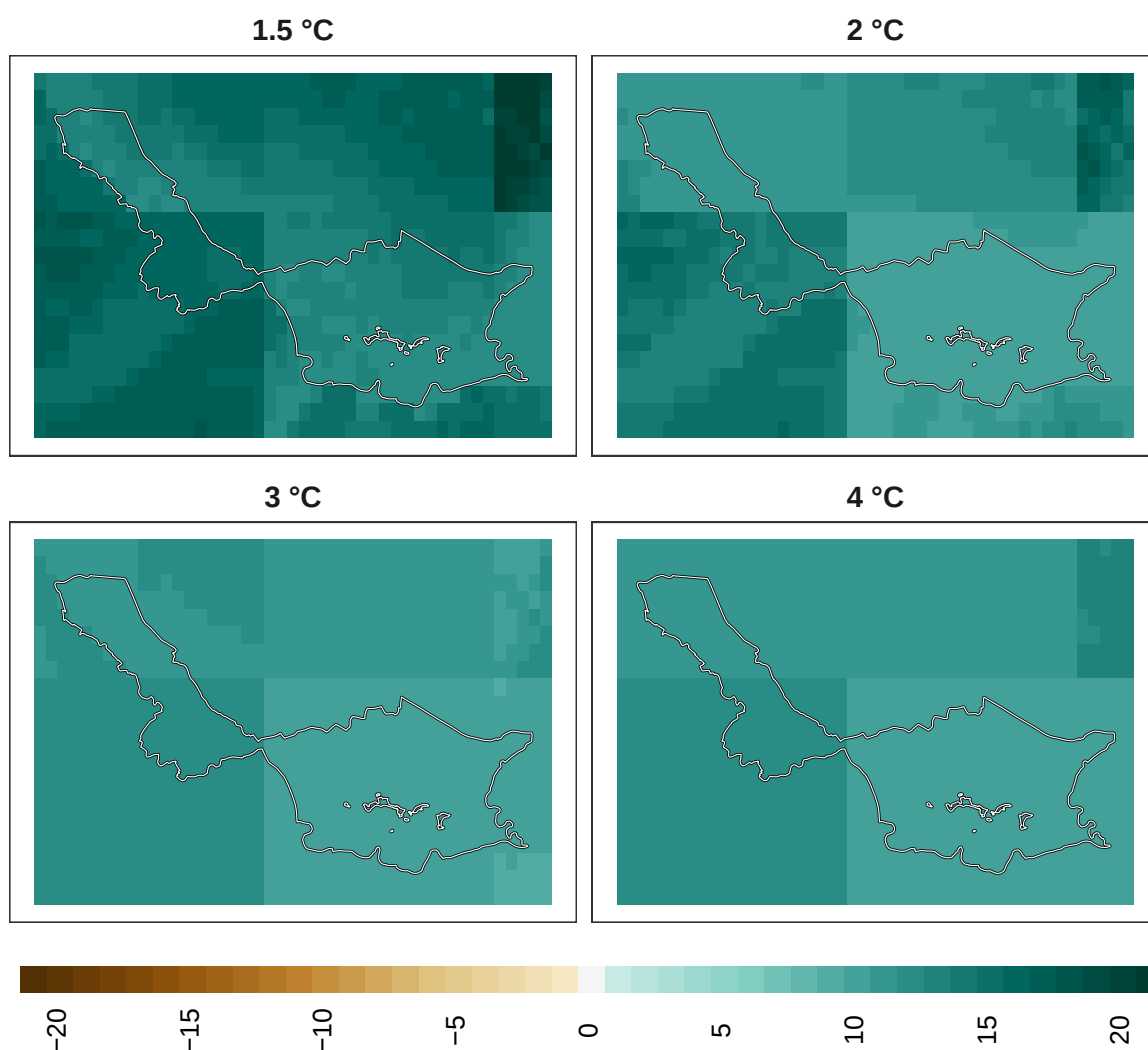
Figure 19: Adaptation effort for mammals at 1 km resolution.
