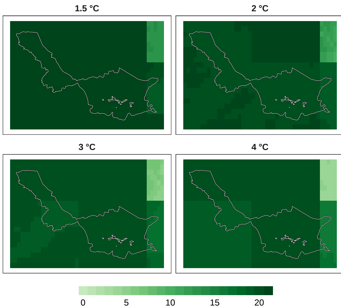
Figure 13: Number of models in agreement for reptile refugia at 1 km resolution.
