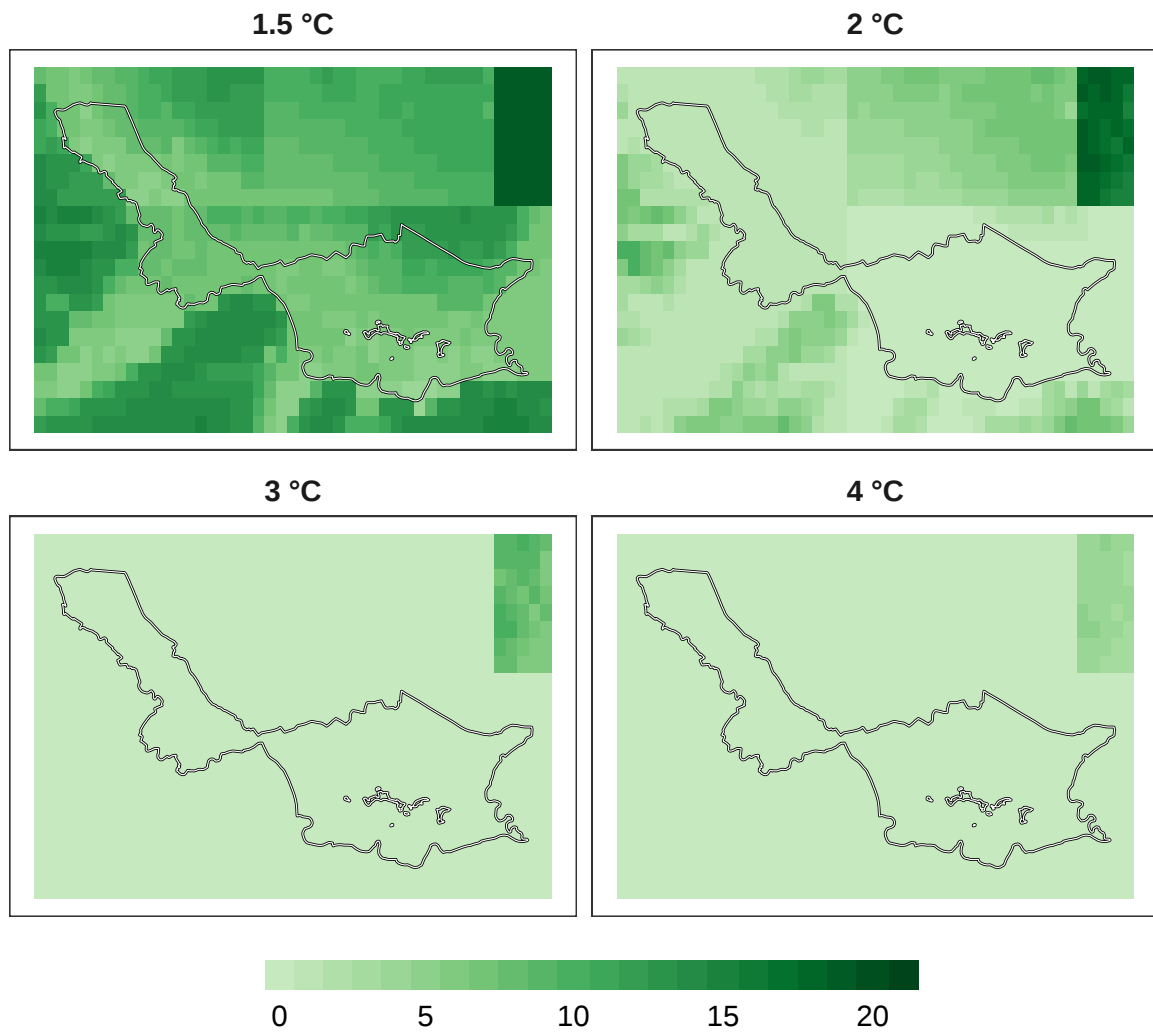
Figure 15: Number of models in agreement for pollinator refugia at 1 km resolution.
