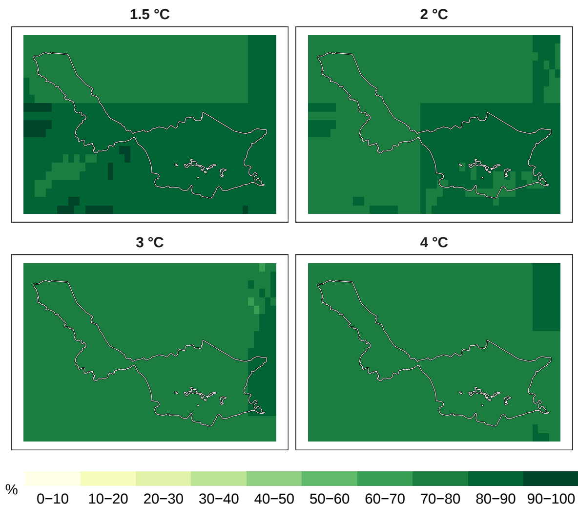
Figure 4: Percent mammals remaining at 1 km resolution.
