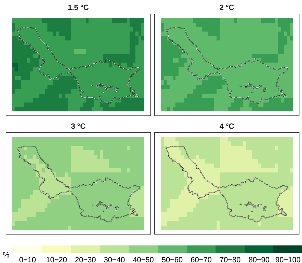
Figure 6: Percent insects remaining at 1 km resolution.
