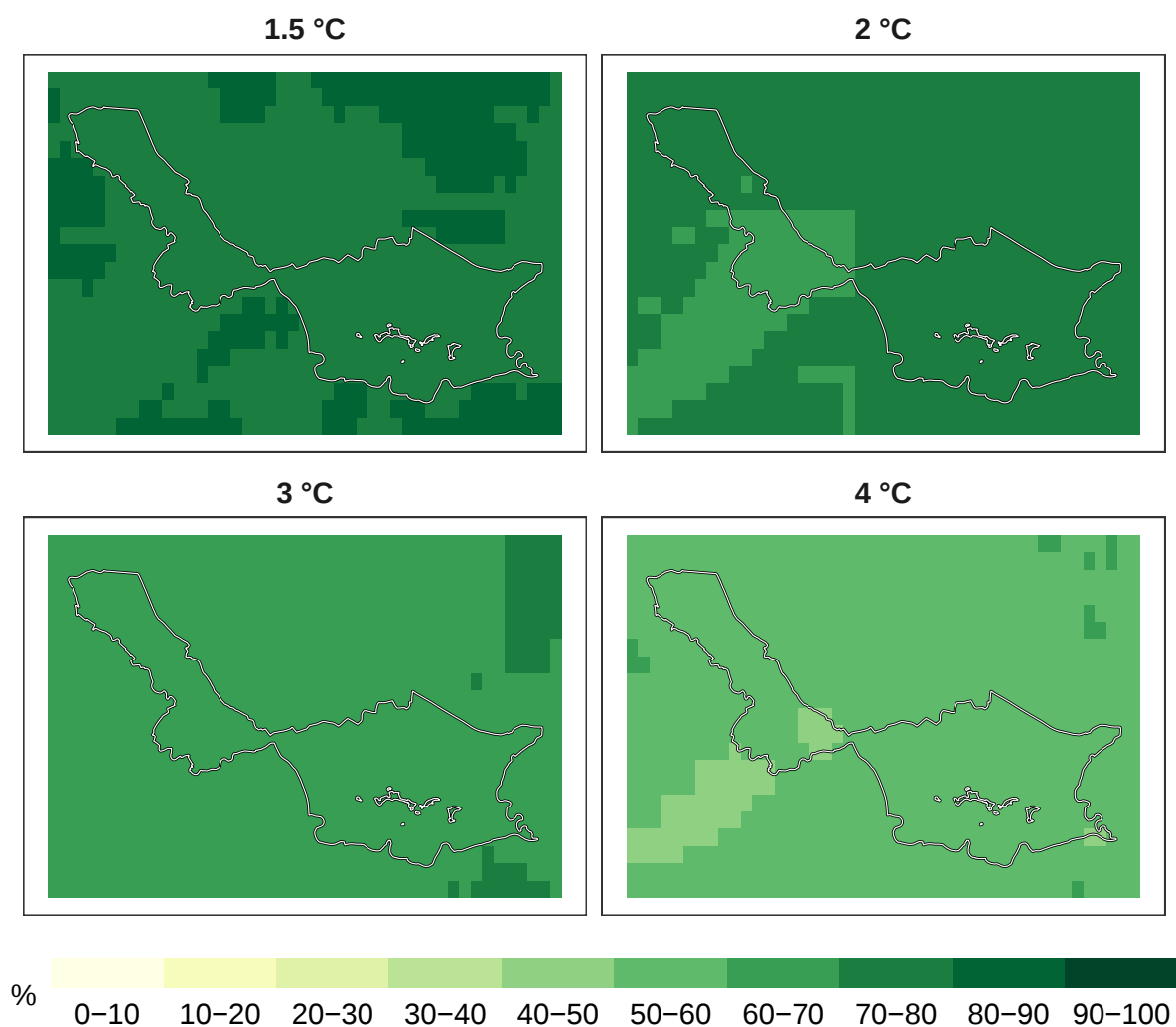
Figure 3: Percent birds remaining at 1 km resolution.
