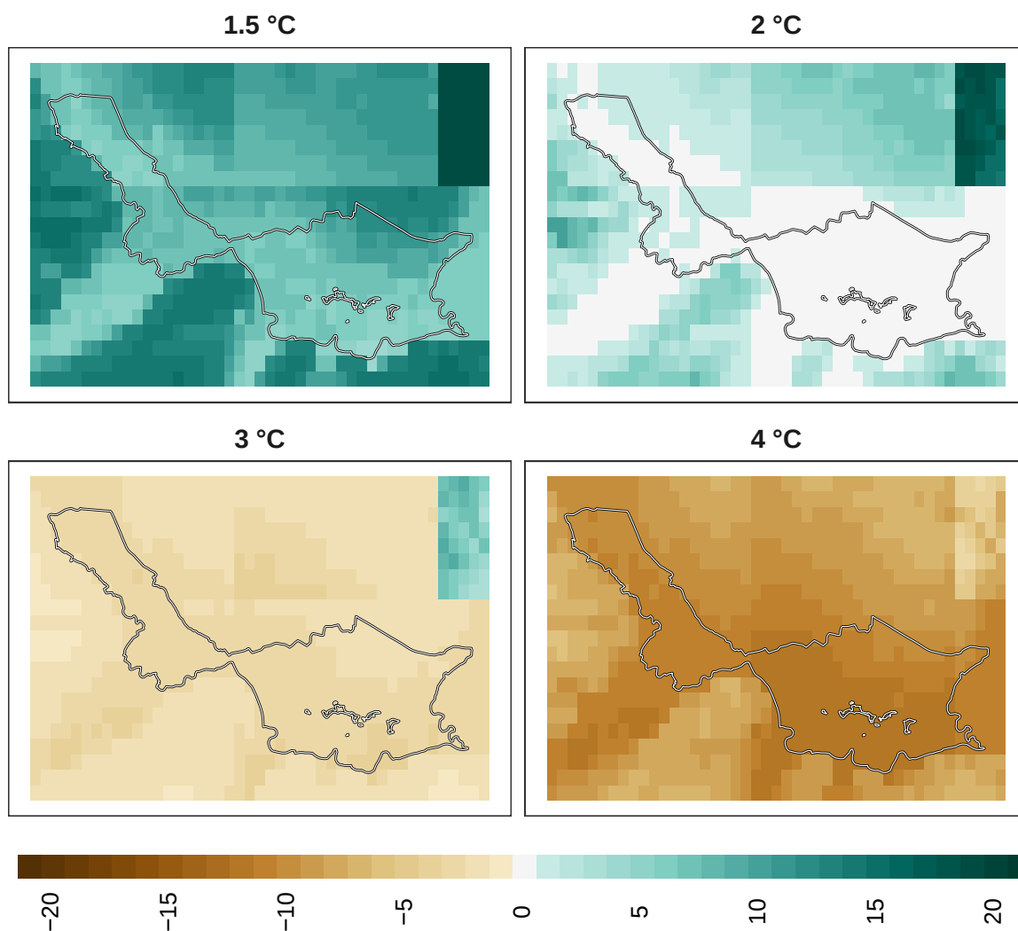
Figure 22: Adaptation effort for pollinators at 1 km resolution.
