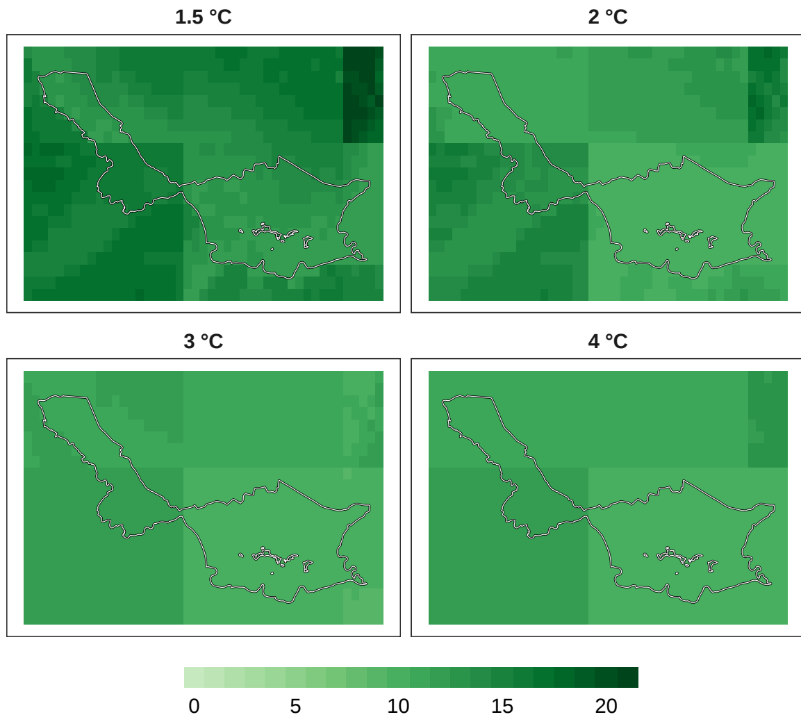
Figure 12: Number of models in agreement for mammal refugia at 1 km resolution.
