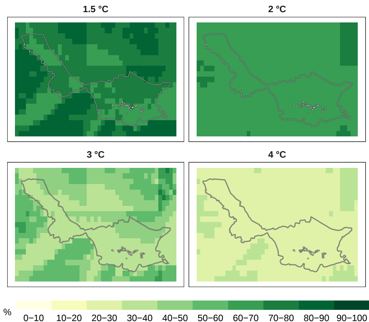
Figure 7: Percent pollinators remaining at 1 km resolution.
