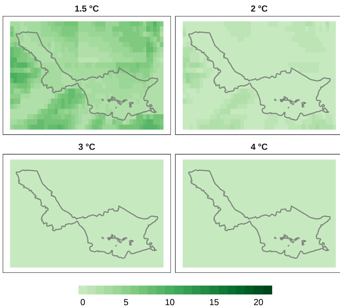
Figure 14: Number of models in agreement for insect refugia at 1 km resolution.
