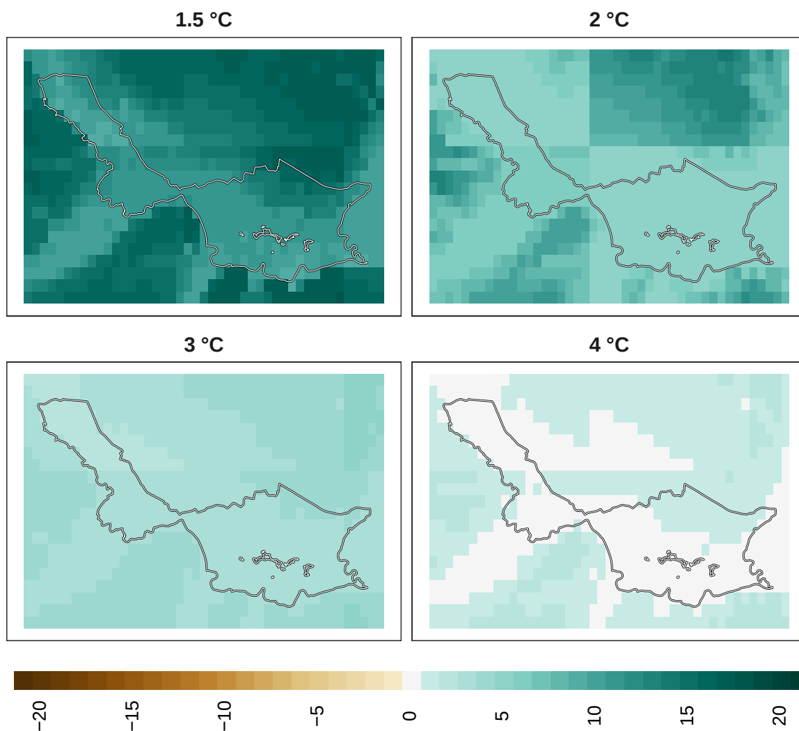
Figure 18: Adaptation effort for birds at 1 km resolution.
