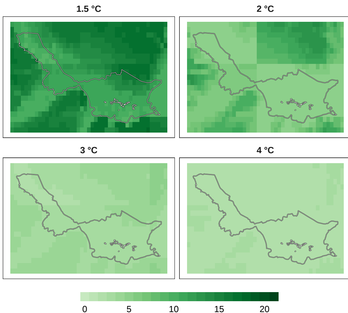
Figure 11: Number of models in agreement for bird refugia.
