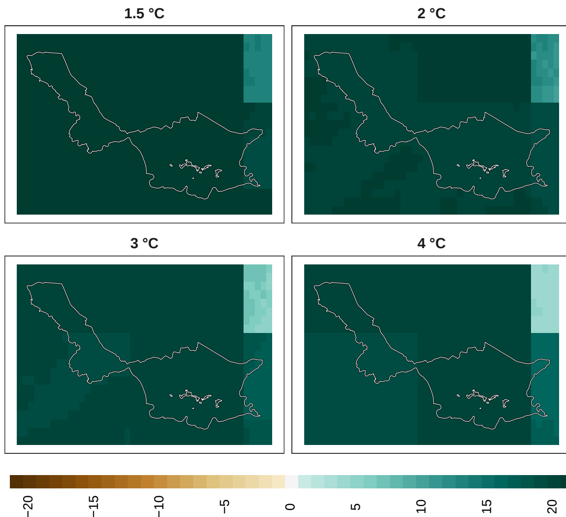
Figure 20: Adaptation effort for reptiles at 1 km resolution.
