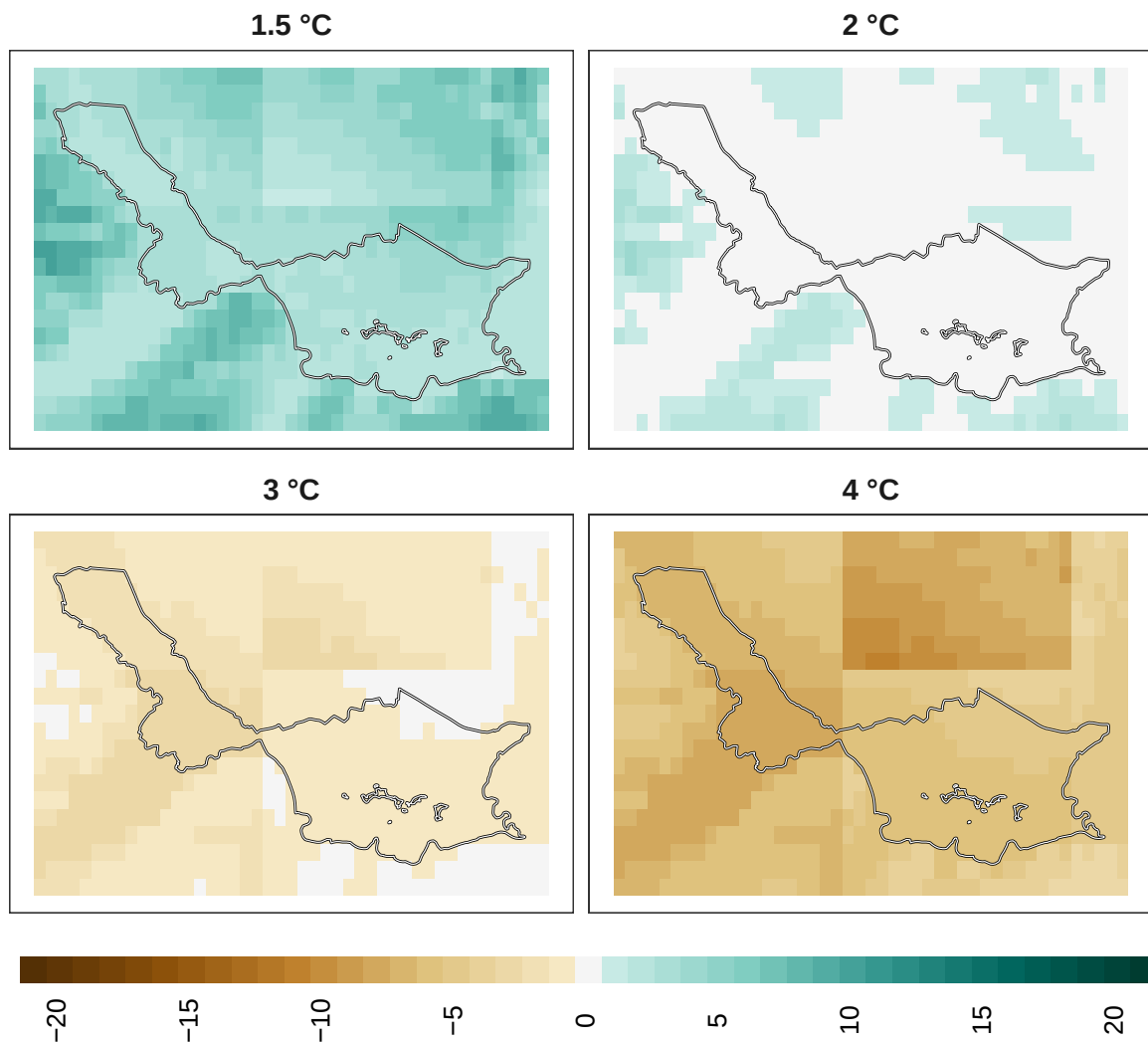
Figure 21: Adaptation effort for insects at 1 km resolution.
