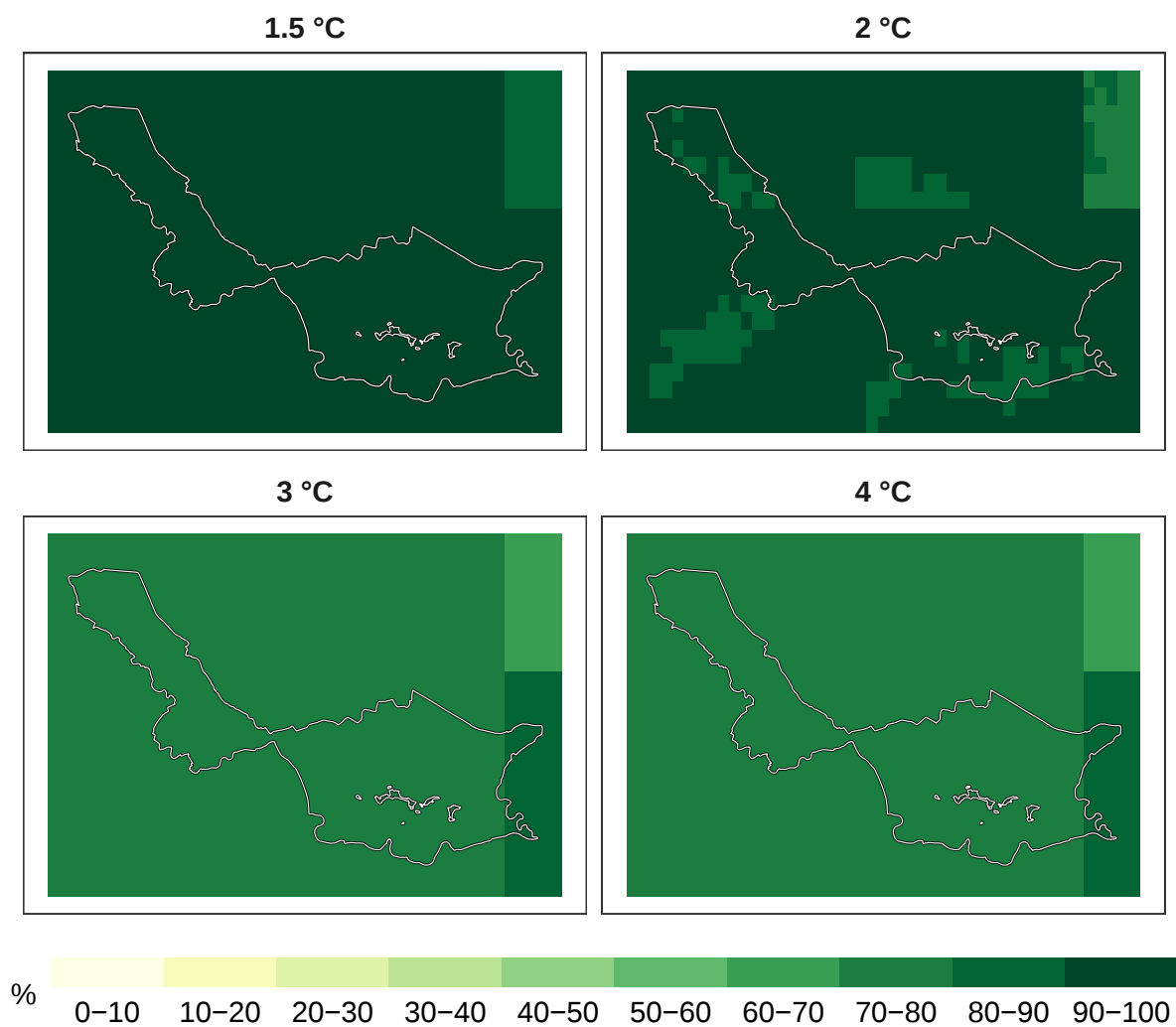
Figure 5: Percent reptiles remaining at 1 km resolution.
