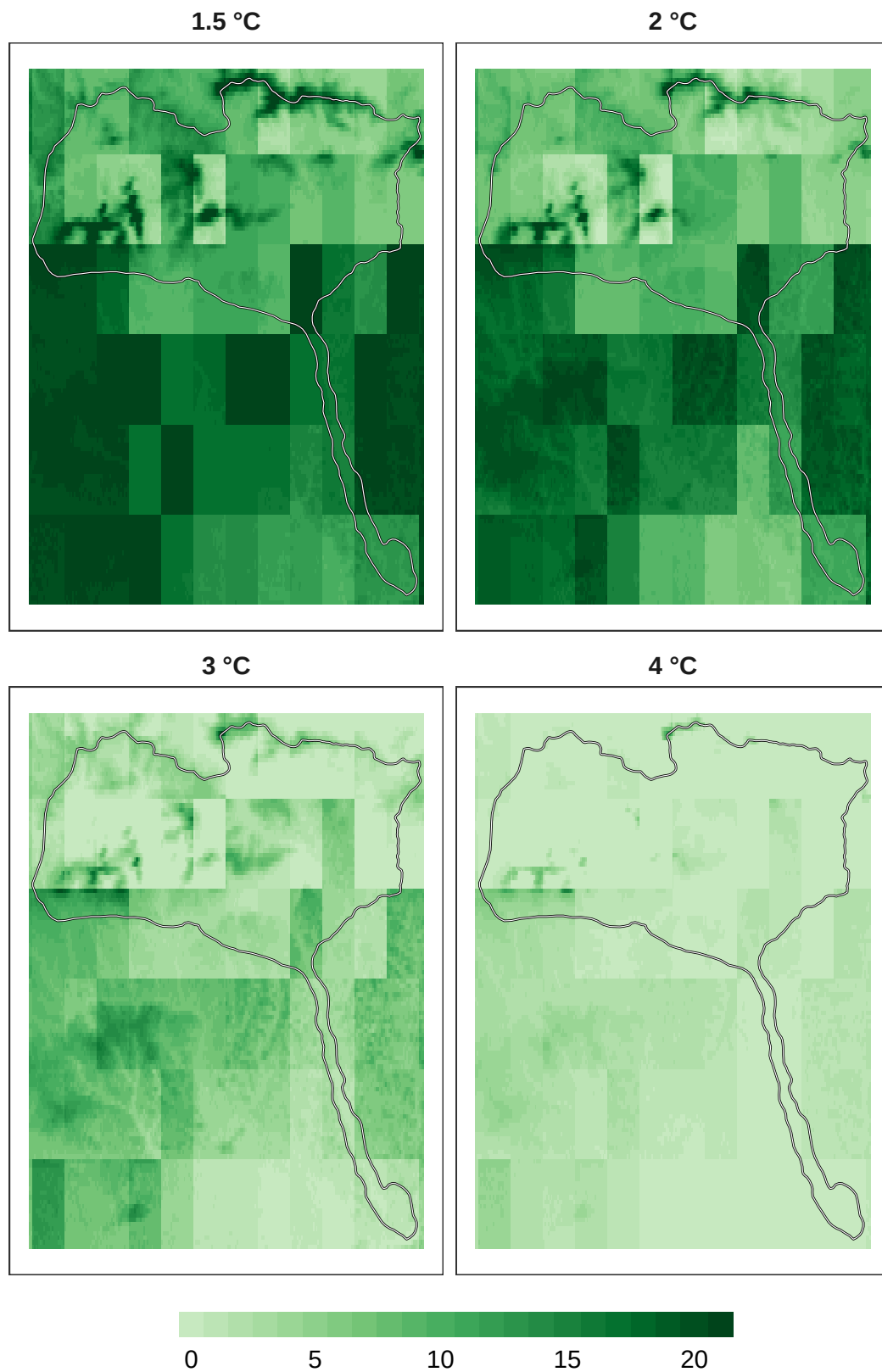
Figure 5: Number of models in agreement for plant refugia at 1 km resolution.
