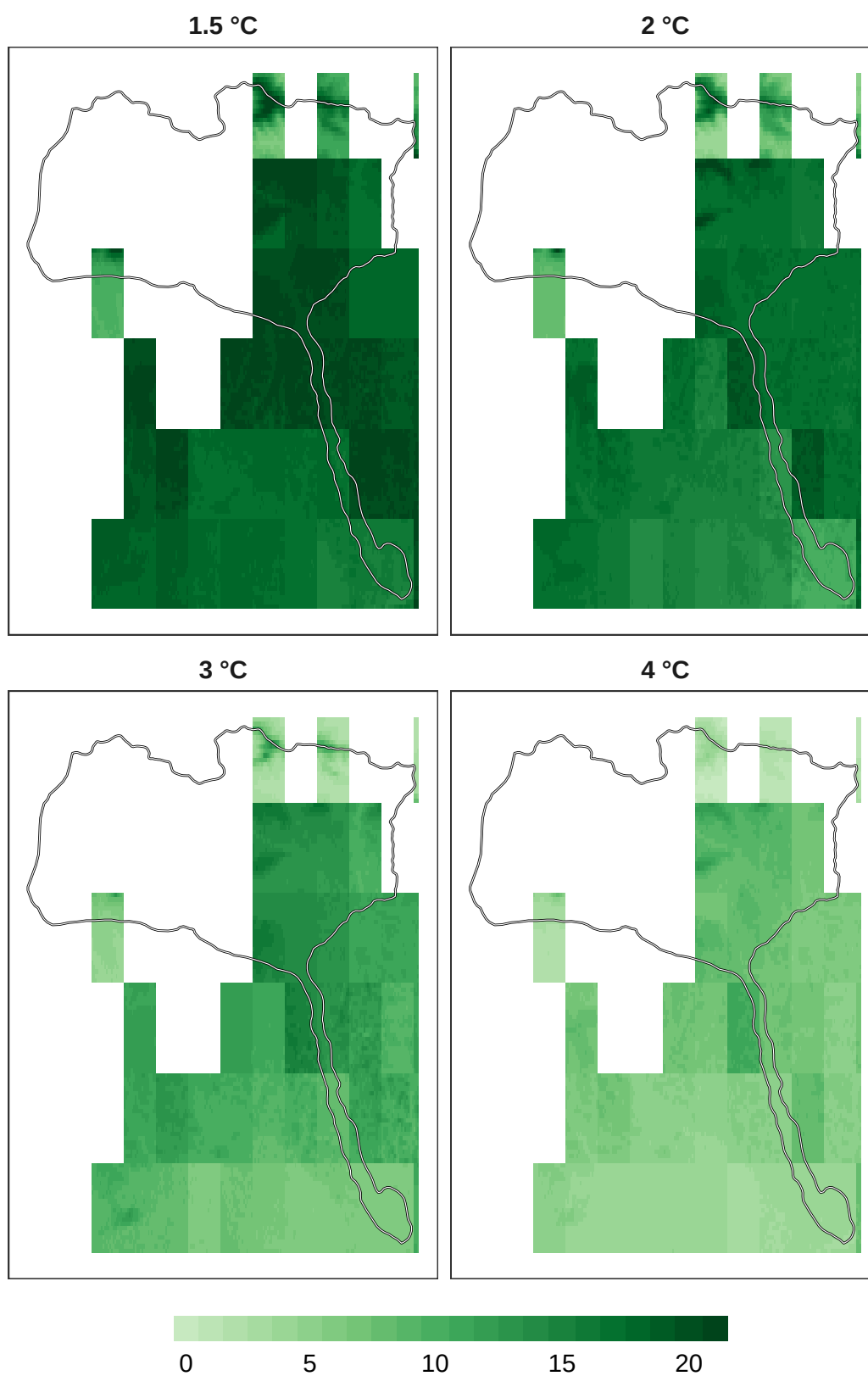
Figure 6: Number of models in agreement for mammal refugia at 1 km resolution.
