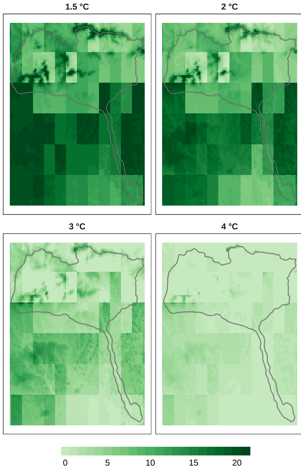
Figure 4: Number of models in agreement for overall biodiversity refugia at 1 km resolution.
