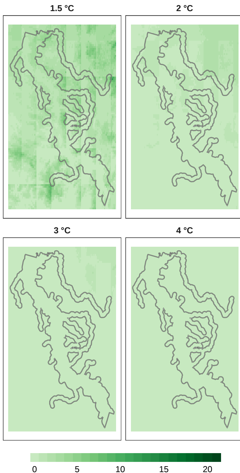
Figure 5: Number of models in agreement for overall biodiversity refugia at 1 km resolution.
