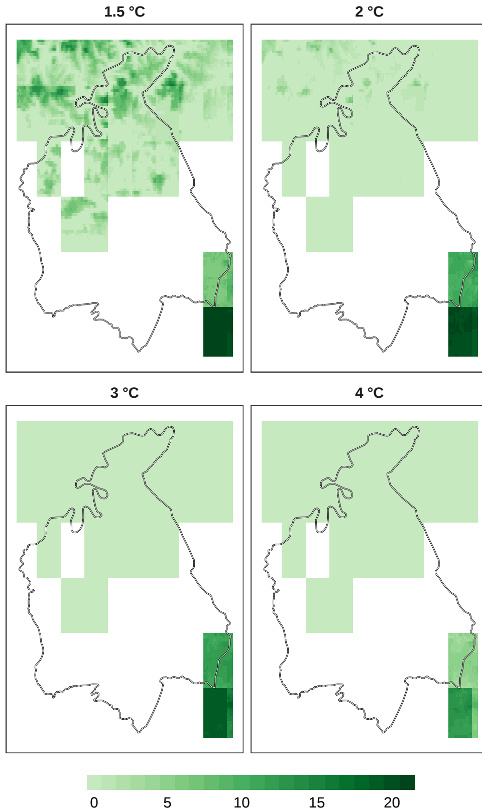
Figure 3: Number of models in agreement for overall biodiversity refugia at 1 km resolution.
