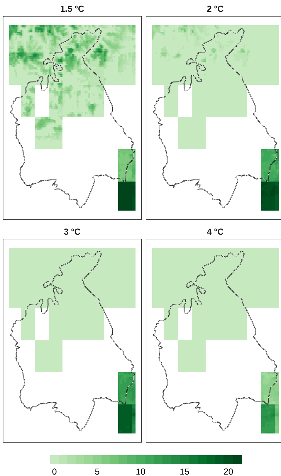
Figure 4: Number of models in agreement for mammal refugia at 1 km resolution.
