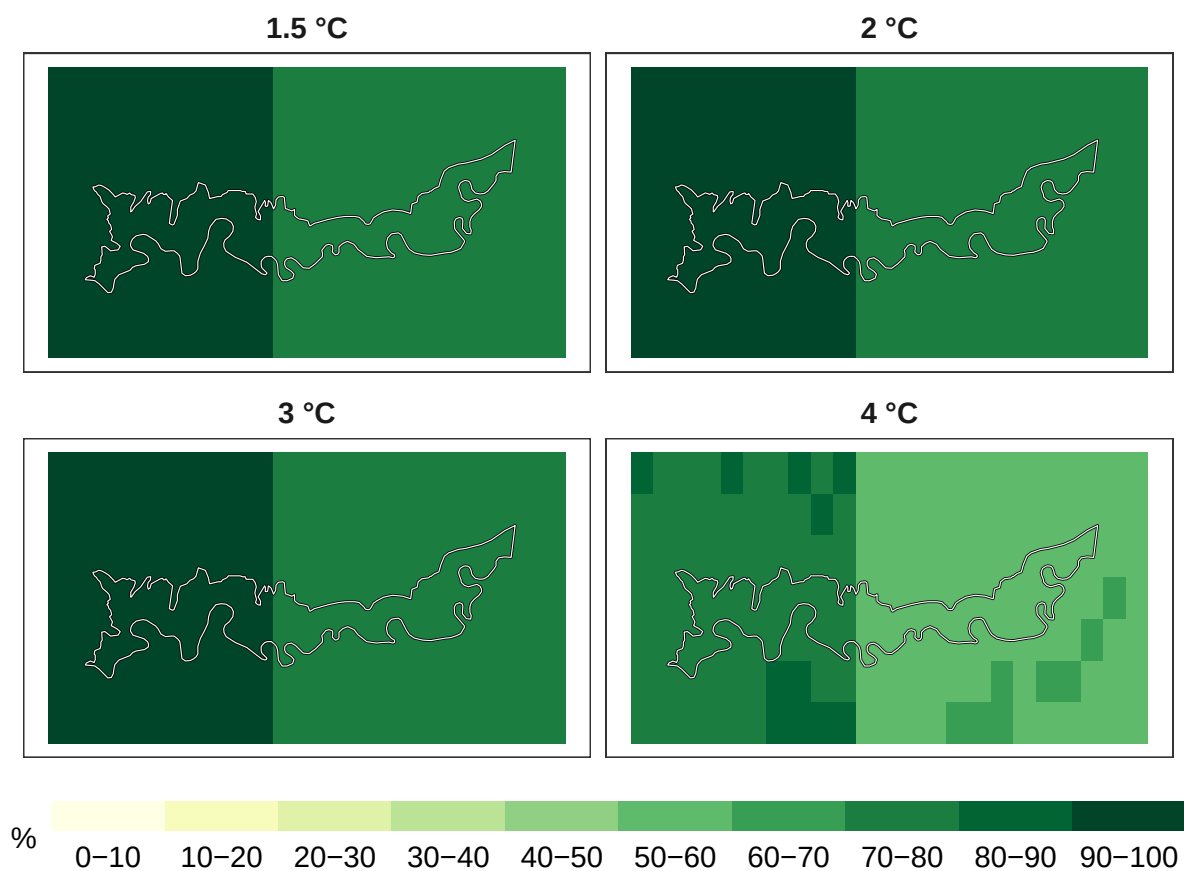
Figure 6: Percent timber species remaining at 1 km resolution.
