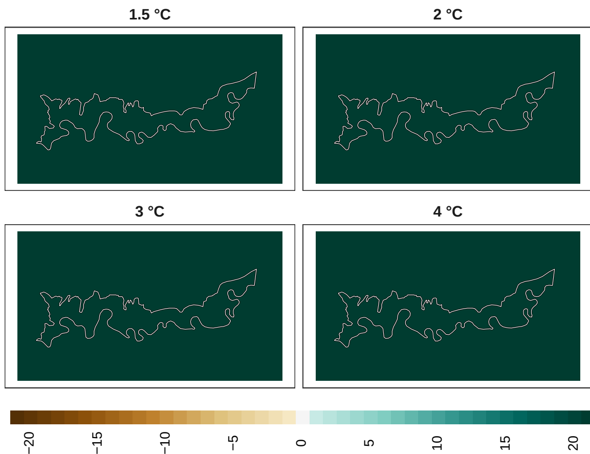
Figure 14: Adaptation effort for birds at 1 km resolution.
