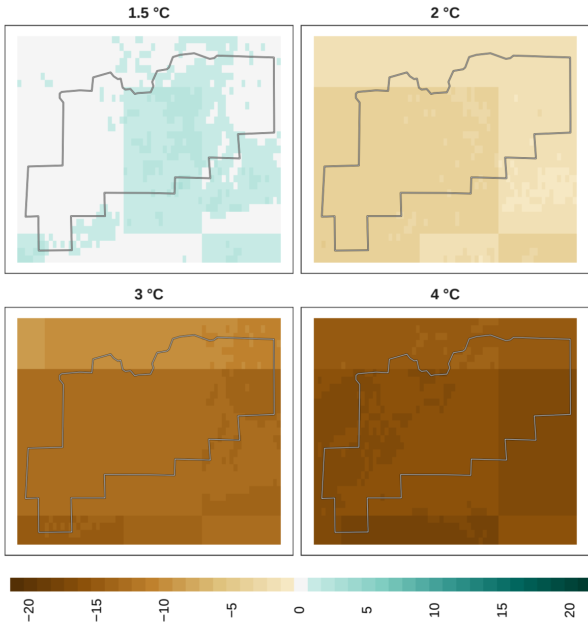
Figure 12: Adaptation effort for plants at 1 km resolution.
