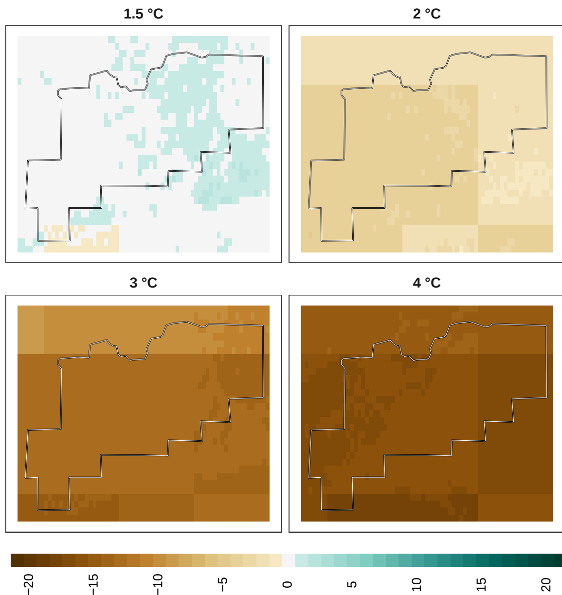
Figure 11: Adaptation effort for overall biodiversity at 1 km resolution.
