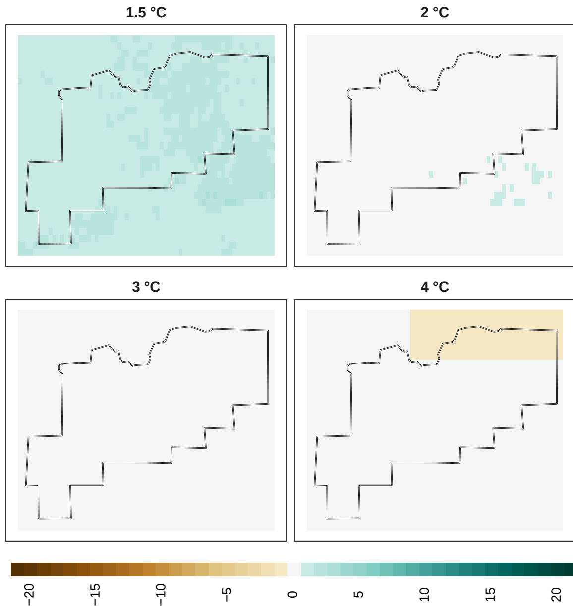
Figure 14: Adaptation effort for mammals at 1 km resolution.
