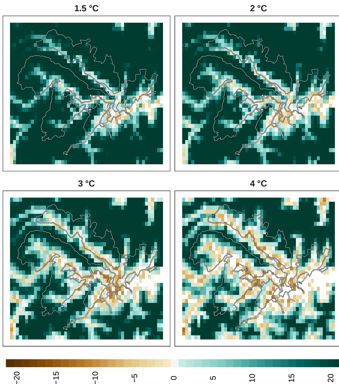
Figure 17: Adaptation effort for plants at 1 km resolution.
