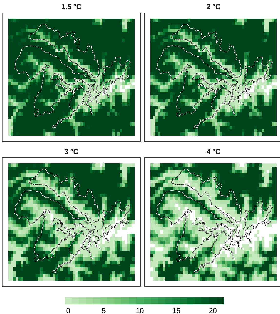
Figure 9: Number of models in agreement for overall biodiversity refugia at 1 km resolution.
