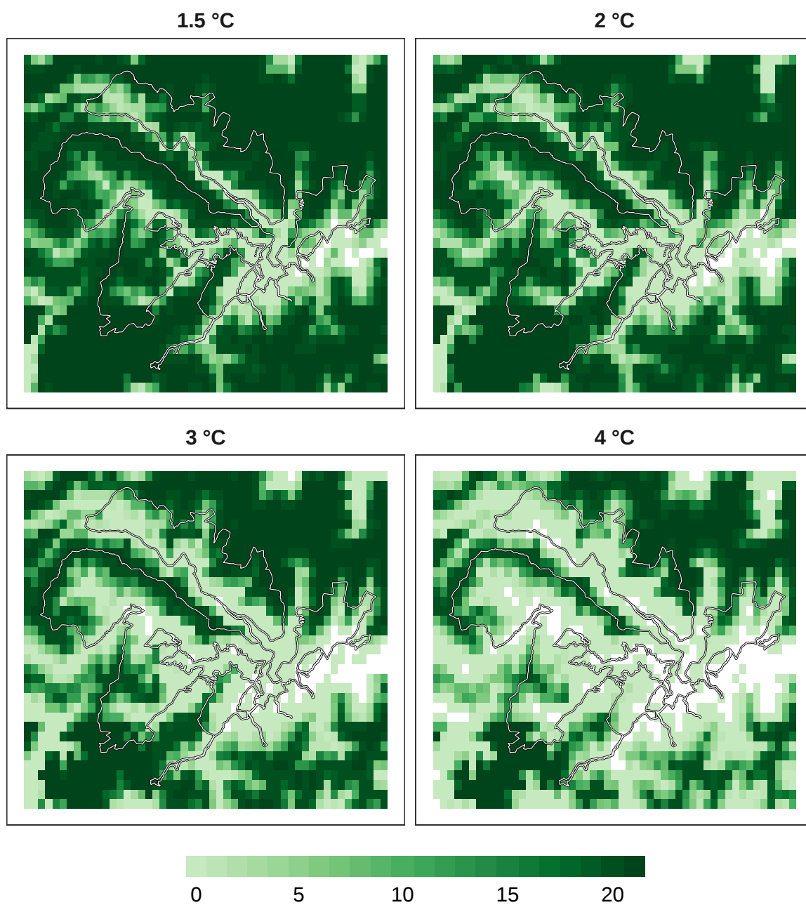
Figure 12: Number of models in agreement for mammal refugia at 1 km resolution.
