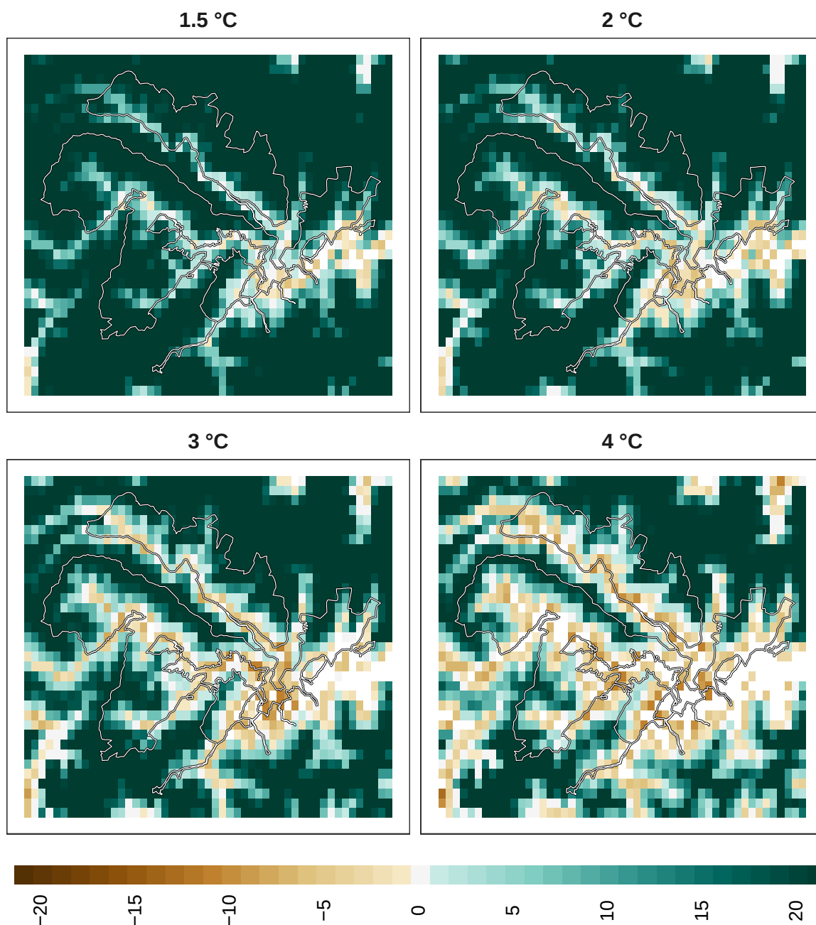
Figure 16: Adaptation effort for overall biodiversity at 1 km resolution.
