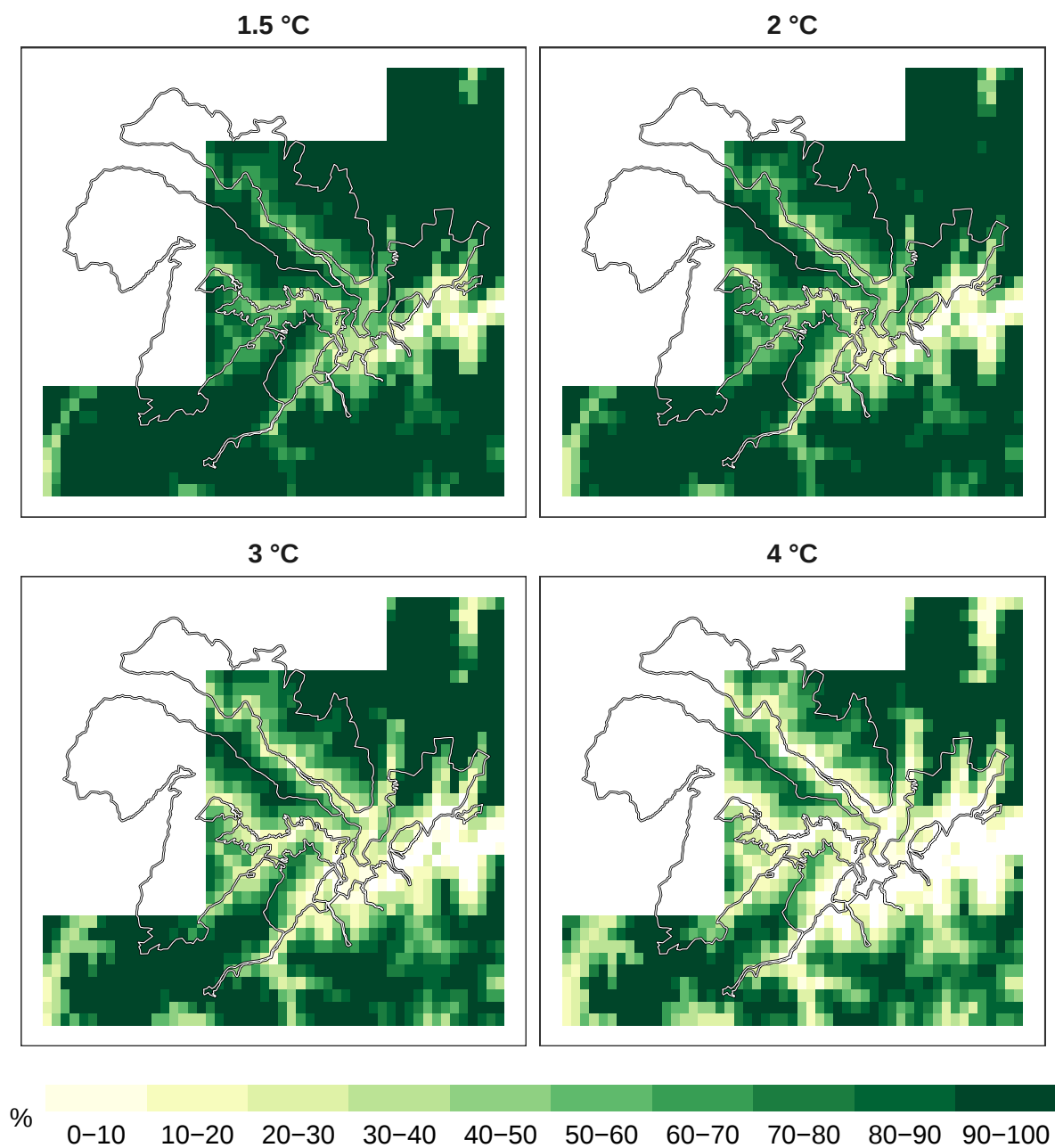
Figure 8: Percent timber species remaining at 1 km resolution.
