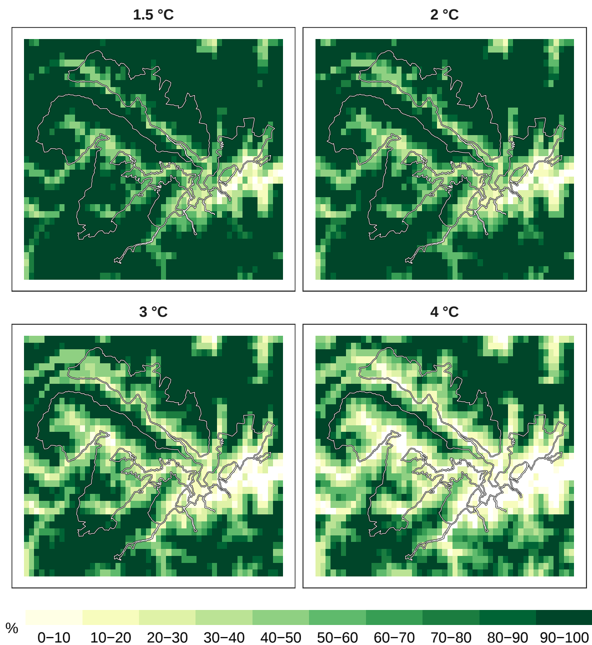
Figure 7: Percent pollinators remaining at 1 km resolution.
