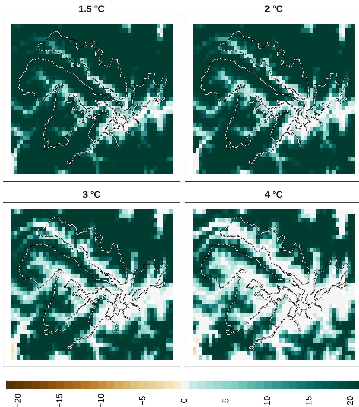
Figure 18: Adaptation effort for birds at 1 km resolution.
