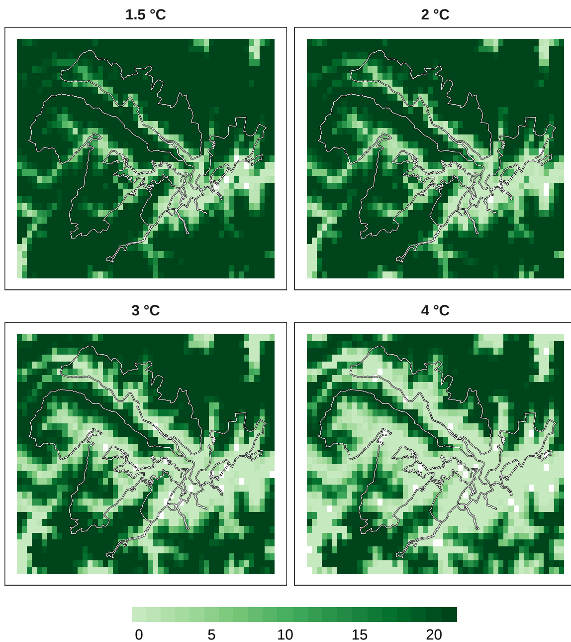
Figure 11: Number of models in agreement for bird refugia.
