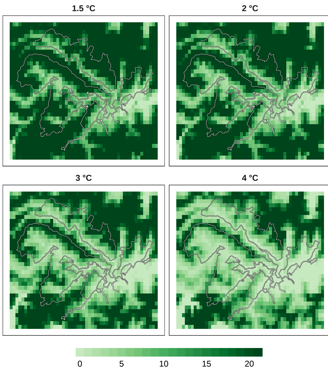
Figure 15: Number of models in agreement for pollinator refugia at 1 km resolution.
