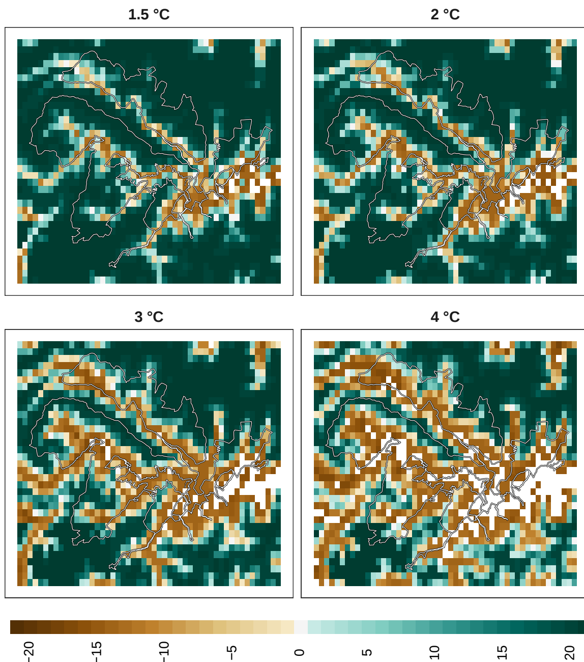
Figure 19: Adaptation effort for mammals at 1 km resolution.
