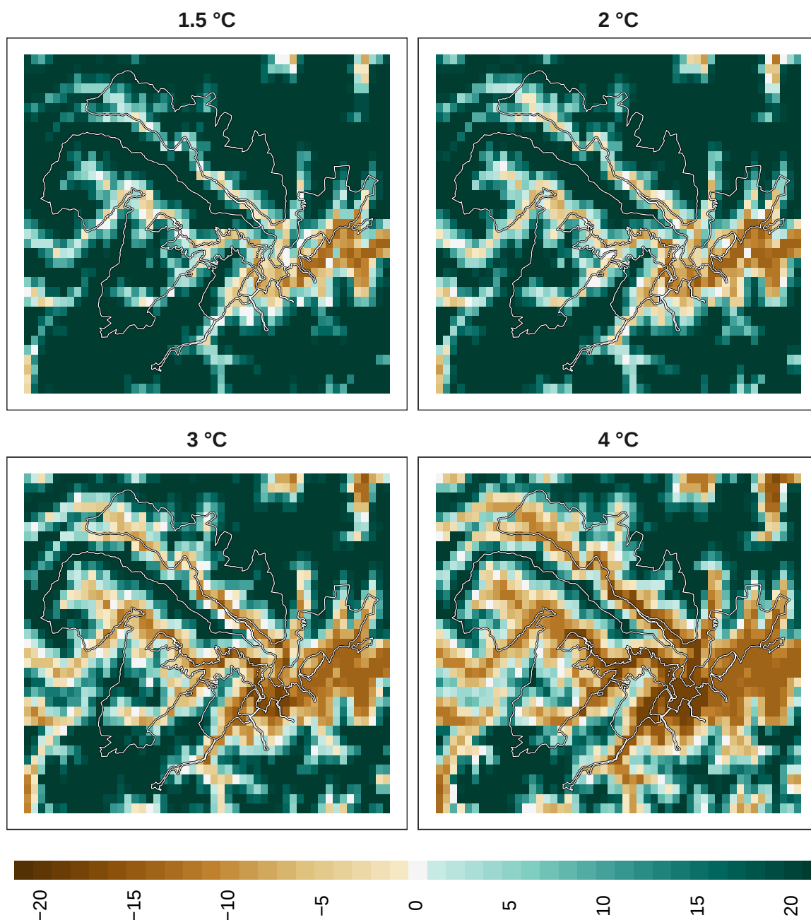
Figure 22: Adaptation effort for pollinators at 1 km resolution.
