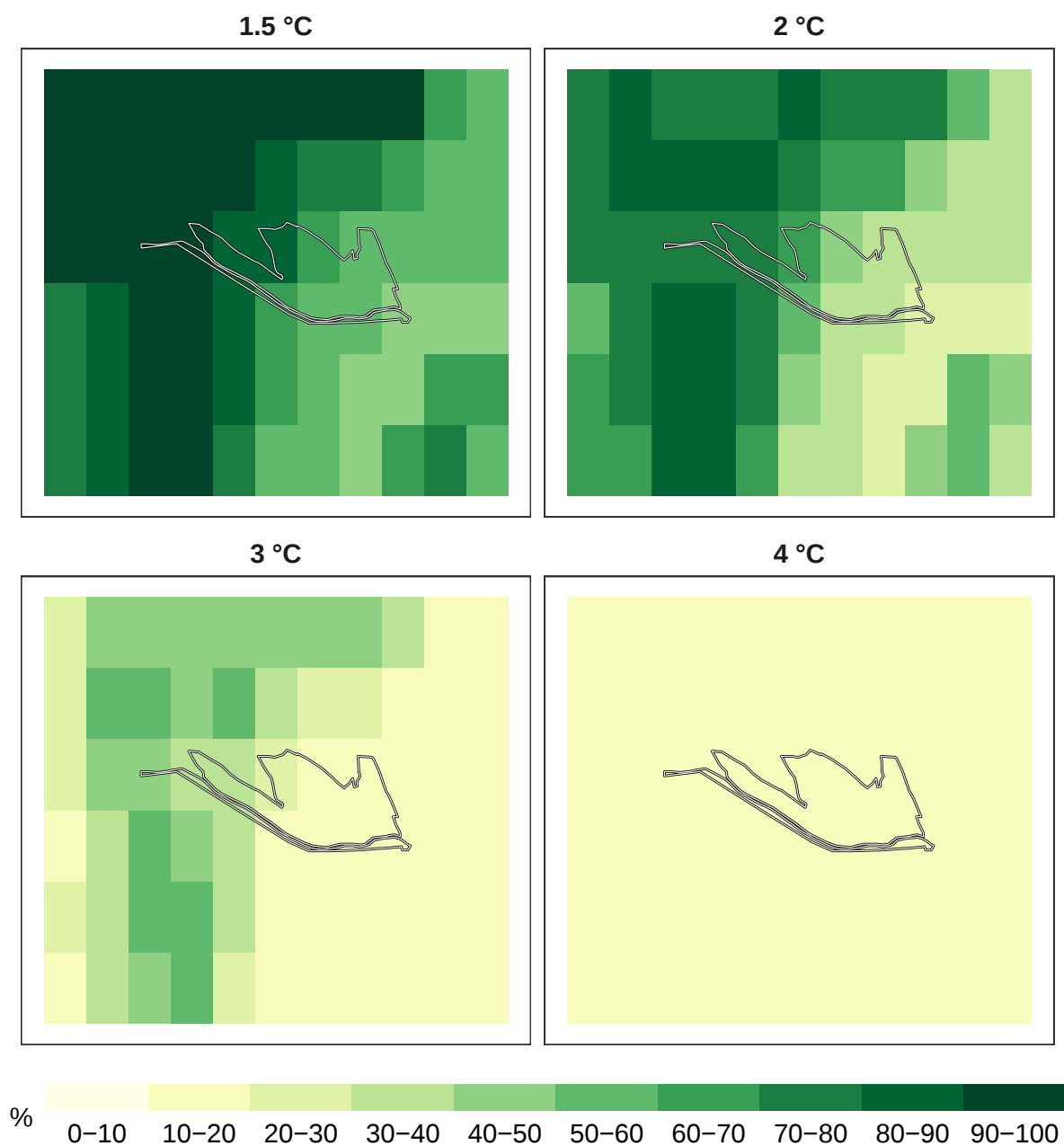
Figure 4: Percent insects remaining at 1 km resolution.
