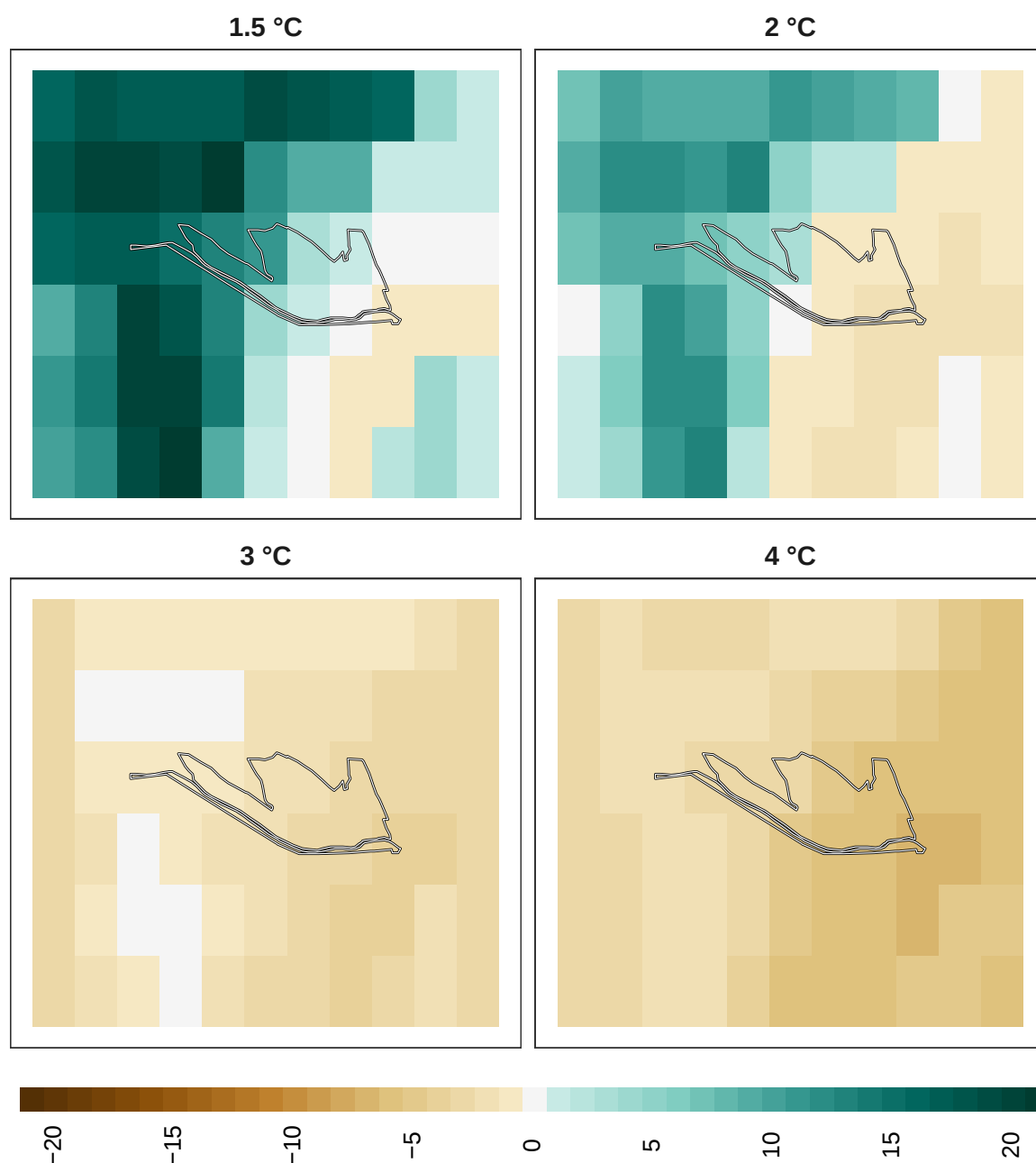
Figure 10: Adaptation effort for plants at 1 km resolution.
