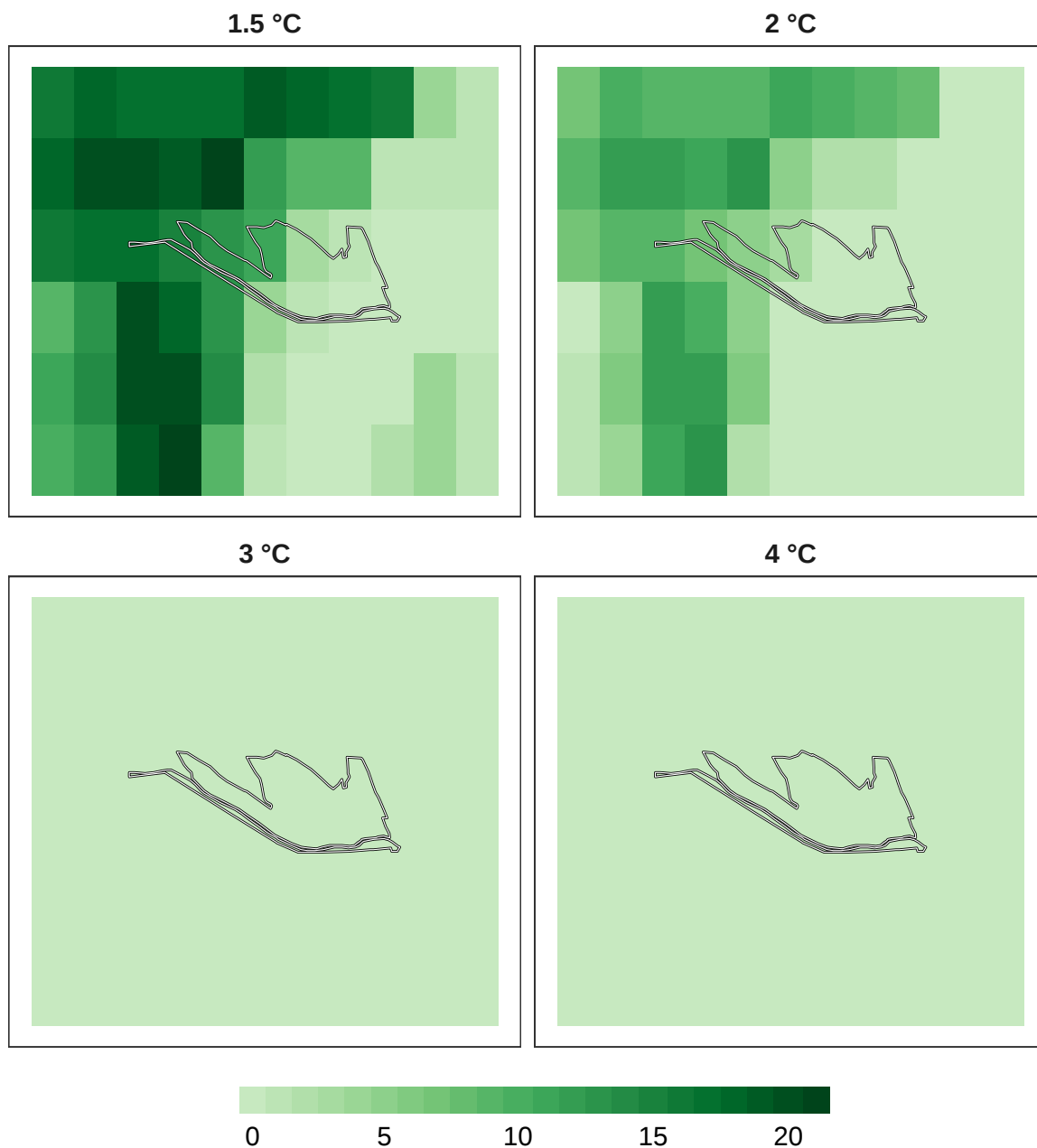
Figure 5: Number of models in agreement for overall biodiversity refugia at 1 km resolution.
