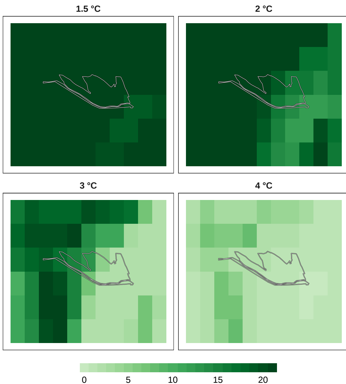
Figure 7: Number of models in agreement for bird refugia.
