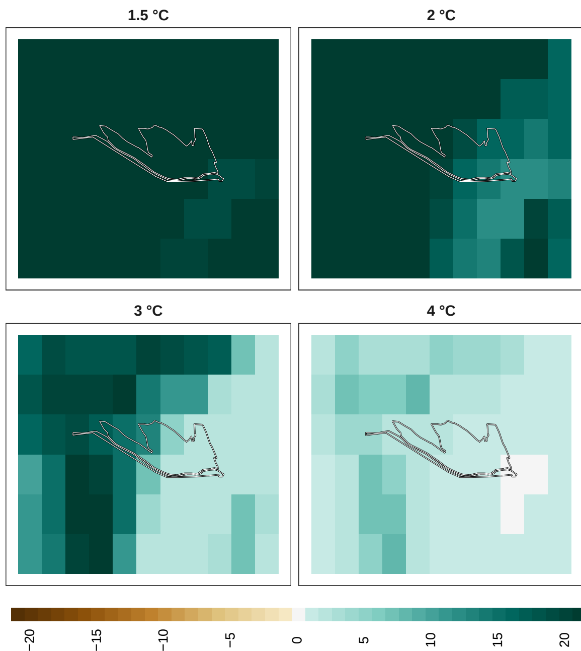
Figure 11: Adaptation effort for birds at 1 km resolution.
