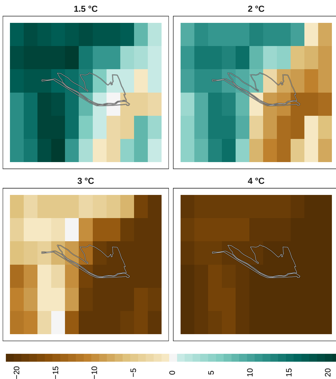
Figure 12: Adaptation effort for insects at 1 km resolution.
