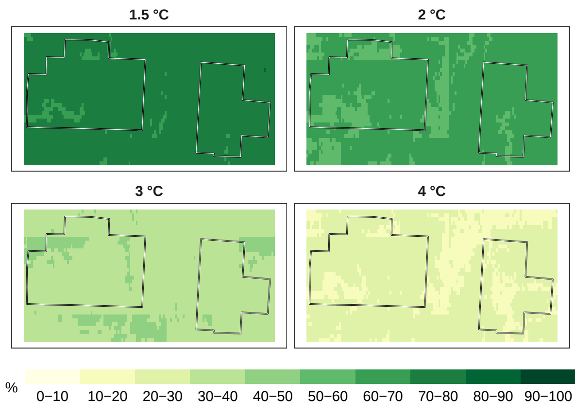
Figure 4: Percent insects remaining at 1 km resolution.
