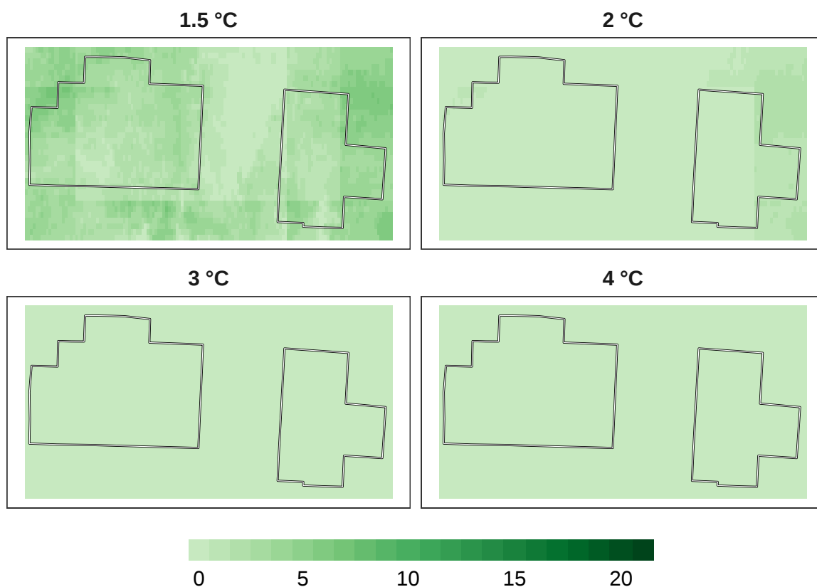
Figure 10: Number of models in agreement for pollinator refugia at 1 km resolution.
