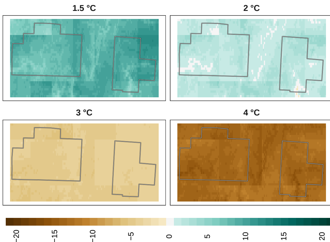
Figure 14: Adaptation effort for insects at 1 km resolution.
