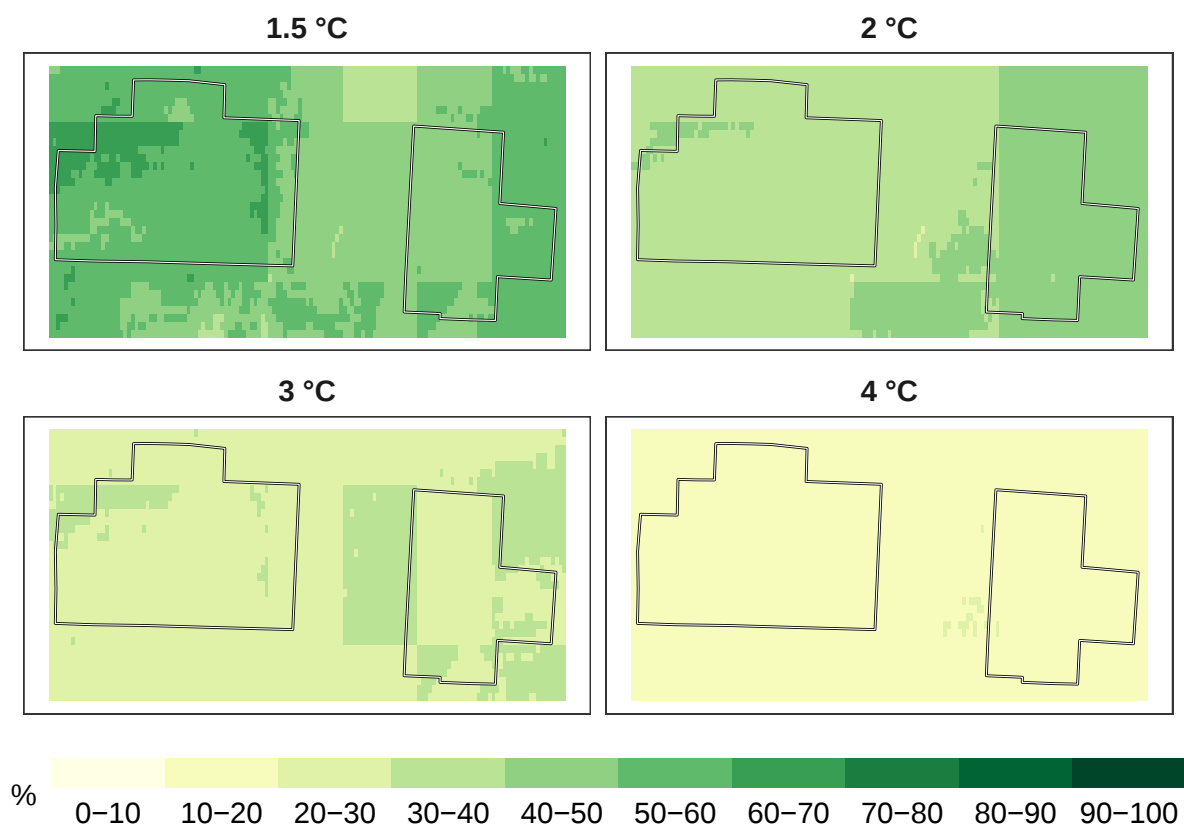
Figure 5: Percent pollinators remaining at 1 km resolution.
