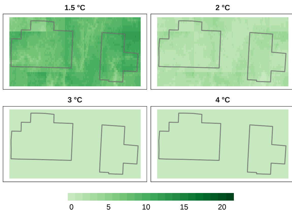
Figure 9: Number of models in agreement for insect refugia at 1 km resolution.
