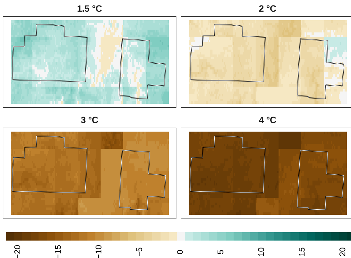
Figure 15: Adaptation effort for pollinators at 1 km resolution.
