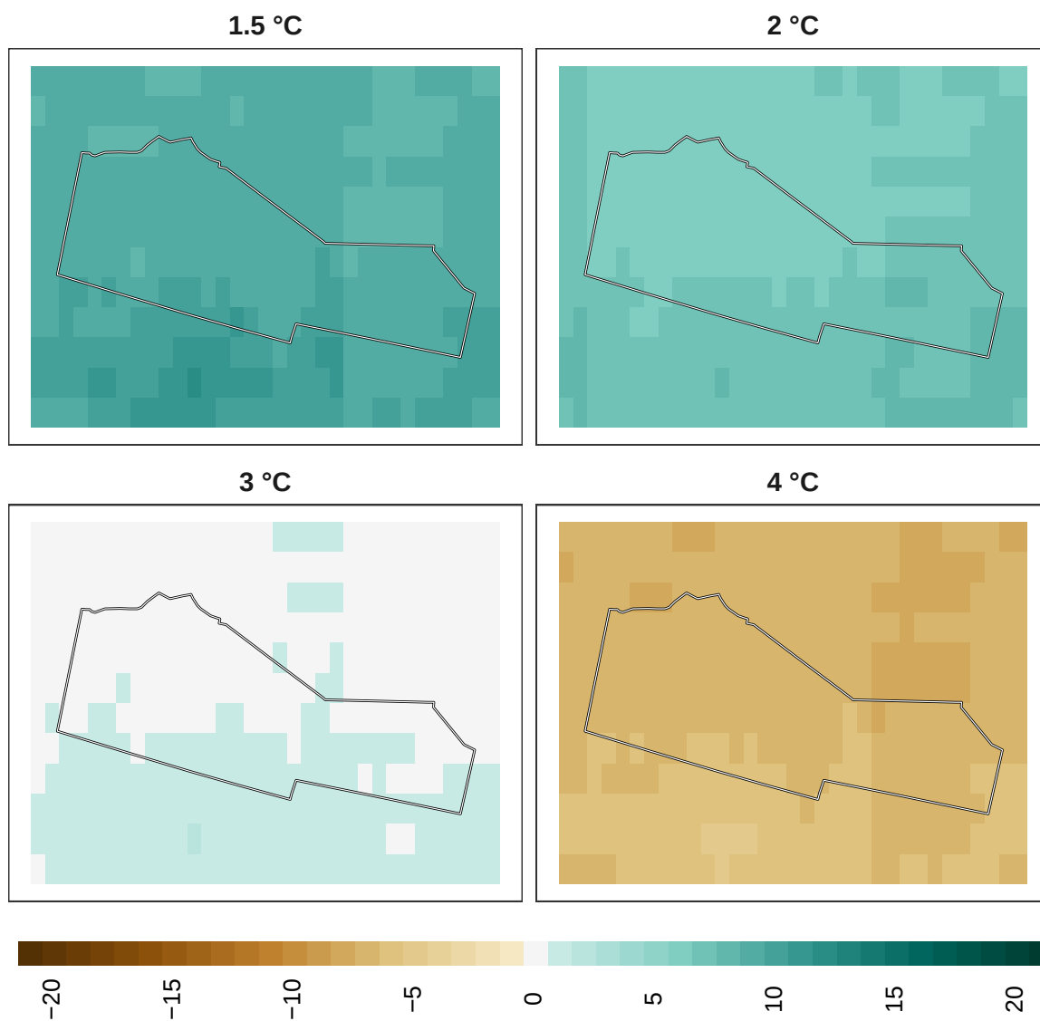
Figure 15: Adaptation effort for pollinators at 1 km resolution.
