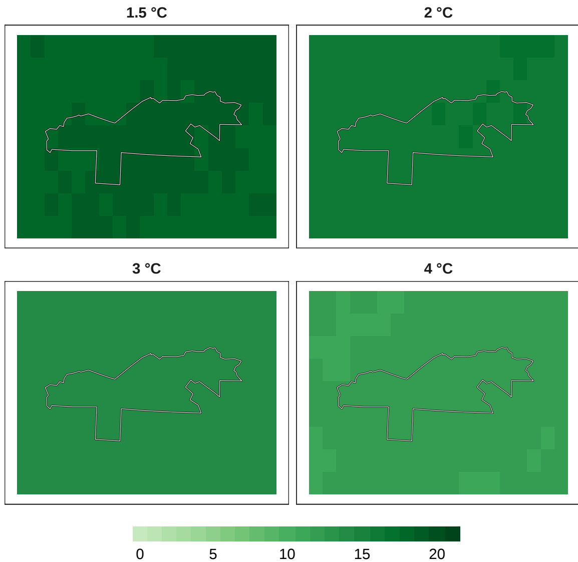
Figure 13: Number of models in agreement for reptile refugia at 1 km resolution.
