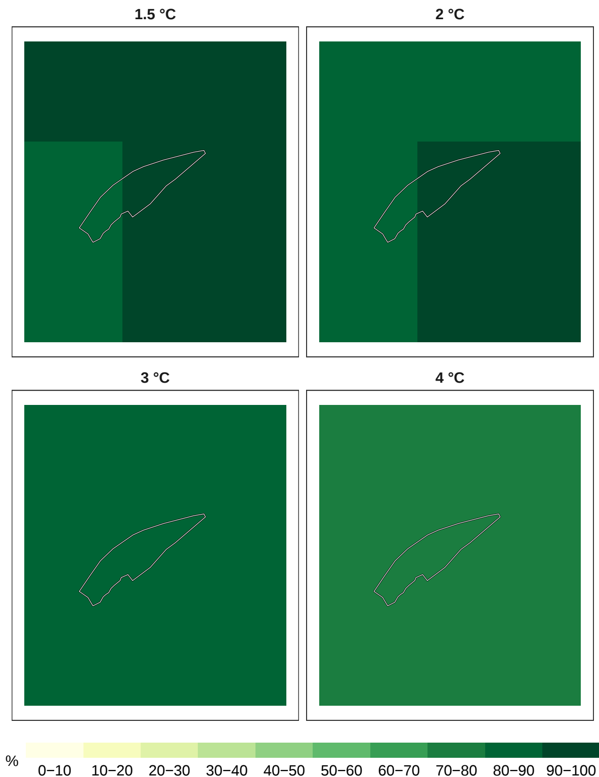
Figure 5: Percent reptiles remaining at 1 km resolution.
