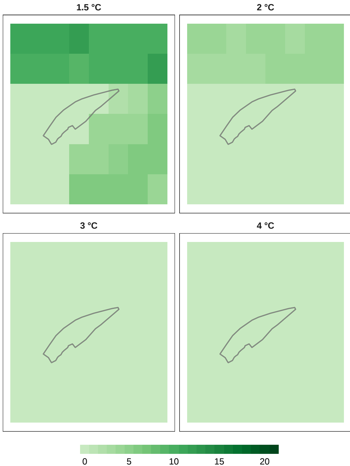
Figure 7: Number of models in agreement for overall biodiversity refugia at 1 km resolution.
