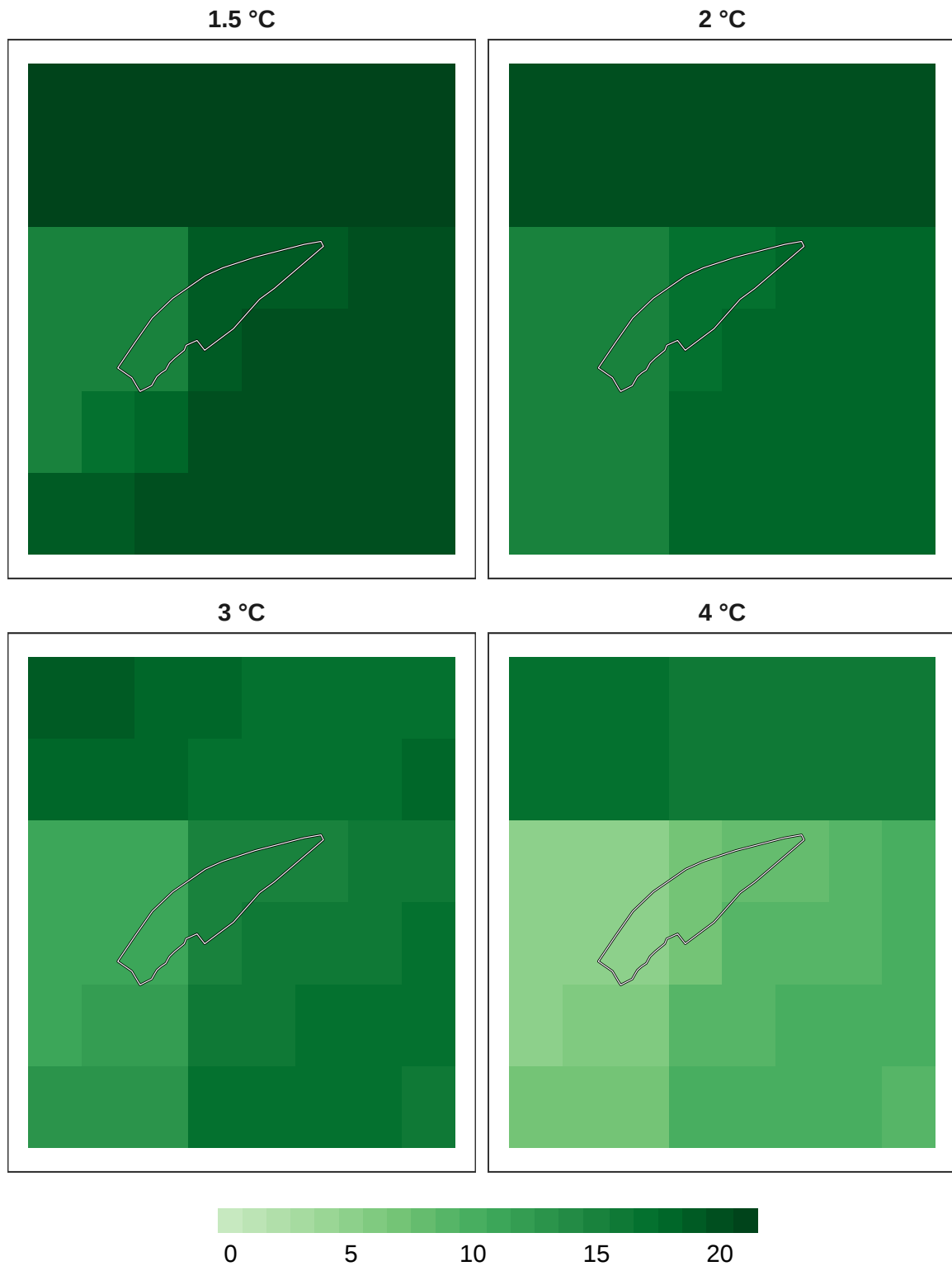
Figure 11: Number of models in agreement for reptile refugia at 1 km resolution.
