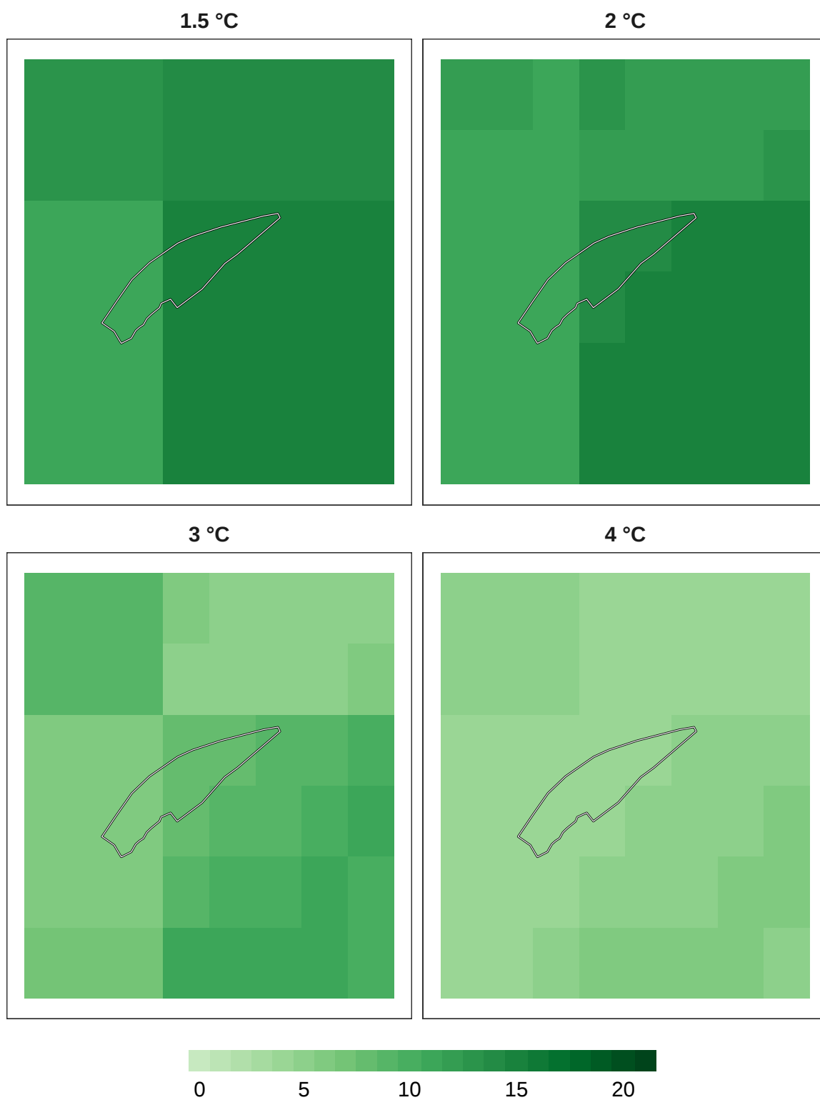
Figure 9: Number of models in agreement for bird refugia.
