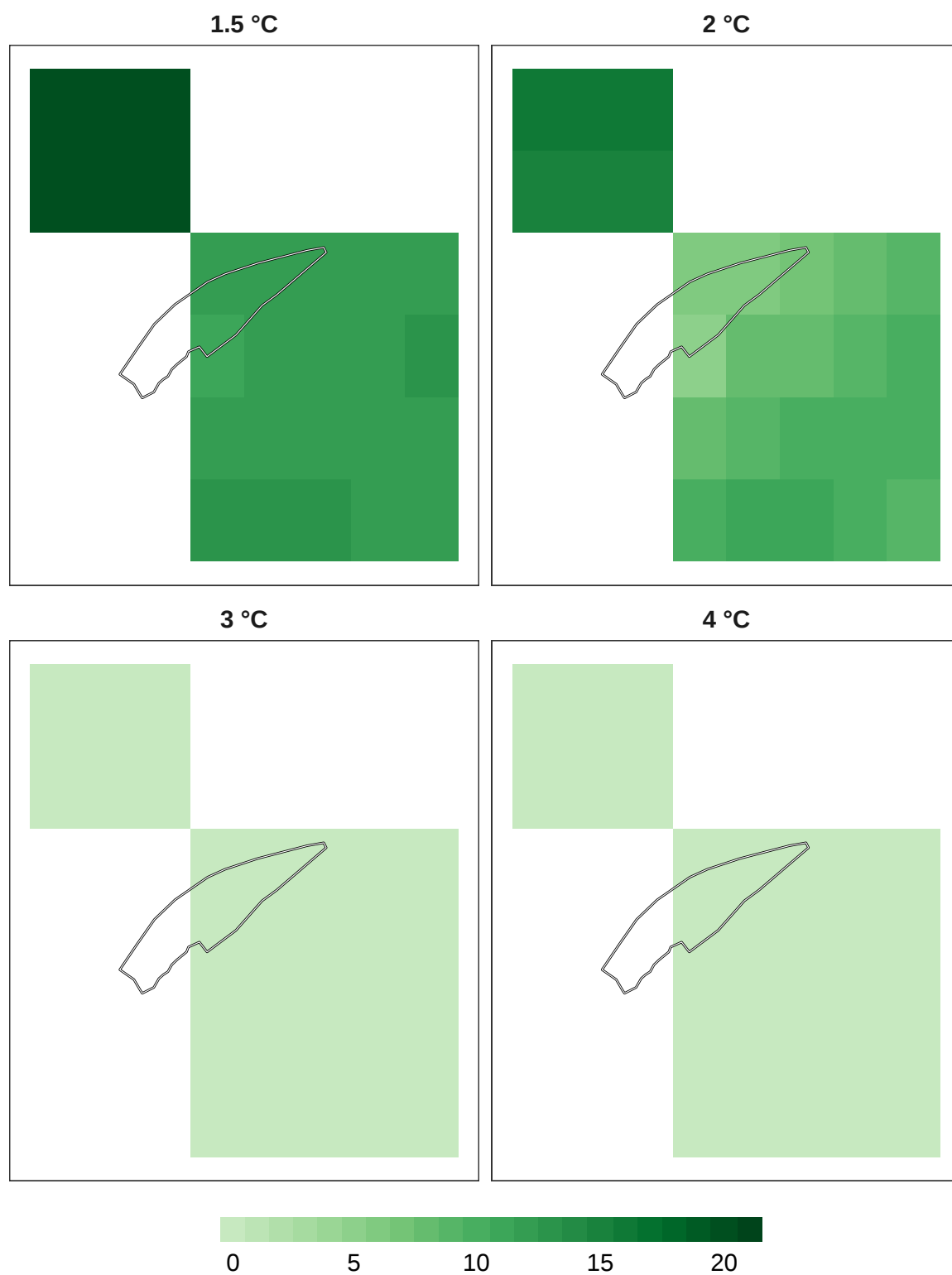
Figure 10: Number of models in agreement for mammal refugia at 1 km resolution.
