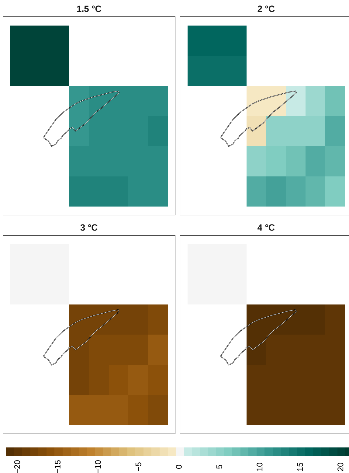
Figure 16: Adaptation effort for mammals at 1 km resolution.
