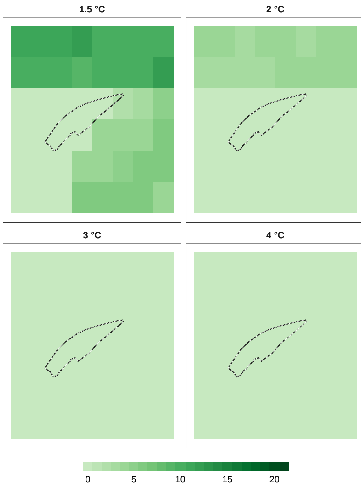
Figure 8: Number of models in agreement for plant refugia at 1 km resolution.
