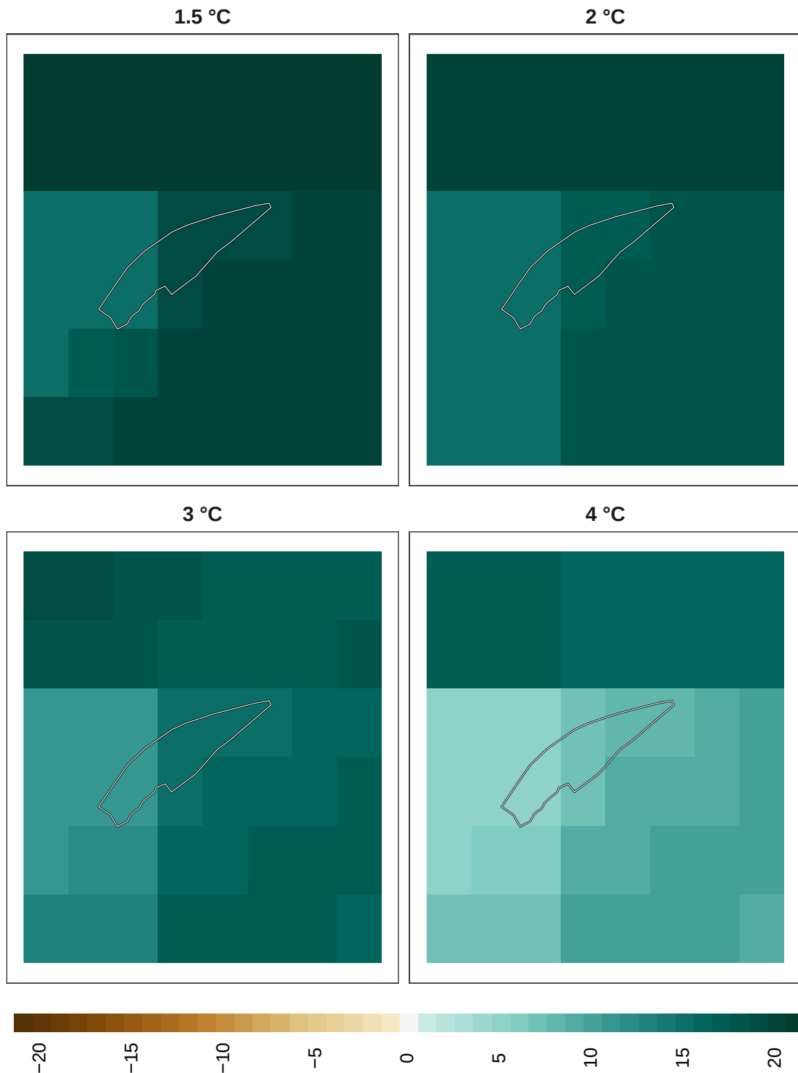
Figure 17: Adaptation effort for reptiles at 1 km resolution.
