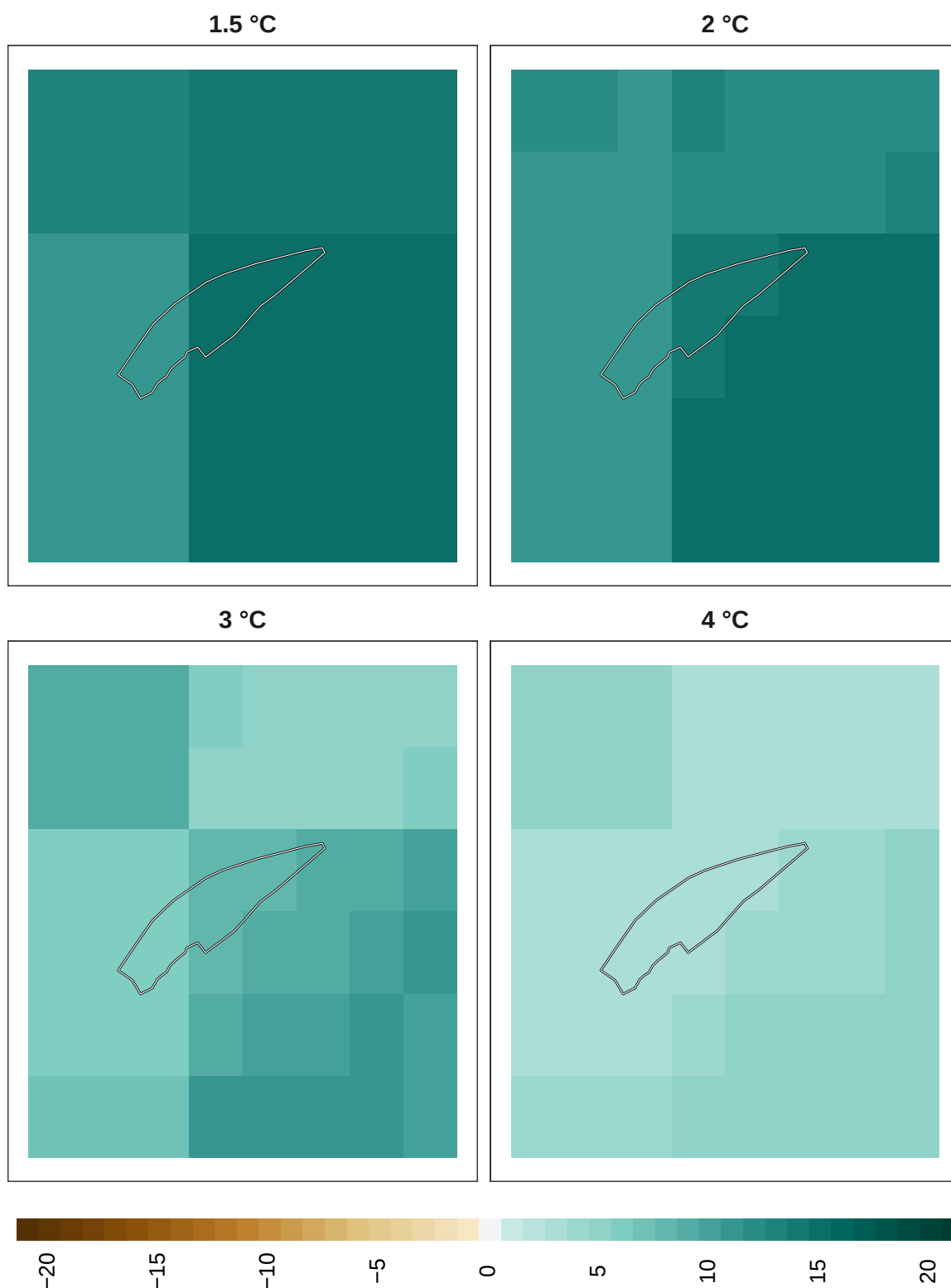
Figure 15: Adaptation effort for birds at 1 km resolution.
