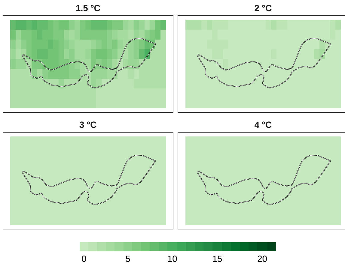
Figure 11: Number of models in agreement for insect refugia at 1 km resolution.
