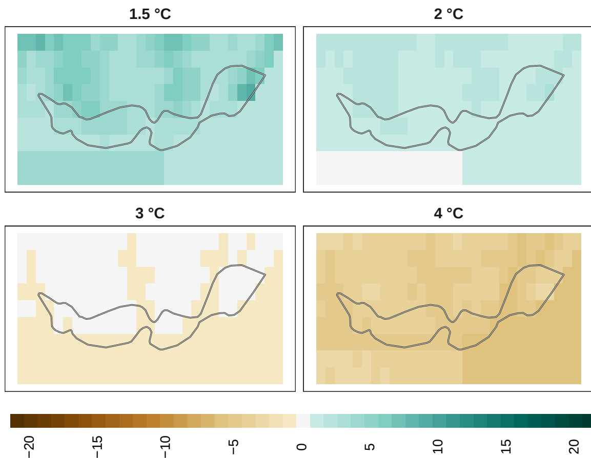
Figure 12: Adaptation effort for overall biodiversity at 1 km resolution.
