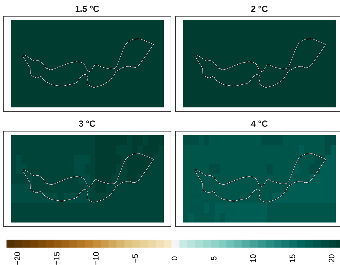
Figure 14: Adaptation effort for birds at 1 km resolution.
