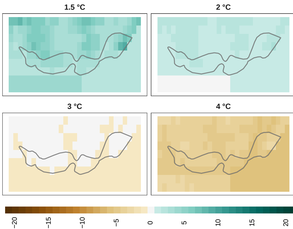
Figure 13: Adaptation effort for plants at 1 km resolution.
