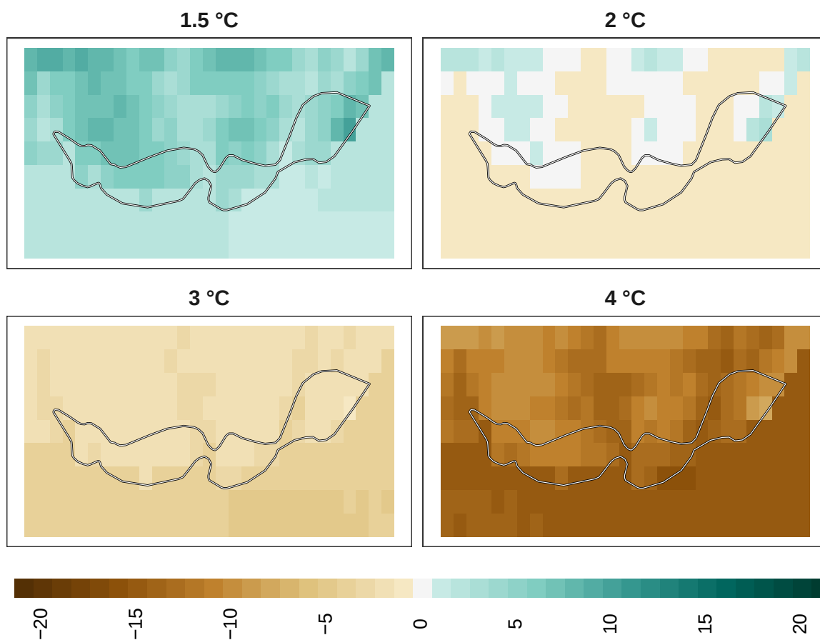
Figure 16: Adaptation effort for insects at 1 km resolution.
