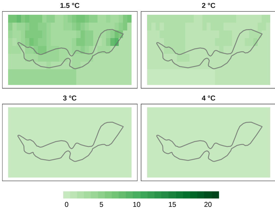
Figure 7: Number of models in agreement for overall biodiversity refugia at 1 km resolution.
