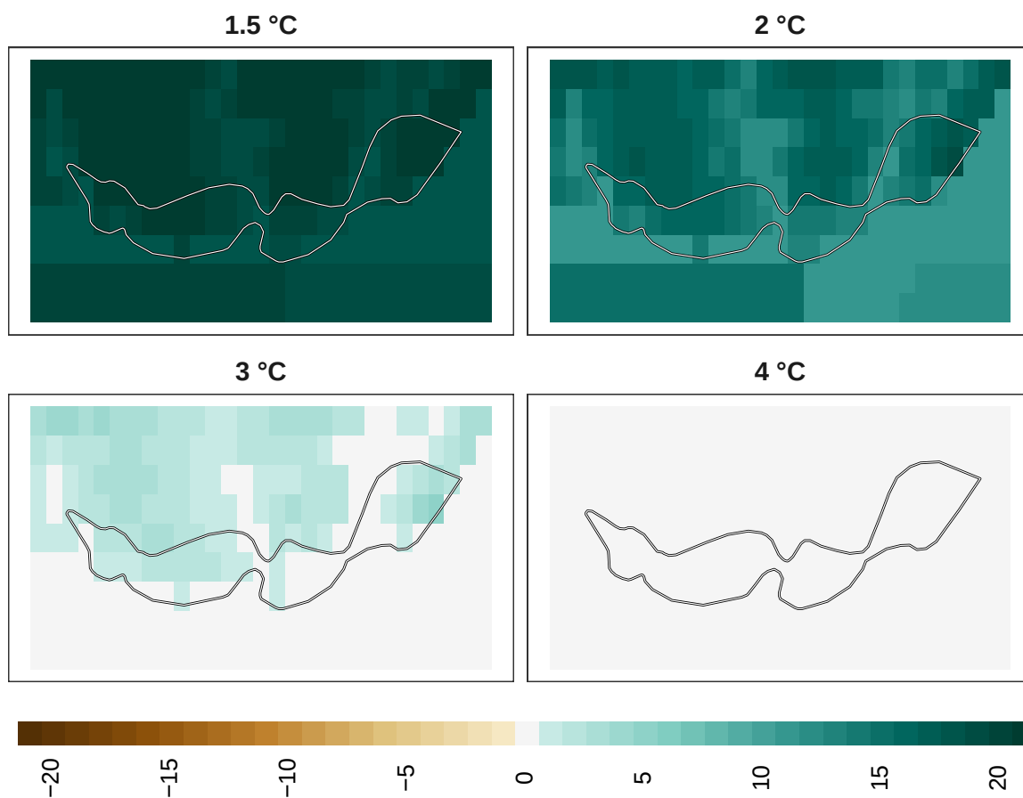
Figure 15: Adaptation effort for mammals at 1 km resolution.
