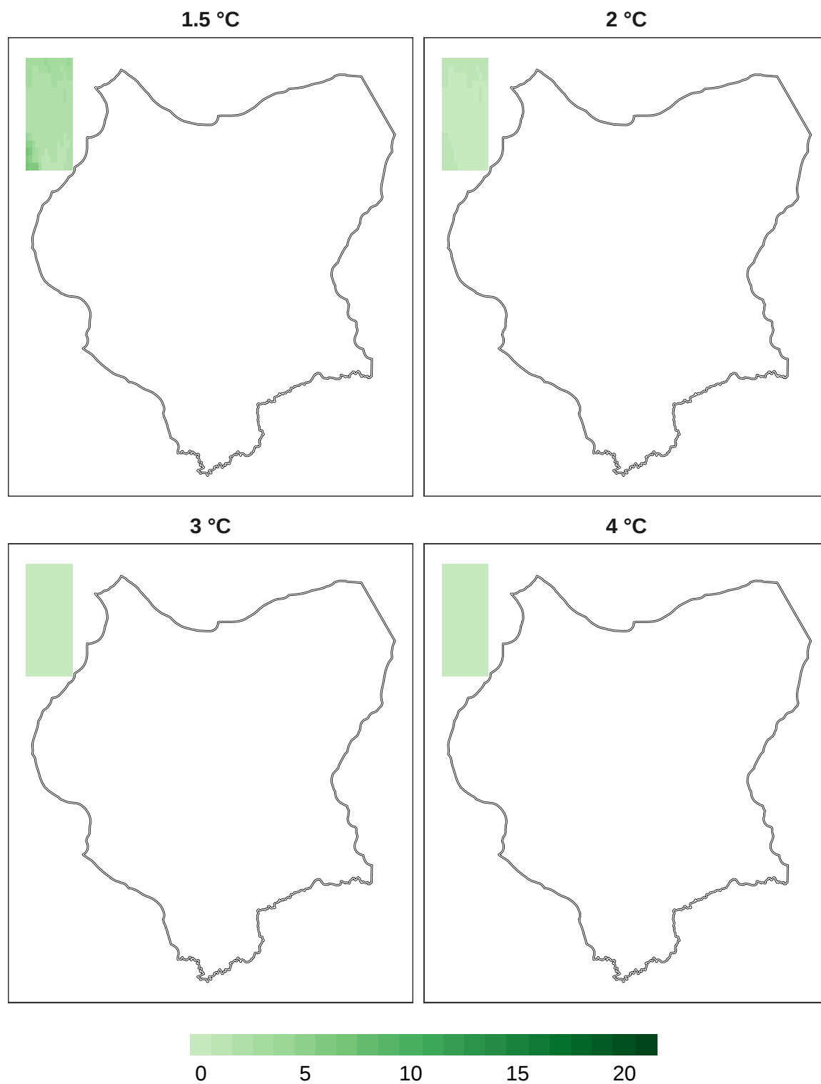
Figure 10: Number of models in agreement for pollinator refugia at 1 km resolution.
