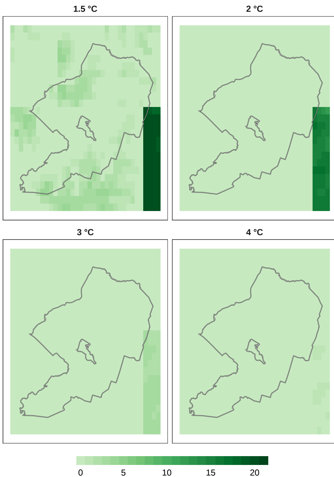
Figure 9: Number of models in agreement for mammal refugia at 1 km resolution.
