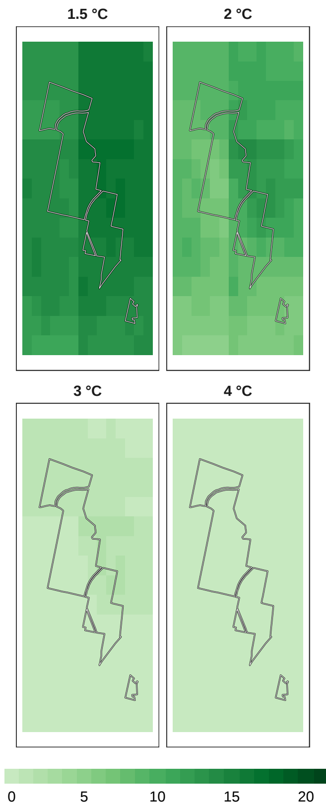
Figure 10: Number of models in agreement for pollinator refugia at 1 km resolution.
