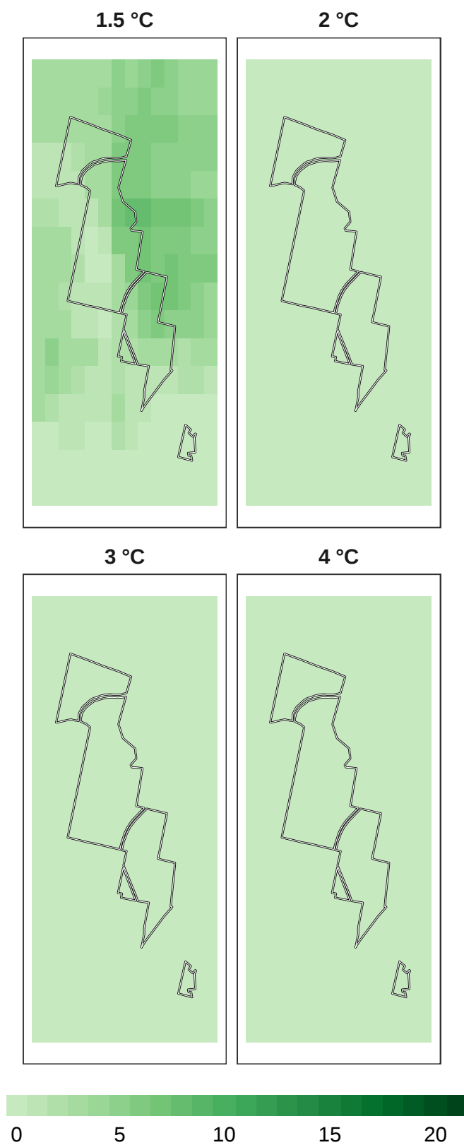
Figure 9: Number of models in agreement for insect refugia at 1 km resolution.
