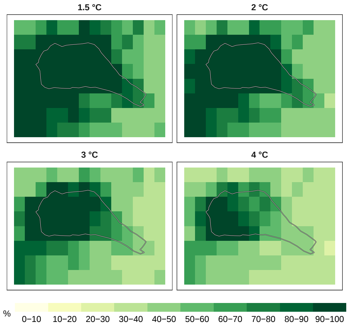
Figure 5: Percent mammals remaining at 1 km resolution.
