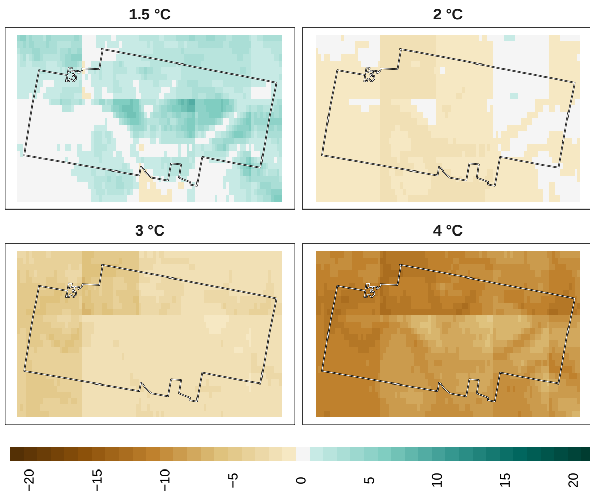
Figure 14: Adaptation effort for overall biodiversity at 1 km resolution.
