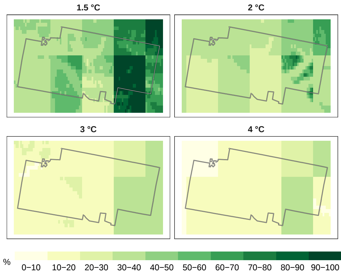
Figure 7: Percent timber species remaining at 1 km resolution.
