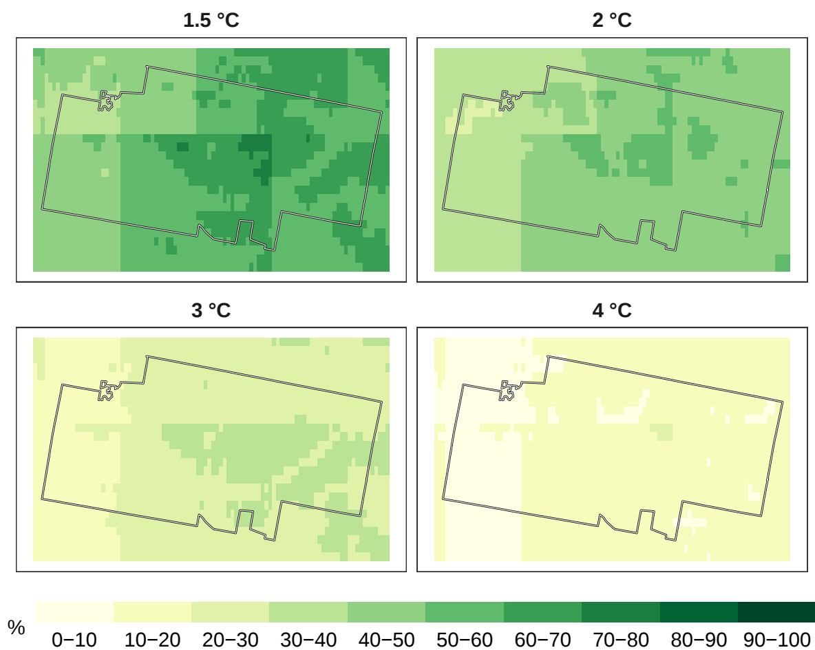
Figure 6: Percent pollinators remaining at 1 km resolution.
