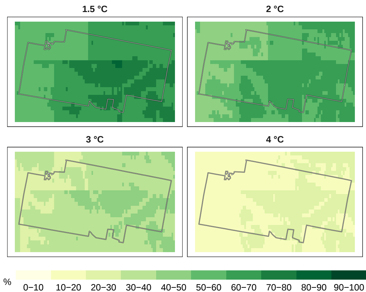
Figure 5: Percent insects remaining at 1 km resolution.
