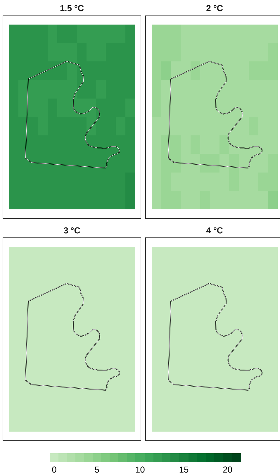
Figure 12: Number of models in agreement for pollinator refugia at 1 km resolution.
