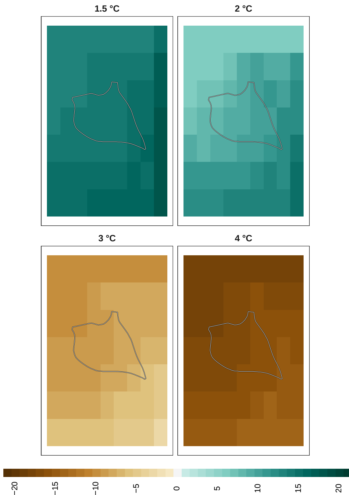
Figure 16: Adaptation effort for pollinators at 1 km resolution.
