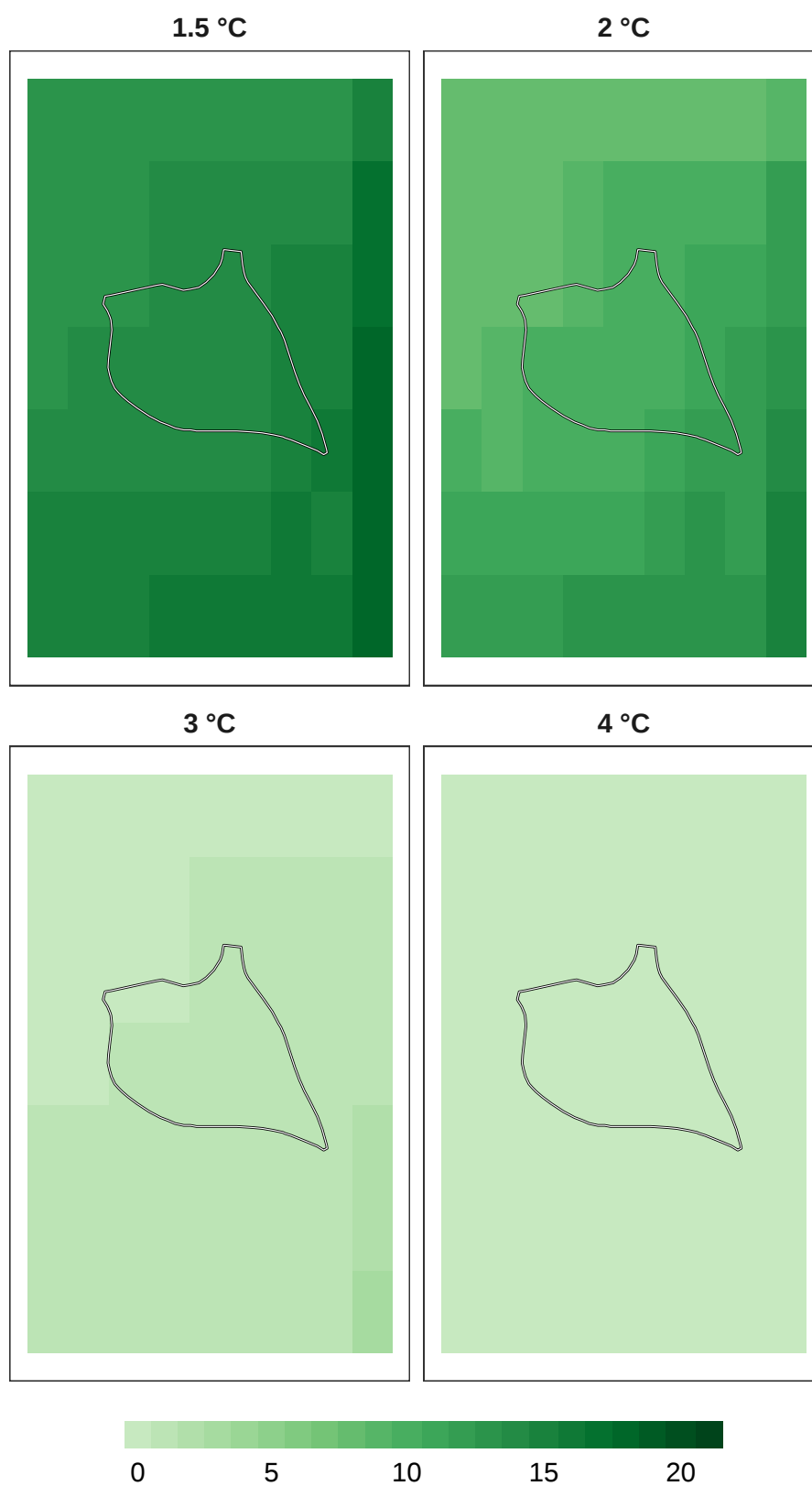
Figure 11: Number of models in agreement for pollinator refugia at 1 km resolution.
