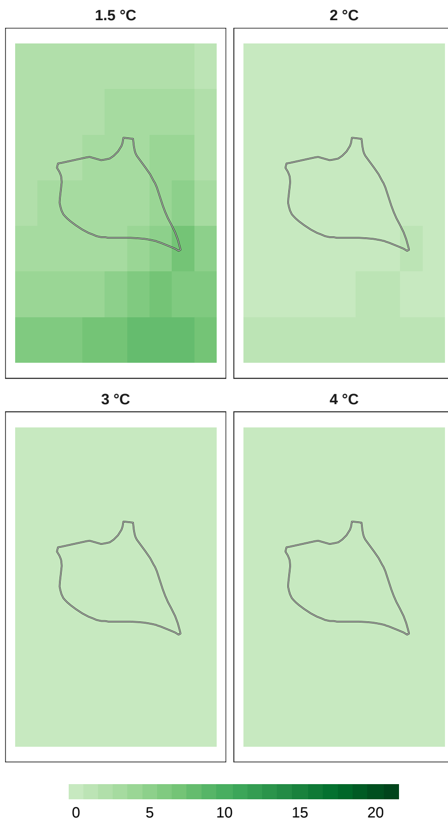
Figure 10: Number of models in agreement for insect refugia at 1 km resolution.
